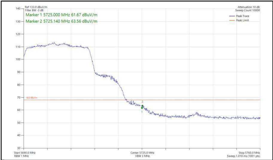
Figure 309 - 802.11ax, HE20, SU, SISO, Core 1 - 5700 MHz, Band Edge Frequency 5725 MHz
