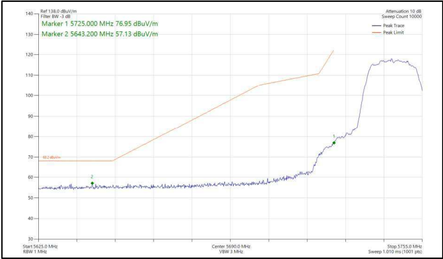
Figure 302 - 802.11a, SISO, Core 1 - 5745 MHz, Band Edge Frequency 5725 MHz
