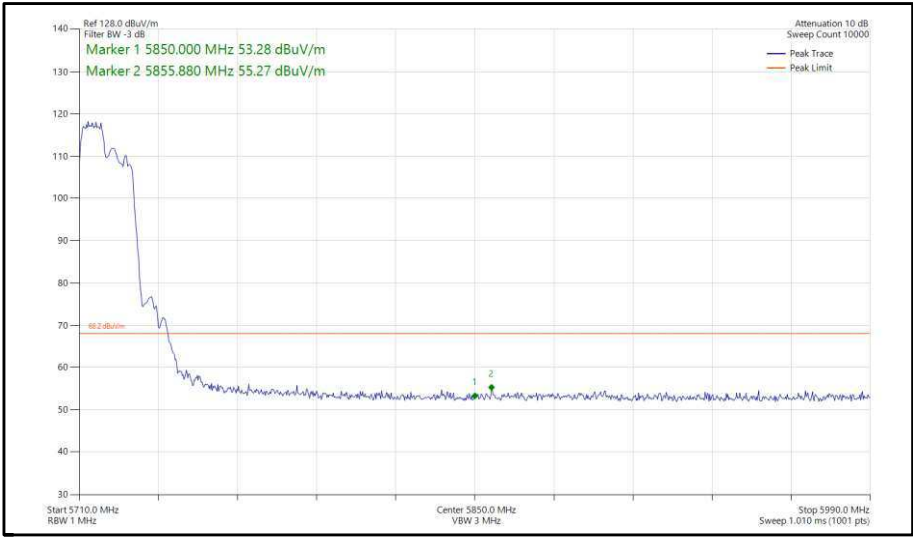
Figure 295 - 802.11ax, HE20, RU 106-53, SISO, Core 0 - 5720 MHz, Band Edge Frequency 5850 MHz
