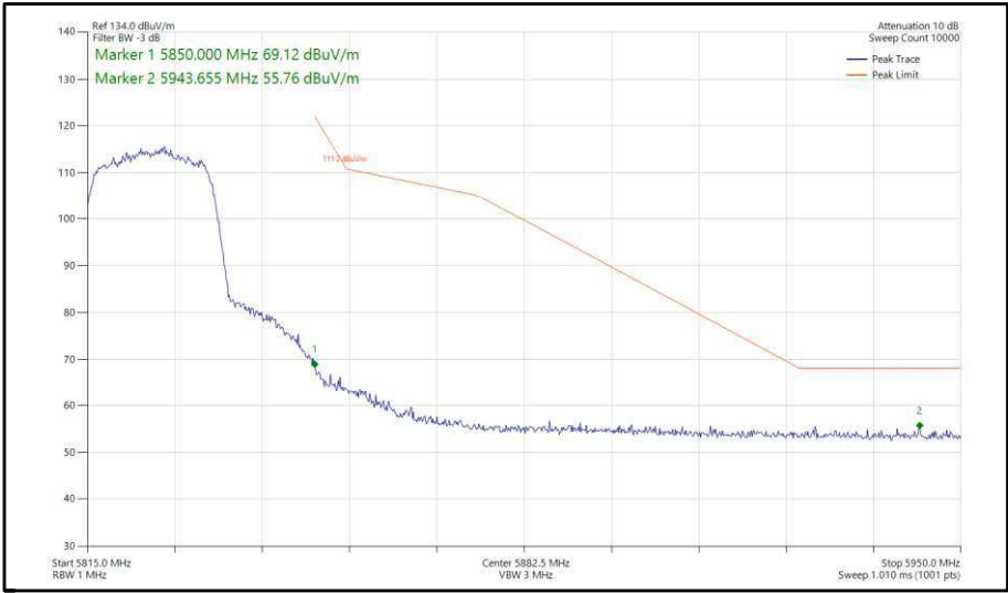
Figure 293 - 802.11n, HT20, SISO, Core 0 - 5825 MHz, Band Edge Frequency 5850 MHz
