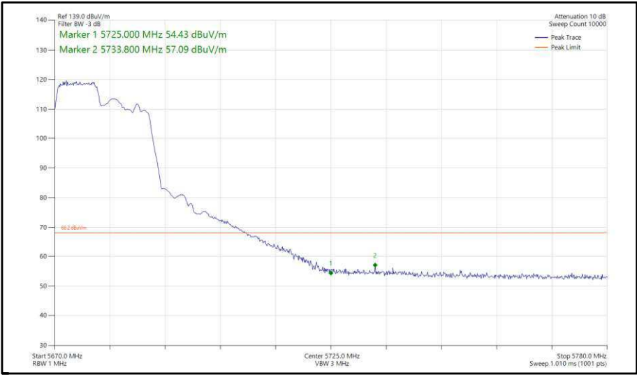
Figure 287 - 802.11ax, HE20, RU 106-53, SISO, Core 0 - 5680 MHz, Band Edge Frequency 5725 MHz
