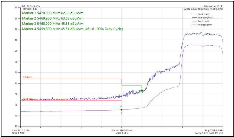
Figure 300 - 802.11ax, HE20, SU, SISO, Core 1 - 5500 MHz, Band Edge Frequency 5470 MHz
