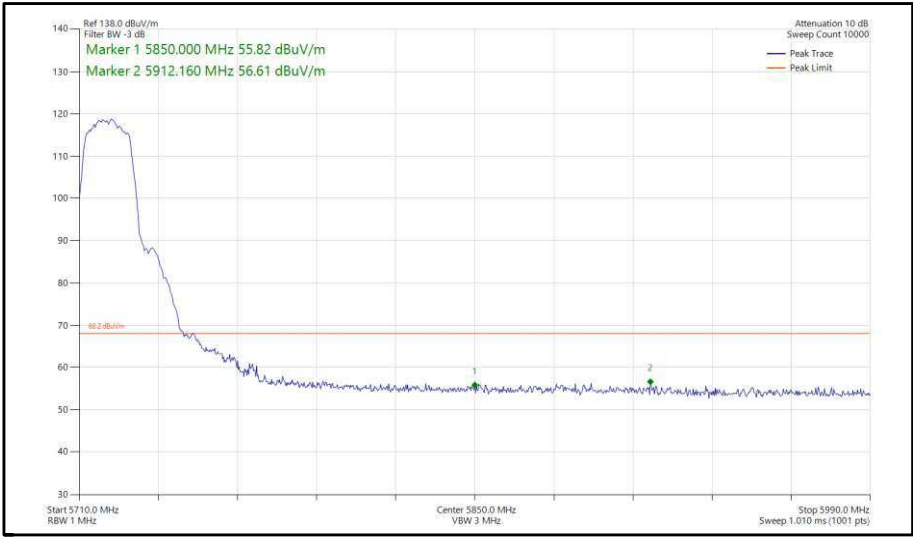
Figure 311 - 802.11a, SISO, Core 1 - 5720 MHz, Band Edge Frequency 5850 MHz
