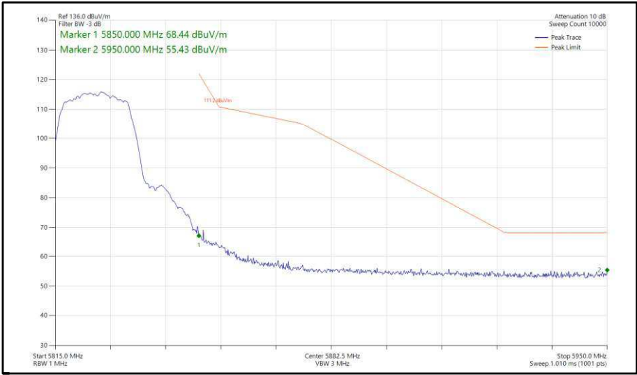
Figure 291 - 802.11a, SISO, Core 0 - 5825 MHz, Band Edge Frequency 5850 MHz
