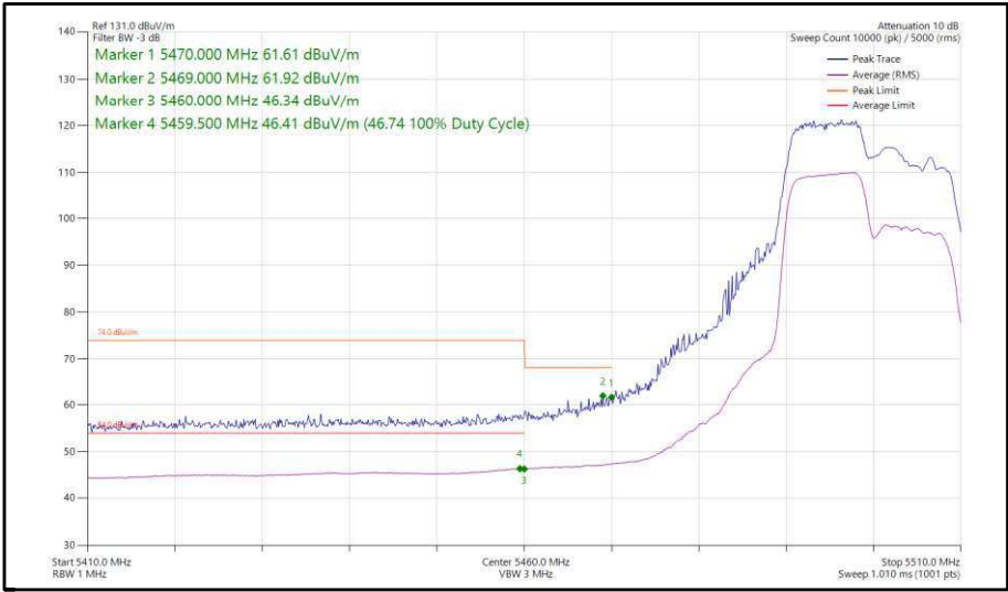
Figure 301 - 802.11ax, HE20, RU 106-53, SISO, Core 1 - 5500 MHz, Band Edge Frequency 5470 MHz
