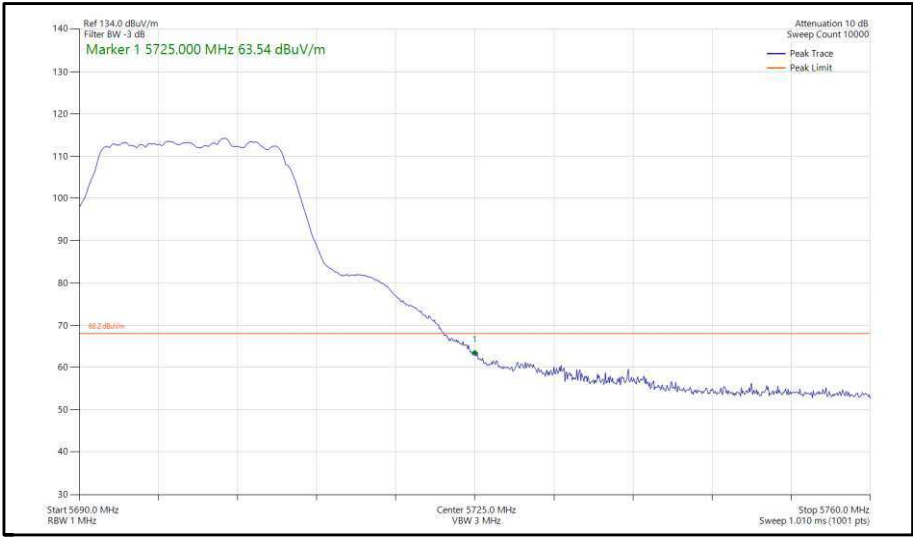
Figure 285 - 802.11a, SISO, Core 0 - 5700 MHz, Band Edge Frequency 5725 MHz
