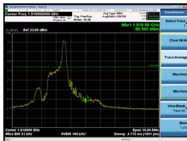
LTE eMTC Band 2 20MHz QPSK 100%RB CH-High
