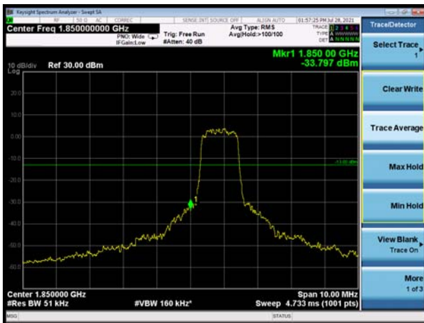
LTE eMTC Band 25 5MHz QPSK 1RB CH-Low
