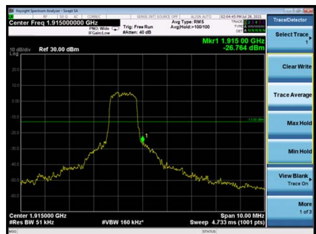
LTE eMTC Band 25 5MHz QPSK 100%RB CH-High
