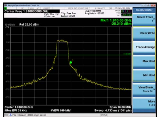
LTE eMTC Band 2 5MHz 16QAM 100%RB CH-High
