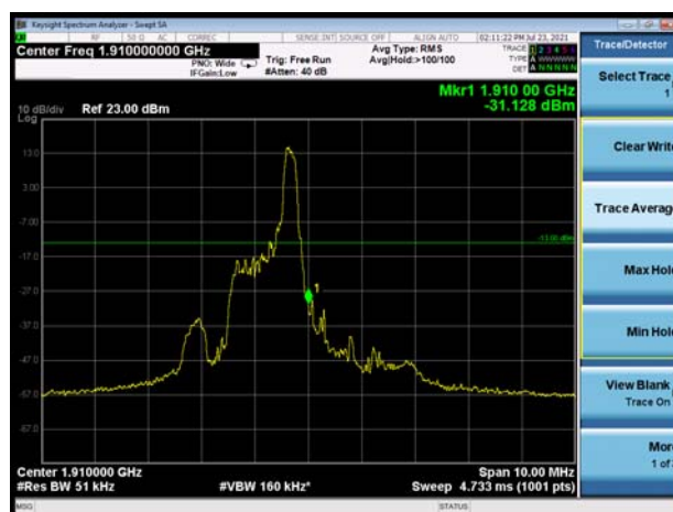
LTE eMTC Band 2 5MHz QPSK 100%RB CH-High
