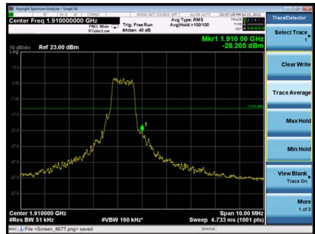
LTE eMTC Band 2 5MHz 16QAM 1RB CH-High
