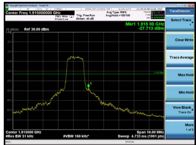
LTE eMTC Band 25 5MHz QPSK 1RB CH-High
