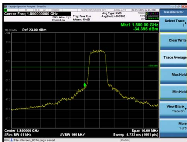
LTE eMTC Band 2 5MHz QPSK 1RB CH-Low
