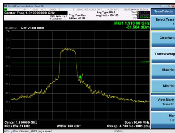
LTE eMTC Band 2 5MHz QPSK 1RB CH-High
