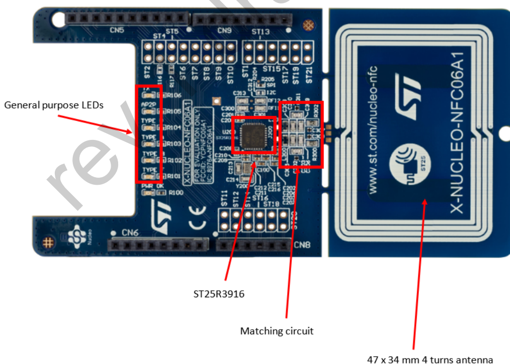
Figure 2. X-NUCLEO-NFC06A1 component placement
