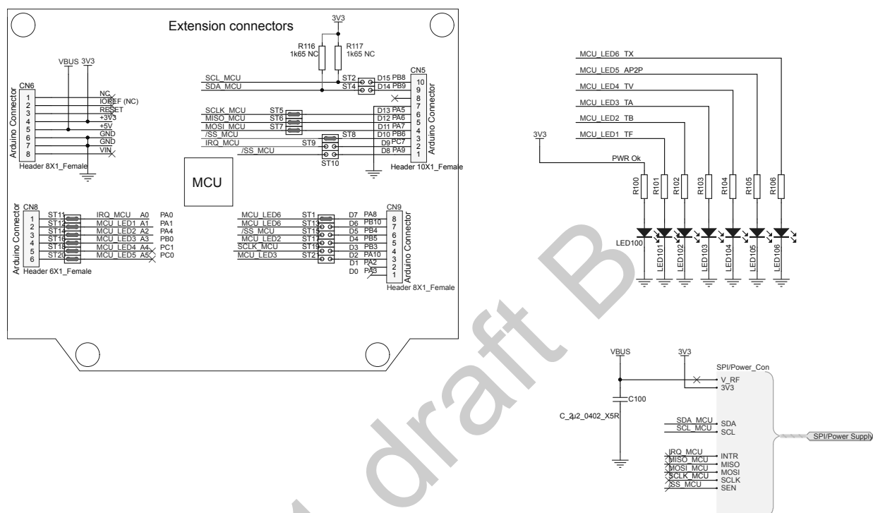
Figure 3. X-NUCLEO-NFC06A1 circuit schematic (1 of 3)
