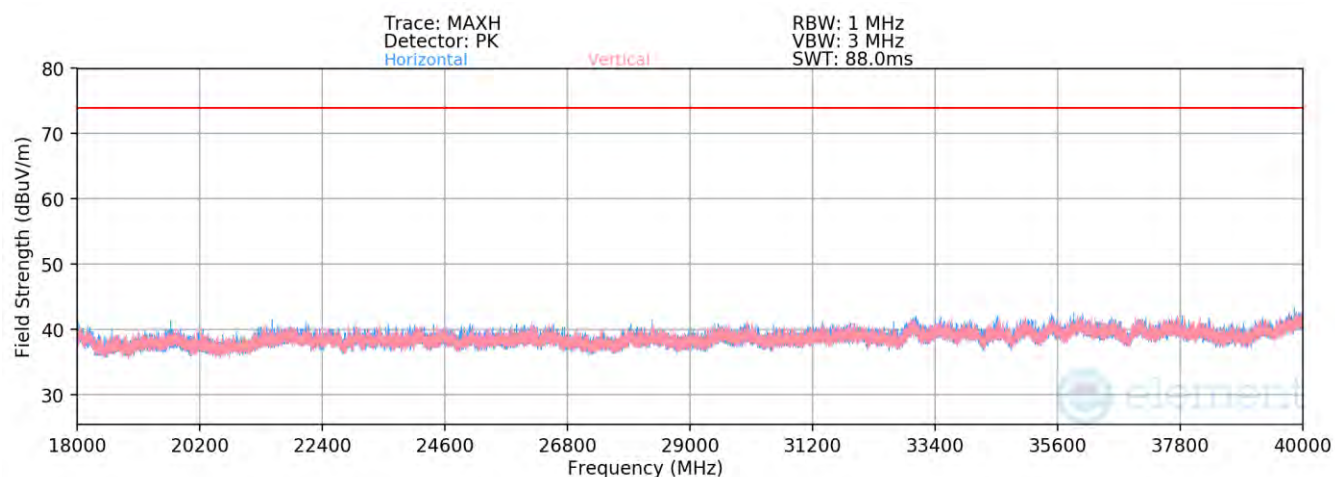
Plot 7-89. Radiated Spurious Emissions Above 18GHz TxBF (4Mbps, HDR4, ePA – Ch. 38)
