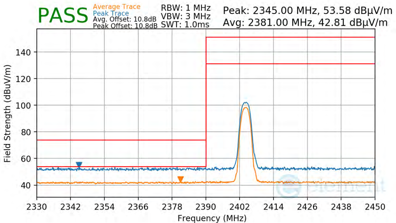
Plot 7-95. Radiated Restricted Lower Band Edge Measurement Antenna 2a
