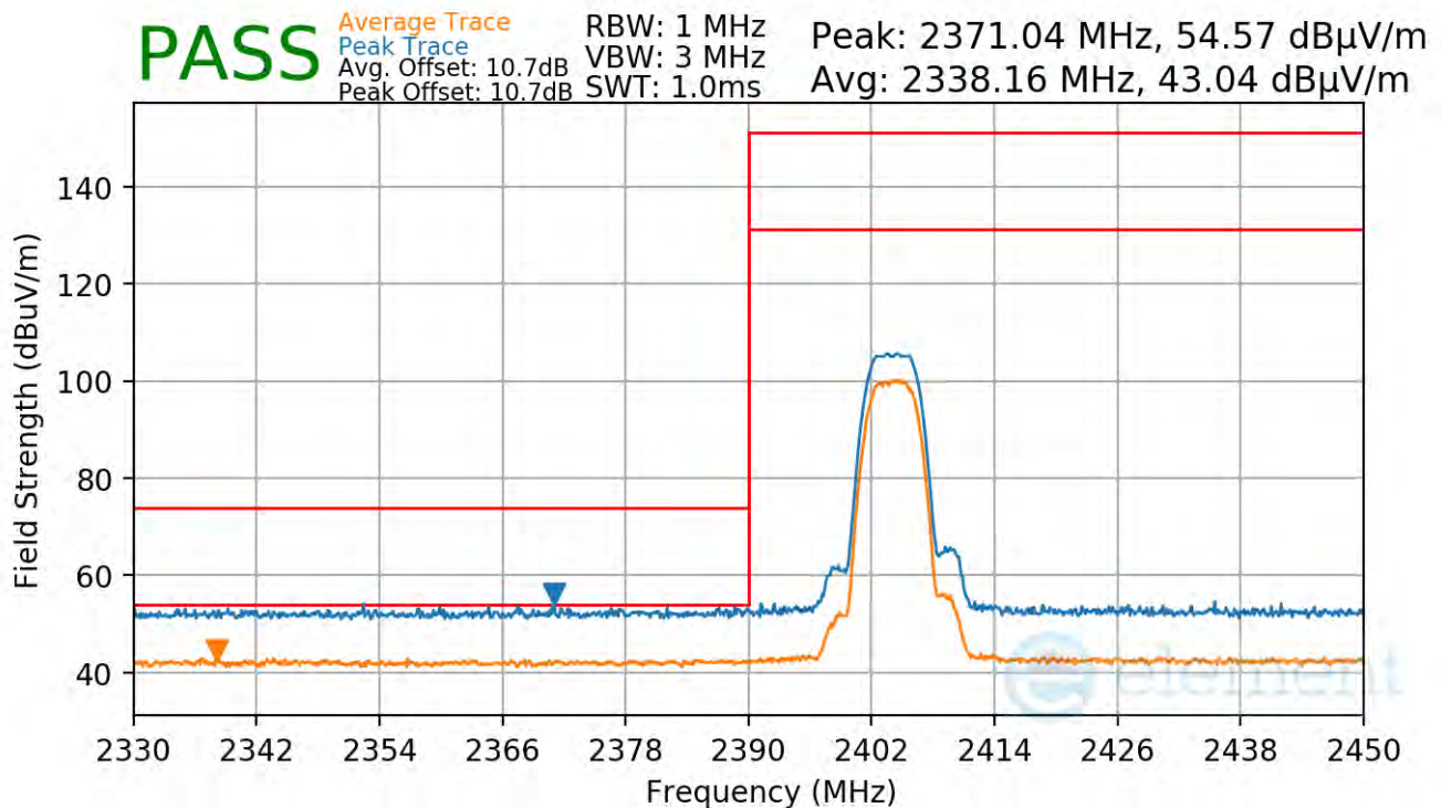
Plot 7-100. Radiated Restricted Lower Band Edge Measurement TxBF
