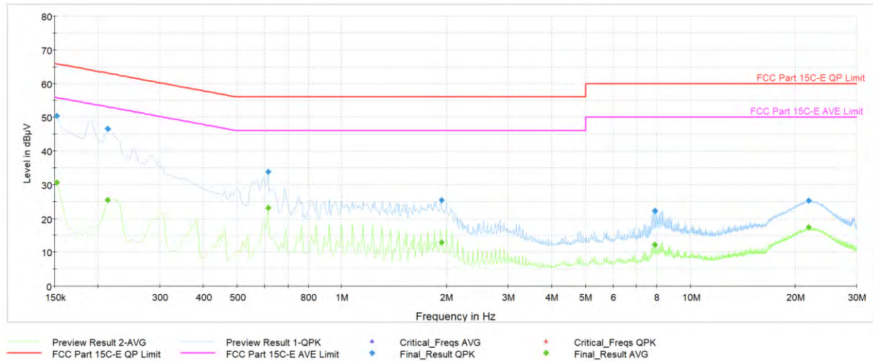
Plot 7-104. AC Line Conducted Plot with Bluetooth HDR TxBF (L1, 4Mbps ePA - Ch.38 with Laptop)
