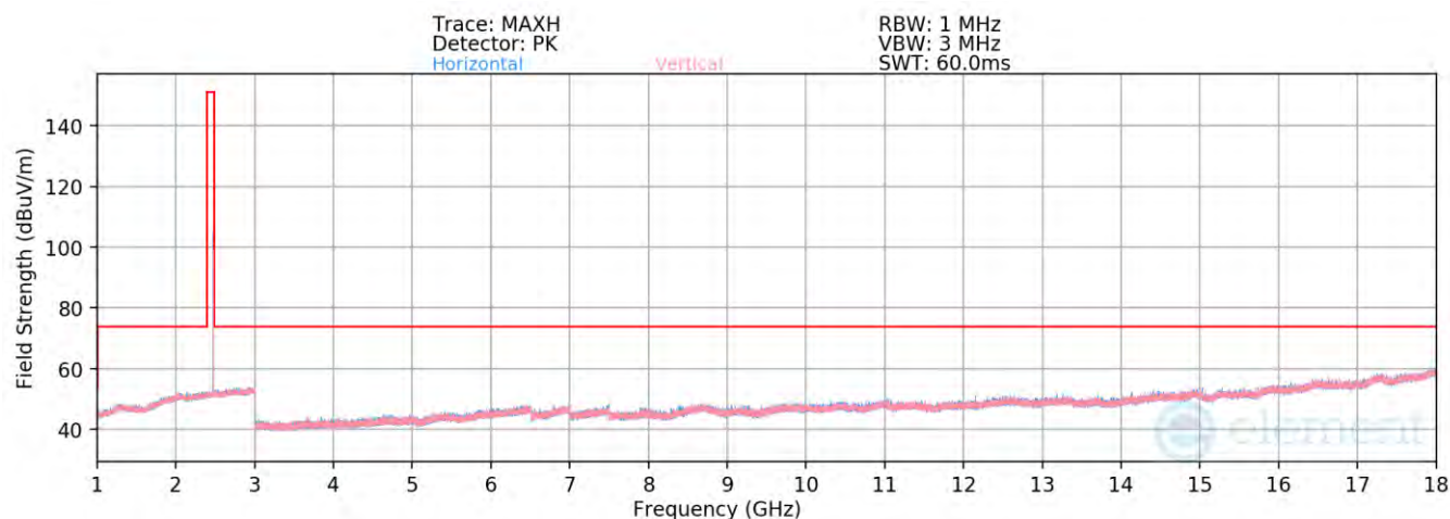
Plot 7-90. Radiated Spurious Emissions 1-18GHz TxBF (4Mbps, HDR4, ePA – Ch. 73)
