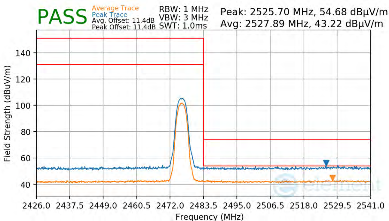
Plot 7-93. Radiated Restricted Upper Band Edge Measurement Antenna 4a
