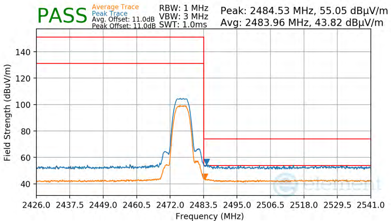
Plot 7-94. Radiated Restricted Upper Band Edge Measurement Antenna 4a
