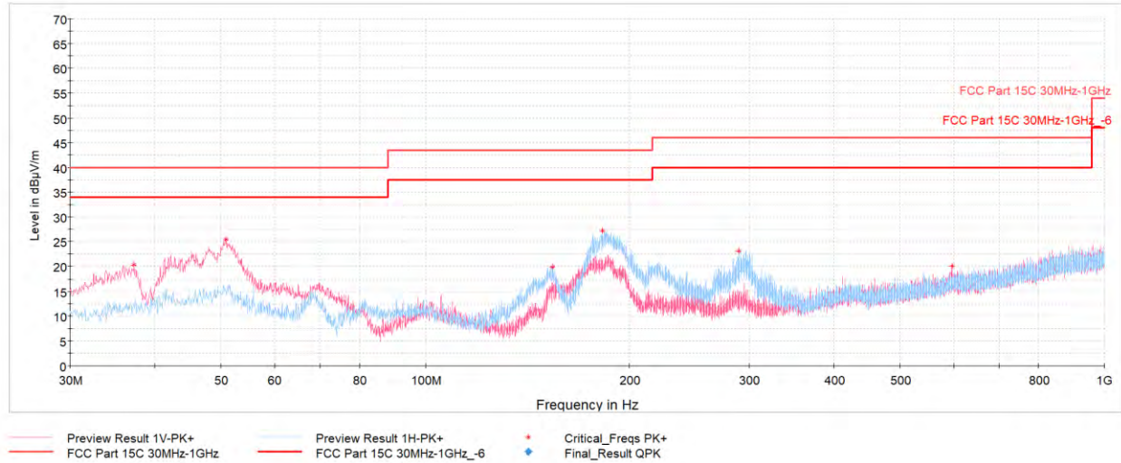
Plot 7-103. Radiated Spurious Emissions Below 1GHz TxBF (4Mbps, ePA – Ch.38 with AC/DC Adapter)
