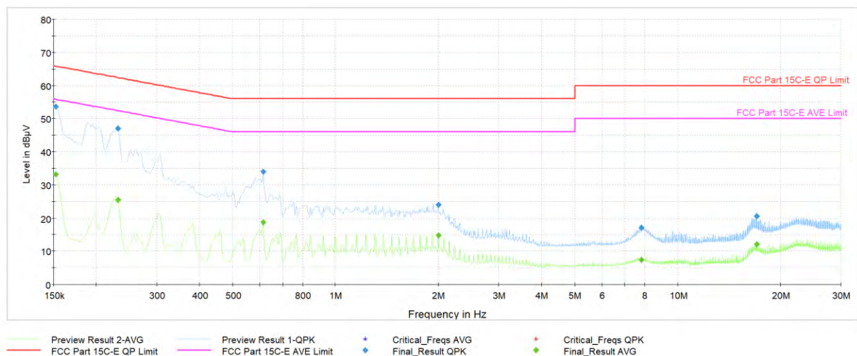
Plot 7-105. AC Line Conducted Plot with Bluetooth HDR TxBF (N, 4Mbps ePA - Ch.38 with Laptop)
