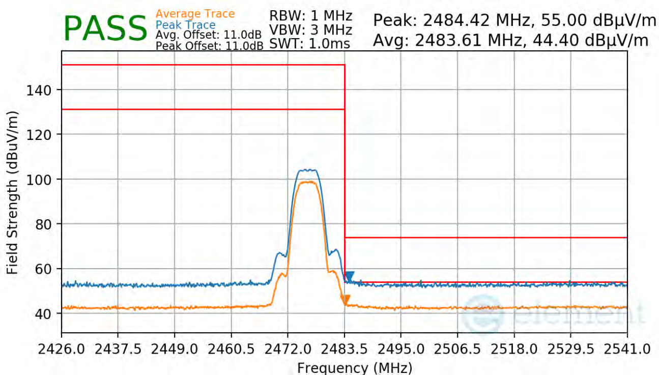
Plot 7-98. Radiated Restricted Upper Band Edge Measurement Antenna 2a
