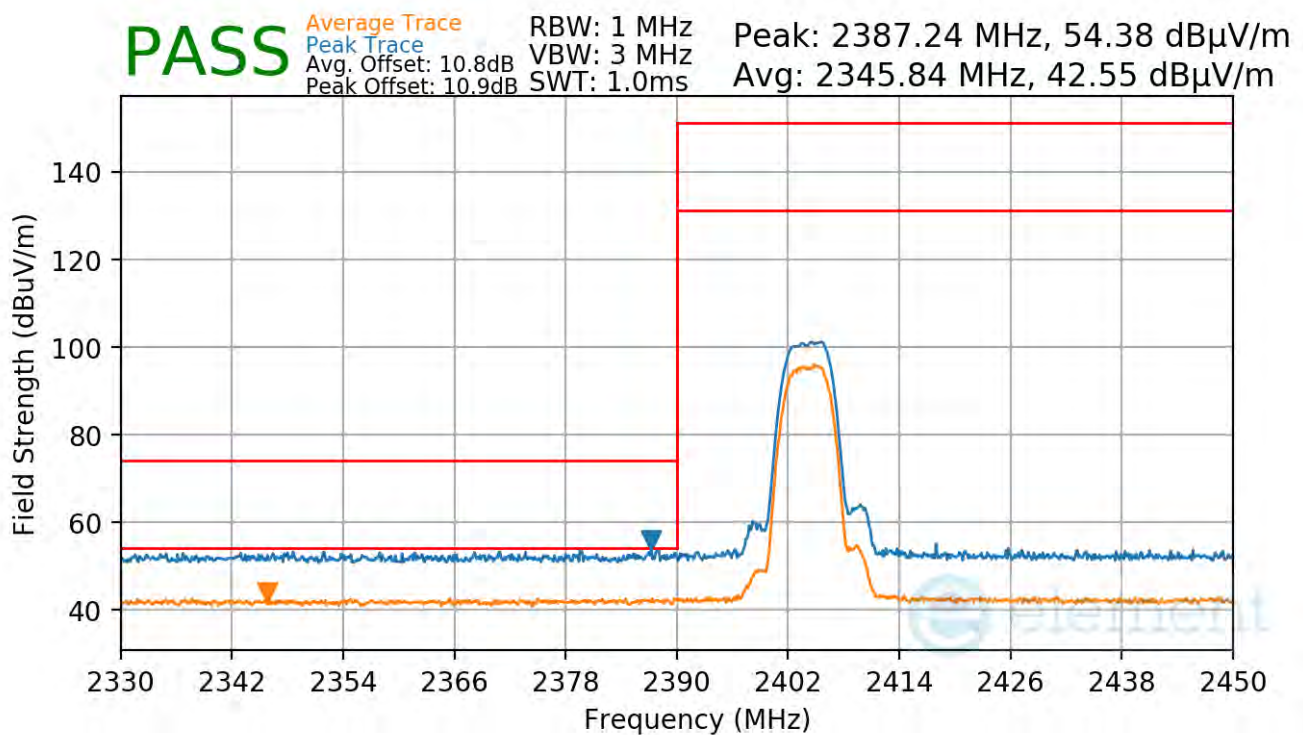
Plot 7-96. Radiated Restricted Lower Band Edge Measurement Antenna 2a
