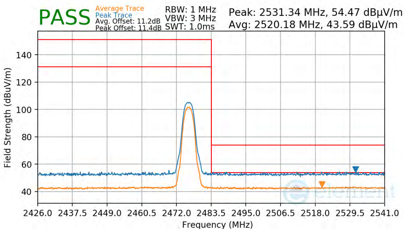
Plot 7-97. Radiated Restricted Upper Band Edge Measurement Antenna 2a
