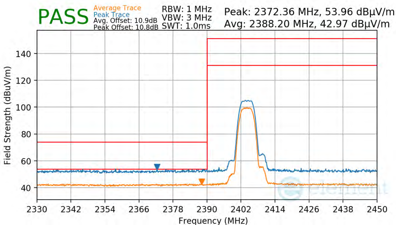
Plot 7-92. Radiated Restricted Lower Band Edge Measurement Antenna 4a
