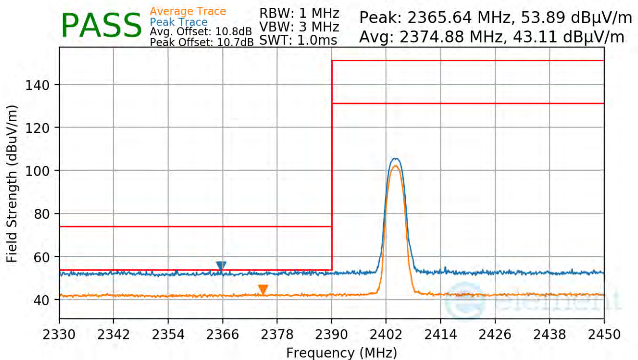
Plot 7-91. Radiated Restricted Lower Band Edge Measurement Antenna 4a
