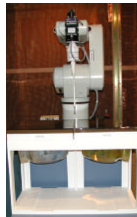
Figure 6.1 ALIDX-500 Test System
