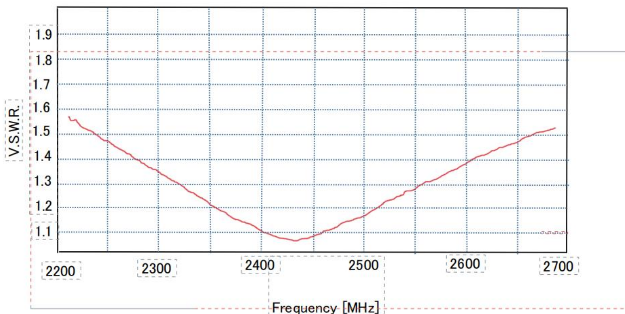
Fig.1 驻波比 VSWR
