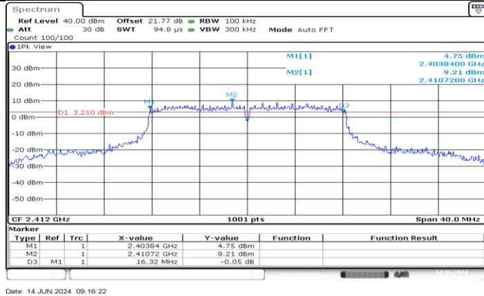
11G-CDD_Ant4_2412
