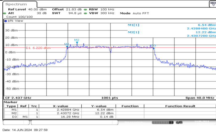
11G-CDD_Ant3_2437
