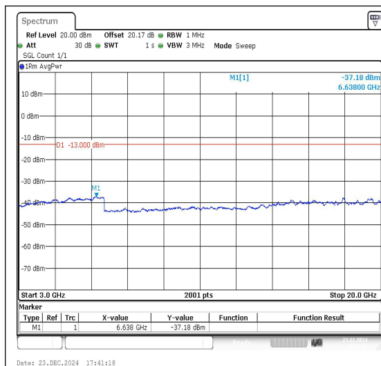
Band66_15MHz_QPSK_132597_1RB#0_3000~2 0000_3000~20000
