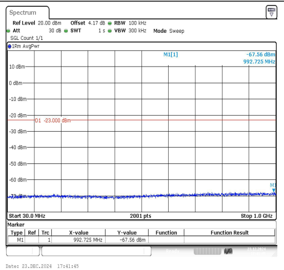
Band66_15MHz_16QAM_132597_1RB#0_30~100 0_30~1000
