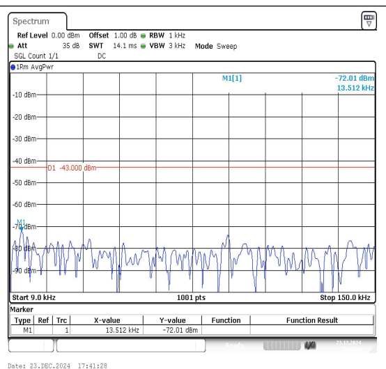
Band66_15MHz_16QAM_132597_1RB#0_0.009~ 0.15_0.009~0.15
