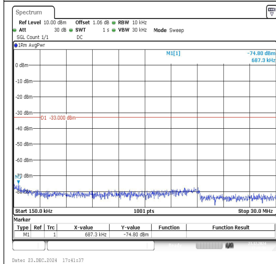
Band66_15MHz_QPSK_132597_1RB#0_0.15~ 30_0.15~30
