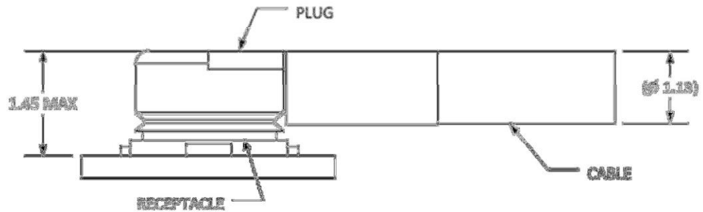
Mated Plug for \varnothing 1.13 mm Coax Cable
