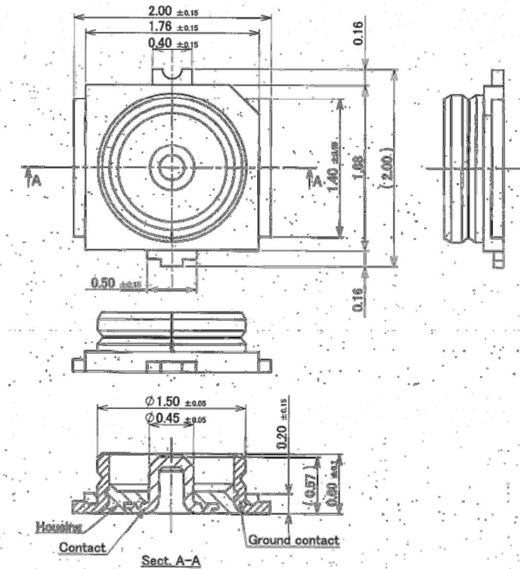
Figure 4-2 RF connectors
