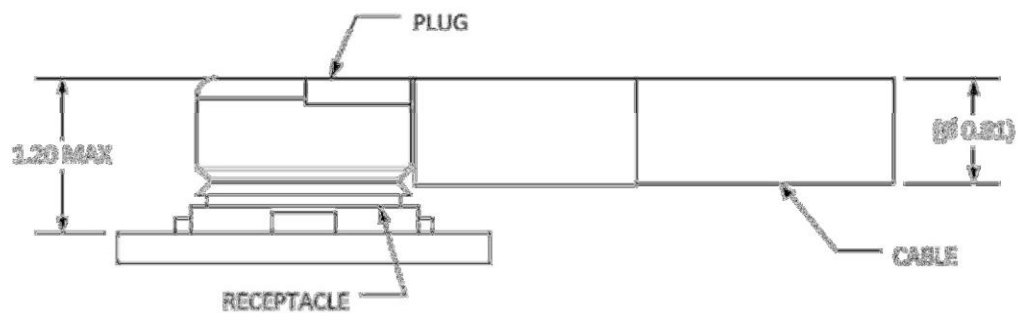
Mated Plug for \varnothing 0.81 mm Coax Cable
