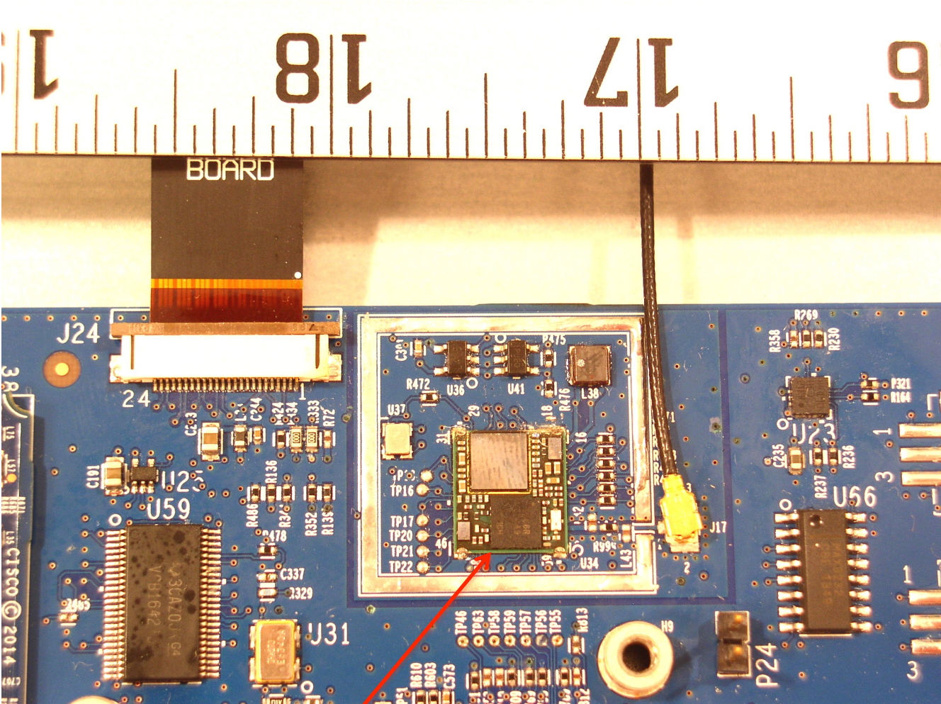
CP-DX80 : Internal PCB Mother Board (Radio Section with Shield removed)
