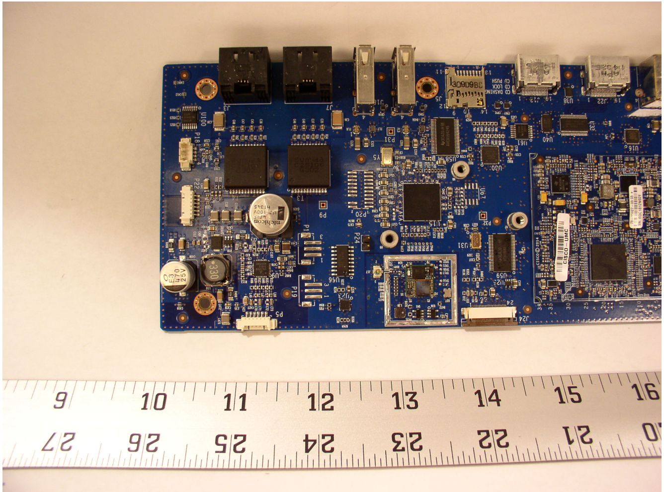
CP-DX80 : Internal PCB Mother Board (Top 1/3) close up view
