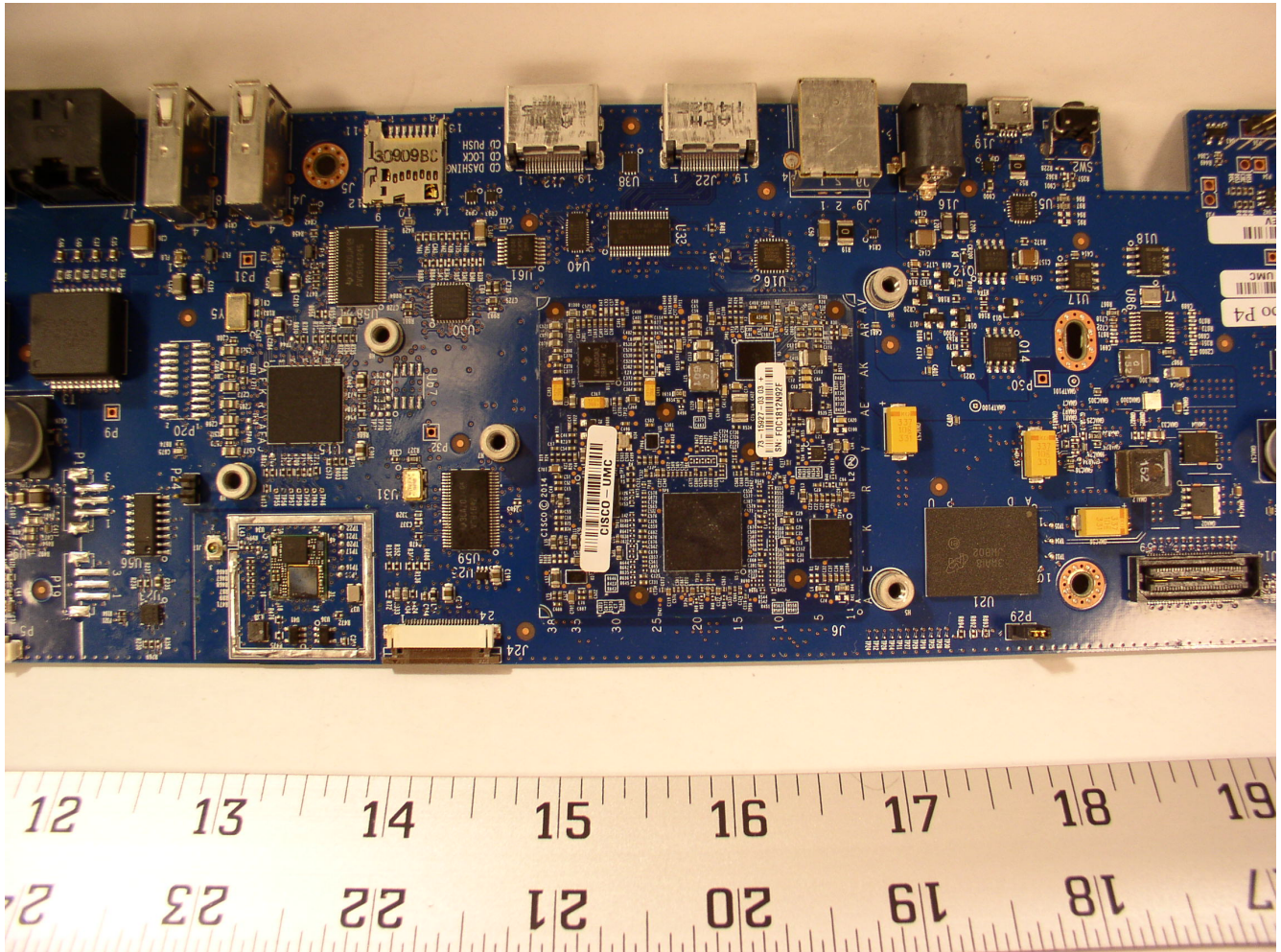
CP-DX80 : Internal PCB Mother Board (Top 2/3) close up view
