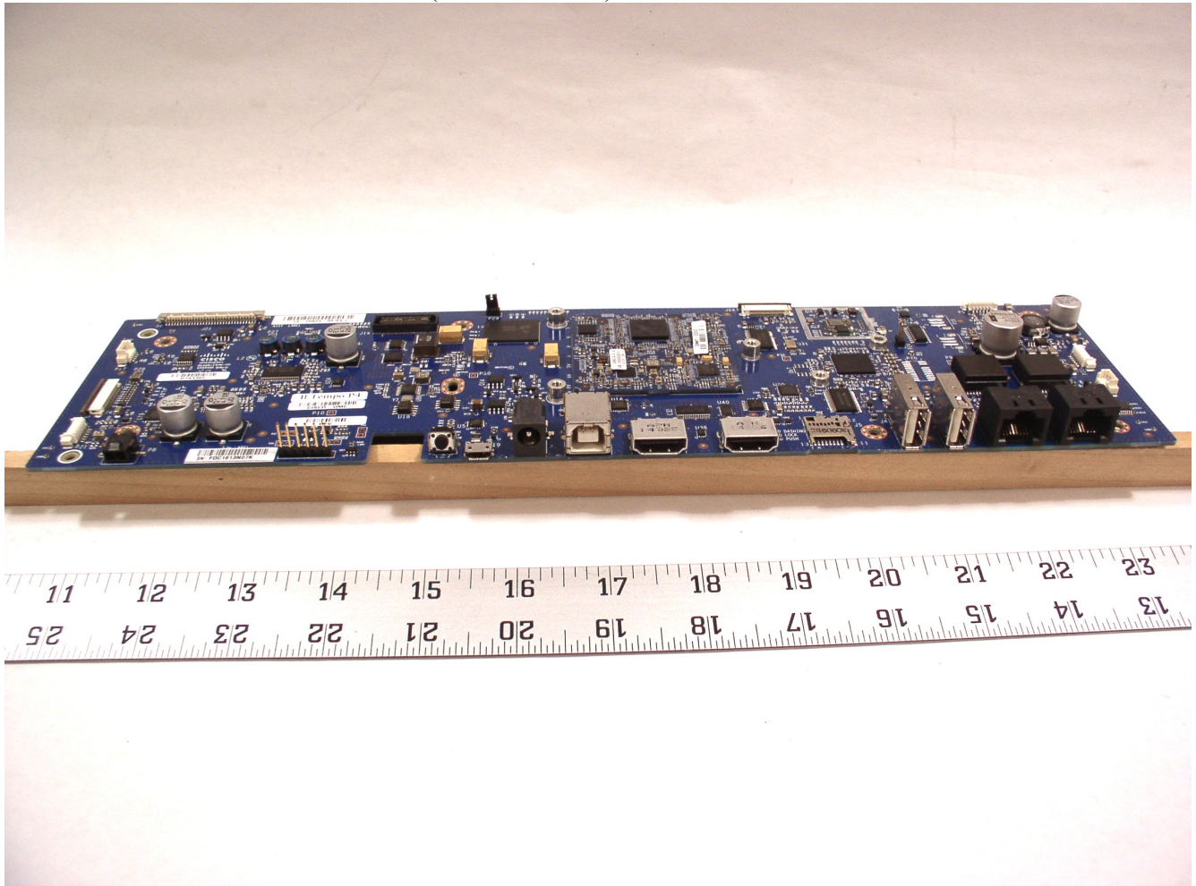
CP-DX80 : Internal PCB Mother Board (Connector view)
