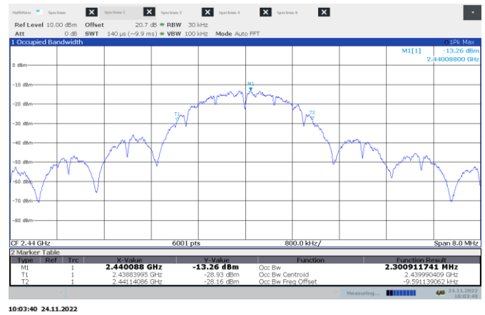
Figure 8.5-5: 99% occupied bandwidth on mid ch.
