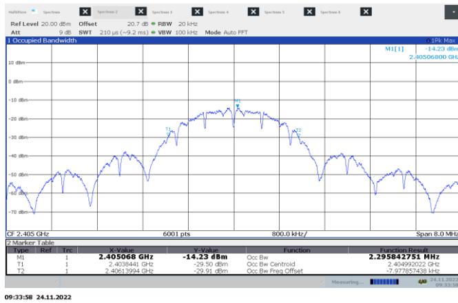
Figure 8.5-4: 99% occupied bandwidth on low ch.
