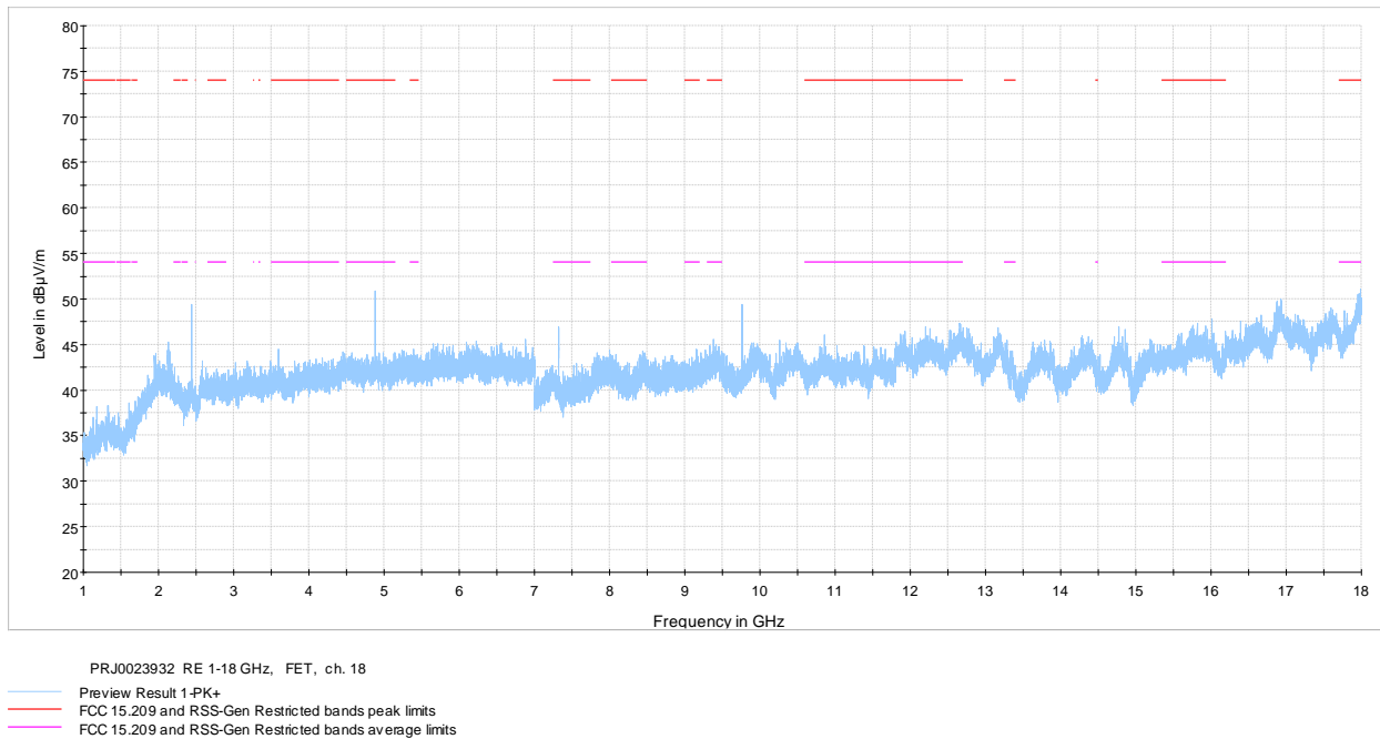
Figure 8.7-5: Radiated spurious emissions 1-18 GHz mid ch.
