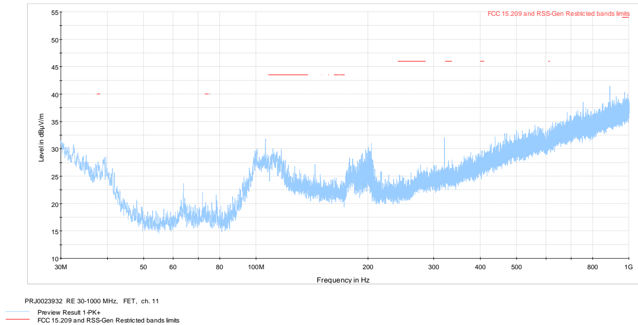
Figure 8.7-1: Radiated spurious emissions 30-1000 MHz low ch.
