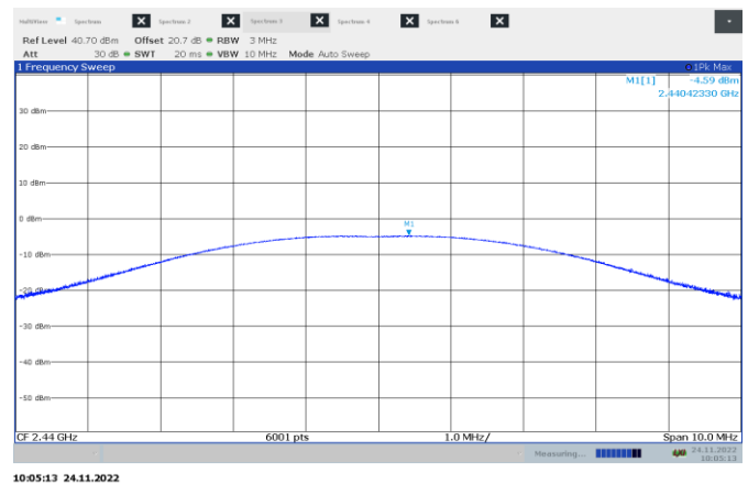
Figure 8.6-2: Output power on mid ch.
