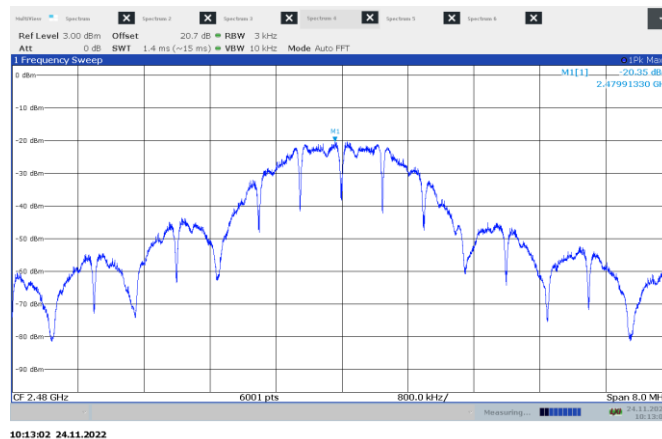
Figure 8.8-3: PSD on high ch.
