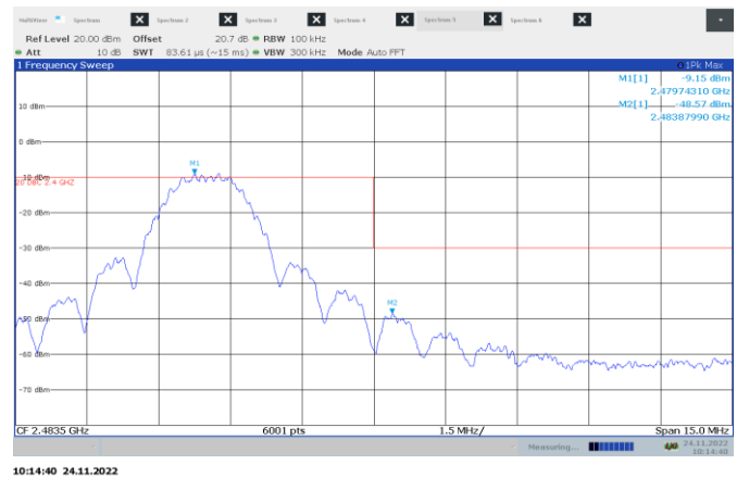
Figure 8.7-15: Conducted non-restricted band edge emissions at 2483.5 MHz
