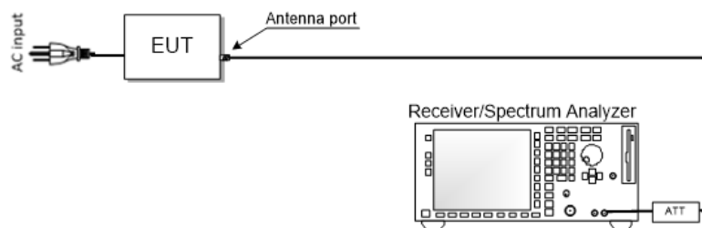
Figure 5.5-2: Antenna port testing block diagram
