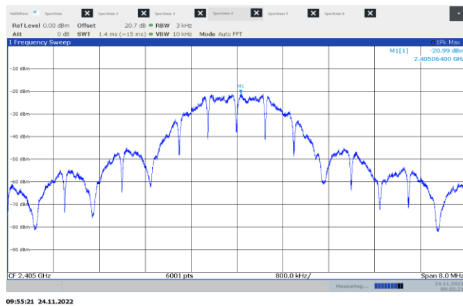
Figure 8.8-1: PSD on low ch.
