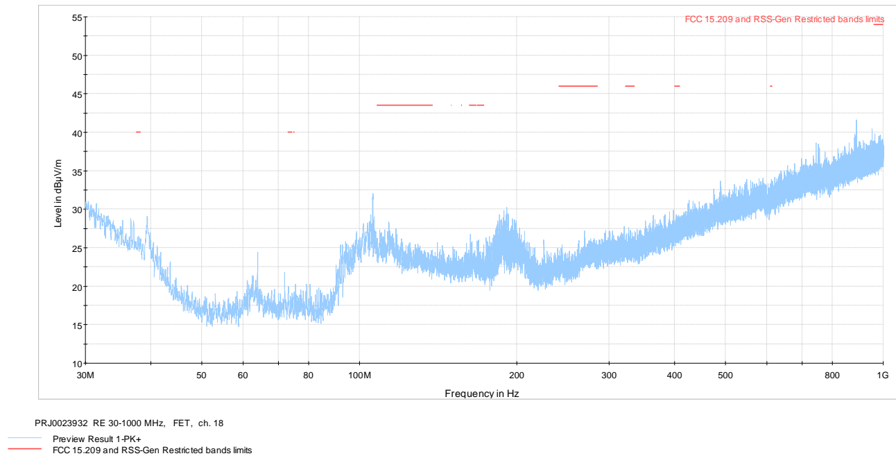
Figure 8.7-2: Radiated spurious emissions 30-1000 MHz mid ch.
