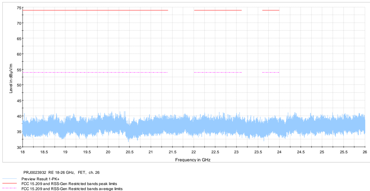
Figure 8.7-9: Radiated spurious emissions 18-26 GHz high ch.
