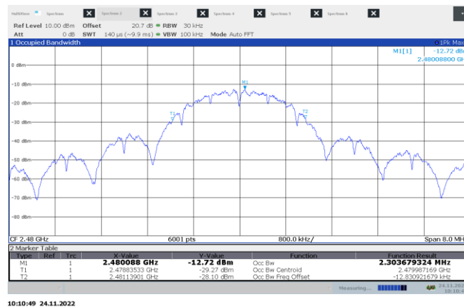
Figure 8.5-6: 99% occupied bandwidth on high ch.
