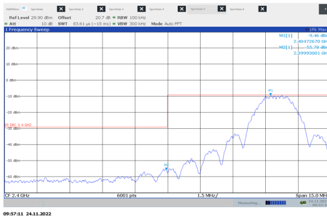
Figure 8.7-14: Conducted non-restricted band edge emissions at 2400 MHz
