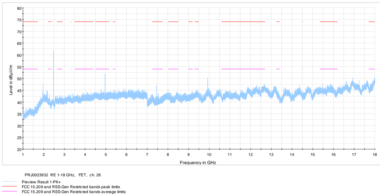
Figure 8.7-6: Radiated spurious emissions 1-18 GHz high ch.
