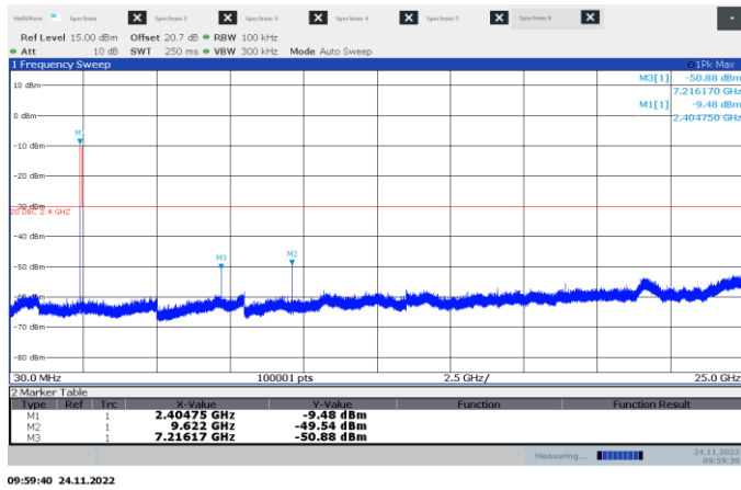
Figure 8.7-16: Conducted spurious emissions at low ch.
