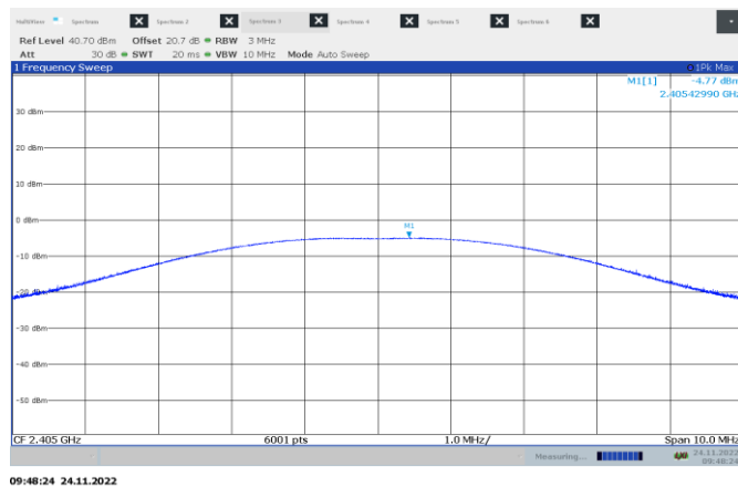
Figure 8.6-1: Output power on low ch.
