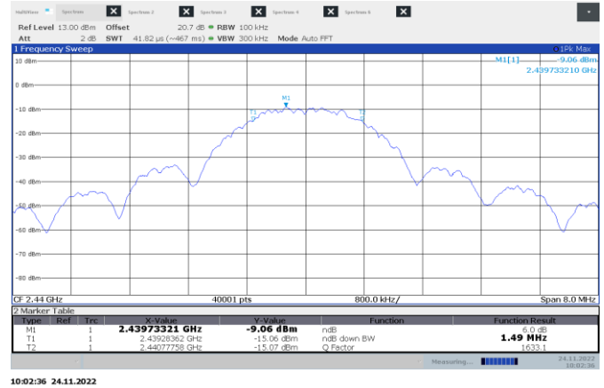
Figure 8.5-2: 6 dB bandwidth on mid ch.
