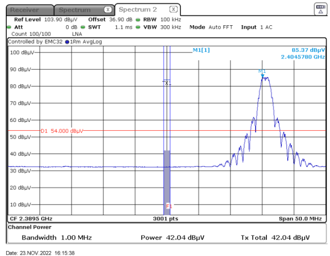
Figure 8.7-11: Radiated band edge spurious emissions at 2390 MHz Average
