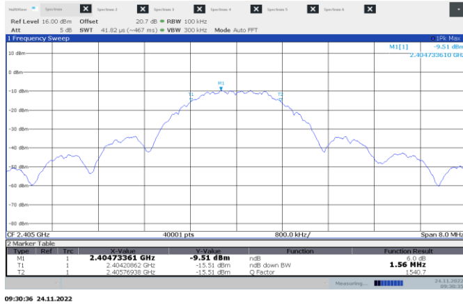
Figure 8.5-1: 6 dB bandwidth on low ch.
