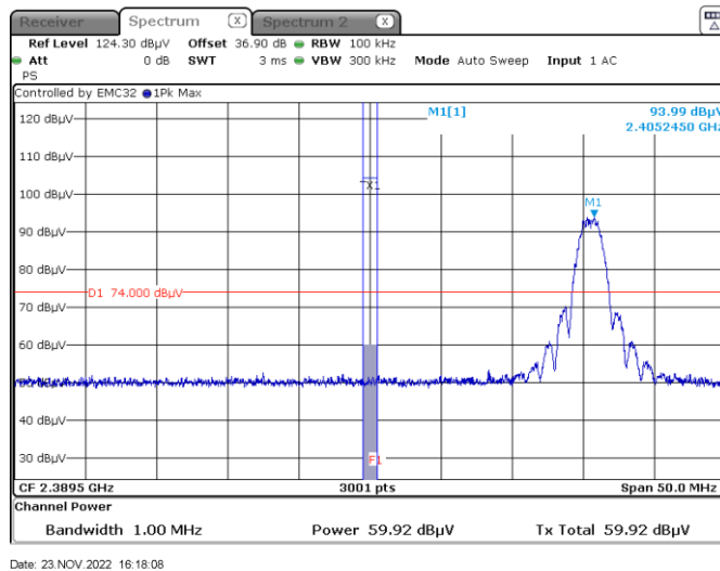
Figure 8.7-10: Radiated band edge spurious emissions at 2390 MHz Peak
