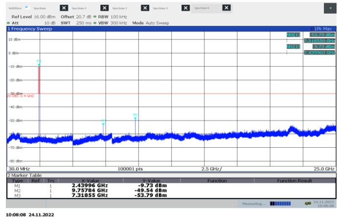
Figure 8.7-17: Conducted spurious emissions at mid ch.
