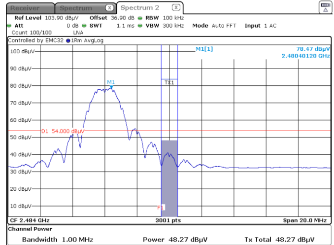
Figure 8.7-13: Radiated band edge spurious emissions at 2483.5 MHz Average
