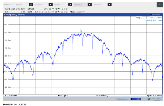
Figure 8.8-2: PSD on mid ch.
