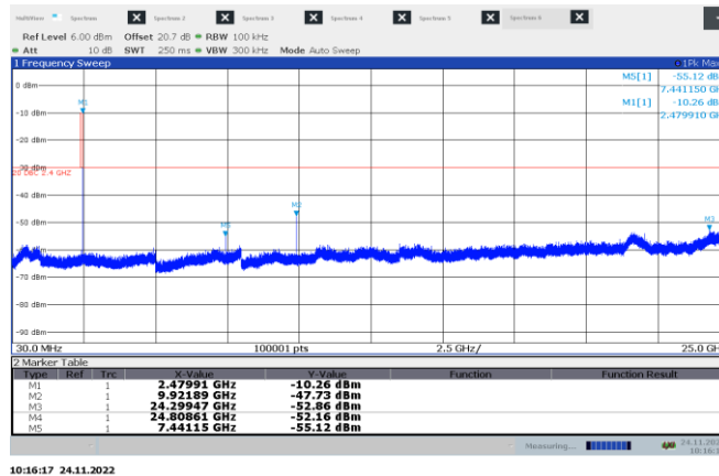
Figure 8.7-18: Conducted spurious emissions at high ch.
