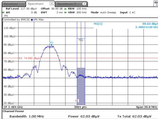
Figure 8.7-12: Radiated band edge spurious emissions at 2483.5 MHz Peak
