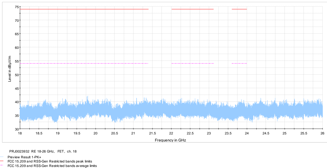
Figure 8.7-8: Radiated spurious emissions 18-26 GHz mid ch.
