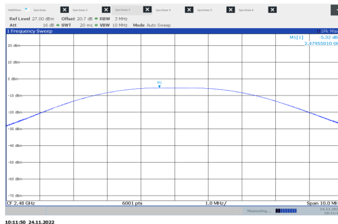
Figure 8.6-3: Output power on high ch.
