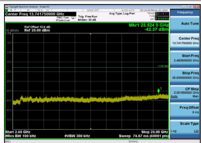
,Plot 4,2483.5MHz~25000MHz-802.11g
