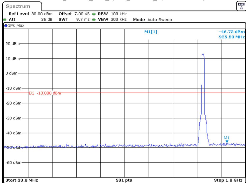
Band 5_10 MHz_Low_QPSK_RB50#0_1(30MHz-1GHz)
