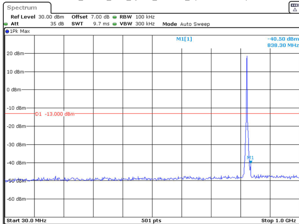
Band 5_3 MHz_Low_QPSK_RB15#0_1(30MHz-1GHz)
