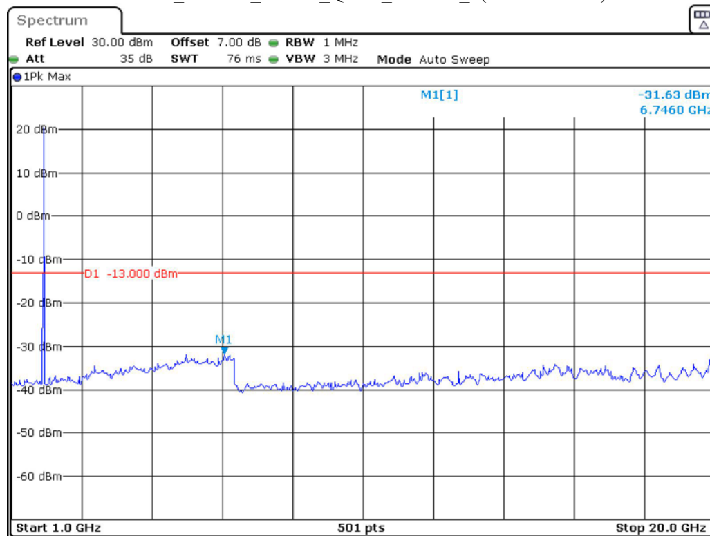
Band 2_10 MHz_Middle_QPSK_RB50#0_2(1GHz-20GHz)
