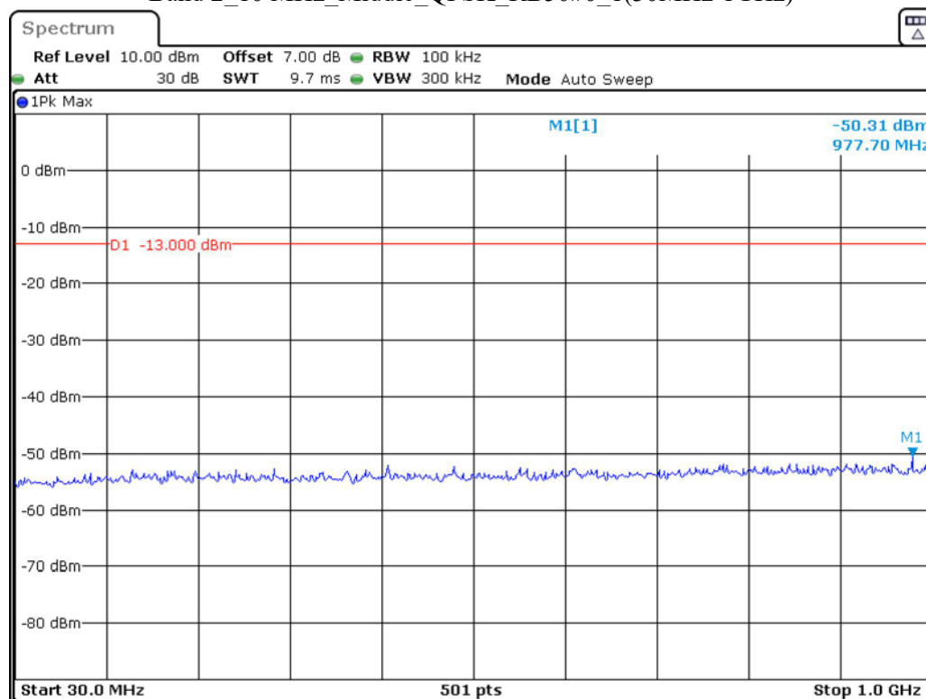
Band 2_10 MHz_Middle_QPSK_RB50#0_1(30MHz-1GHz)
