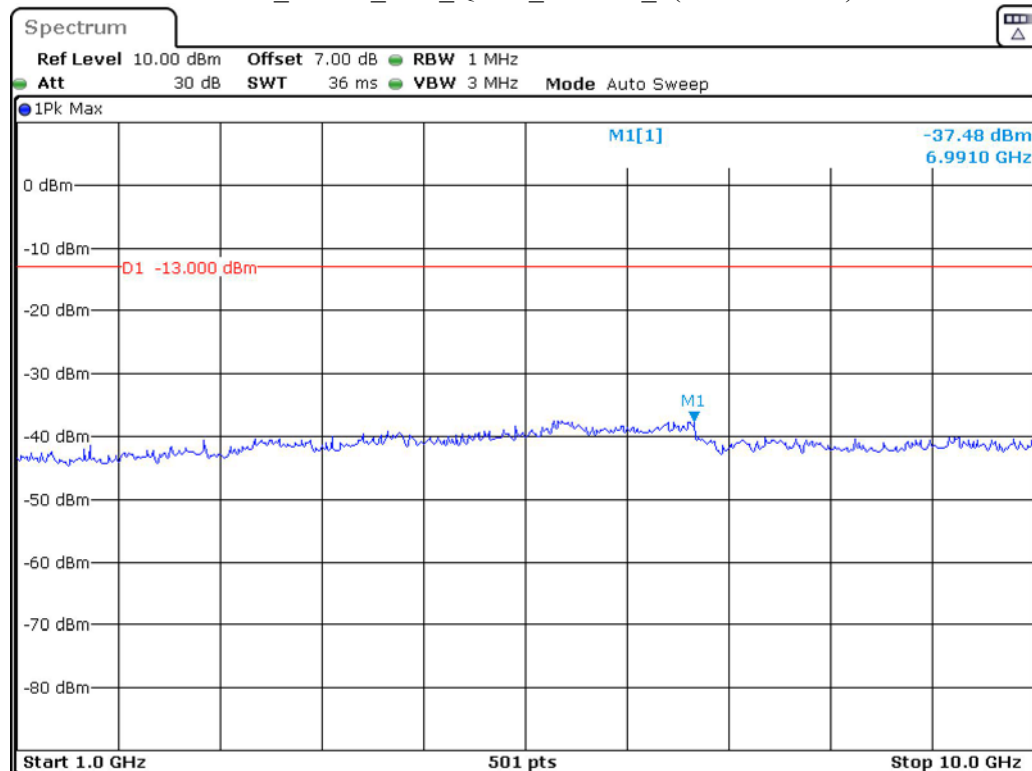
Band 5_3 MHz_Low_QPSK_RB15#0_2(1GHz-10GHz)
