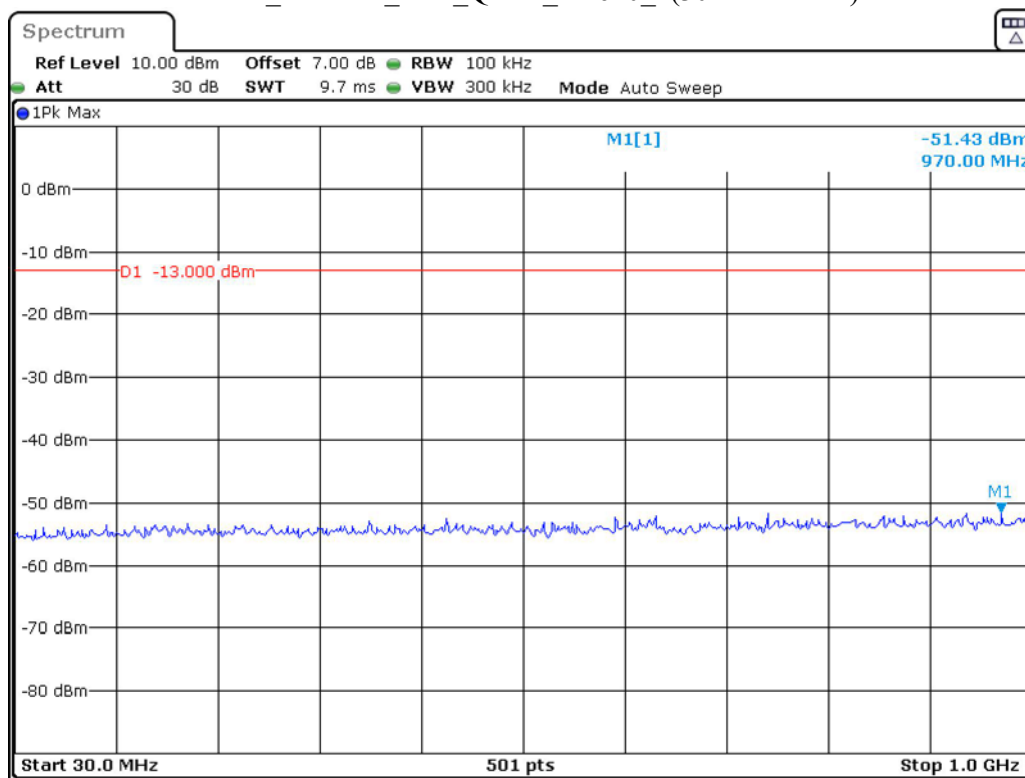
Band 2_1.4 MHz_Low_QPSK_RB6#0_1(30MHz-1GHz)
