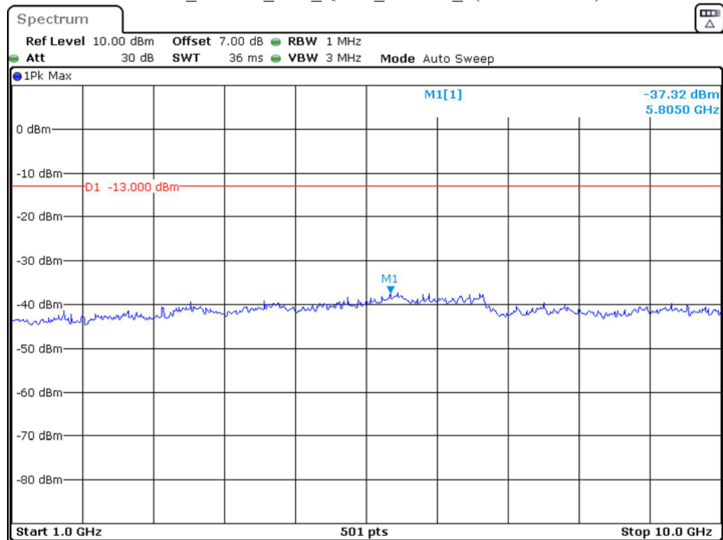
Band 5_10 MHz_Low_QPSK_RB50#0_2(1GHz-10GHz)
