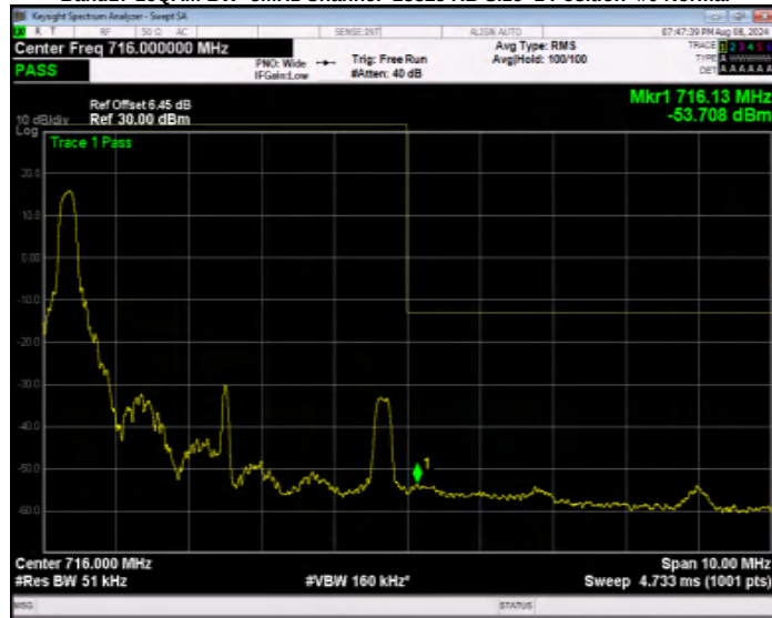
Band17 16QAM BW=5MHz Channel=23825 RB Size=1 Position=#Max Extended
