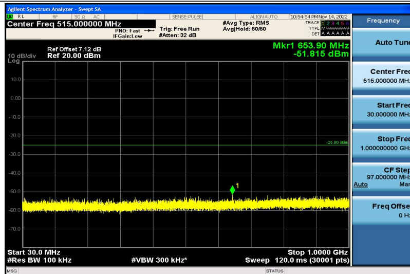
Band7-10MHz-QPSK-21100-1RB#0-30~1000MHz
