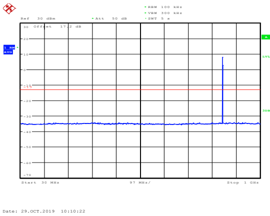
LTE Band 5 1.4MHz CH-High 30MHz~1GHz
