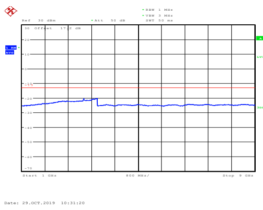
LTE Band 5 1.4MHz CH-High 1GHz ~9GHz
