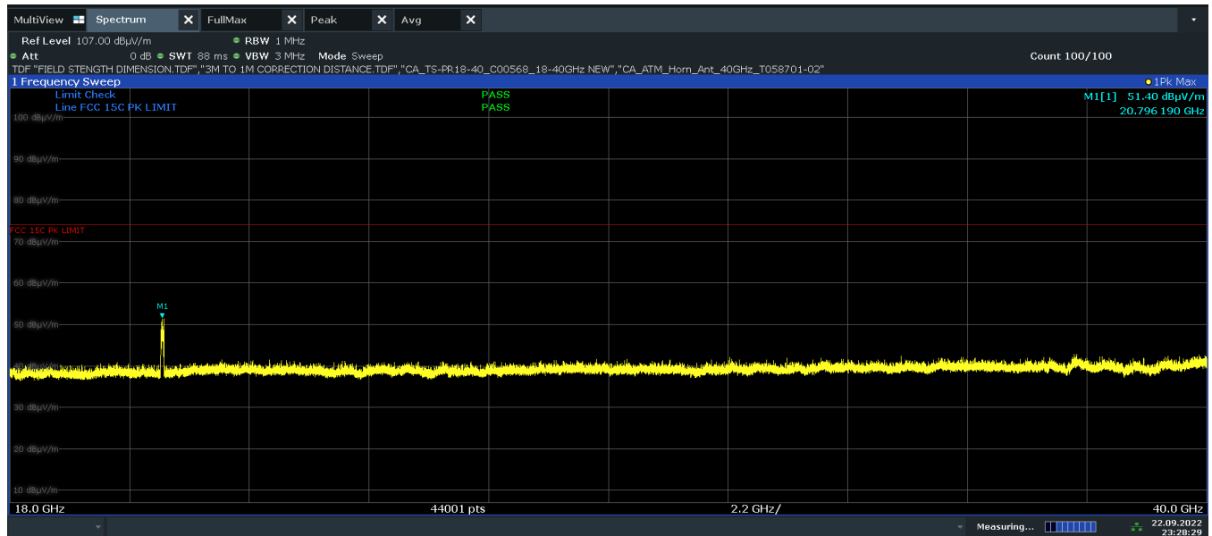
Plot 7-35. Radiated Spurious Emissions Simultaneous Transmission Above 18GHz Ant. Pol. H
