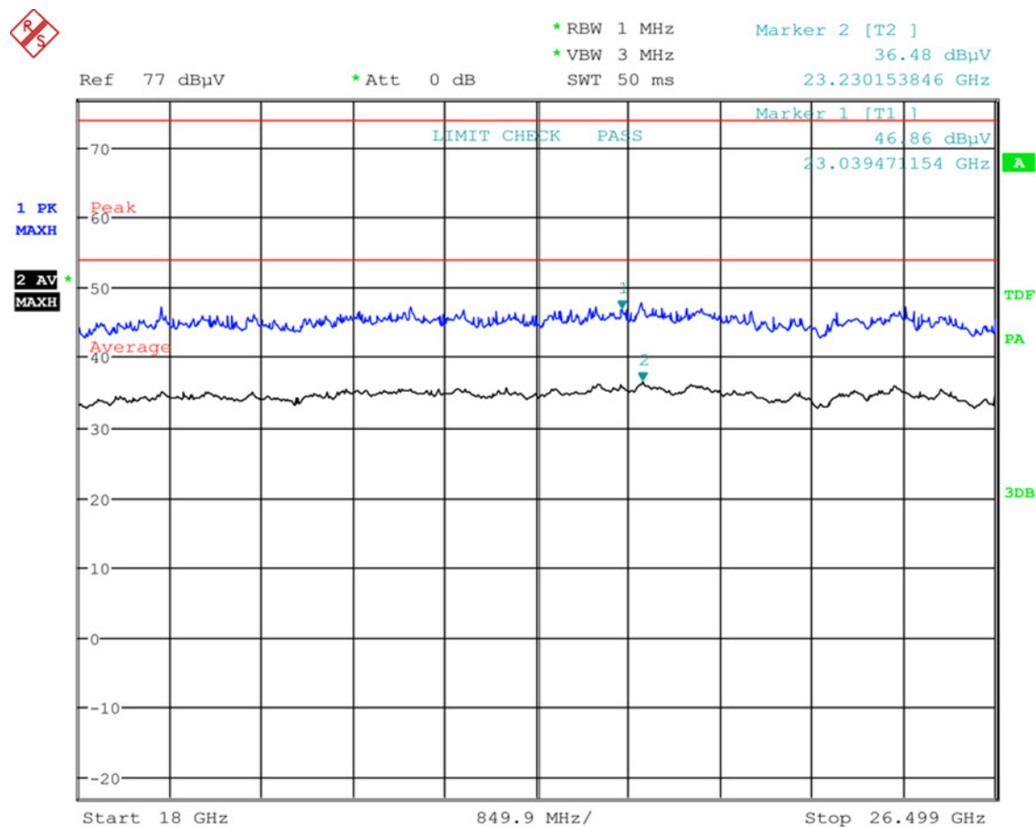
Plot 6-545: Radiated Emissions of Carrier - TC #9 Fiberglass Container
