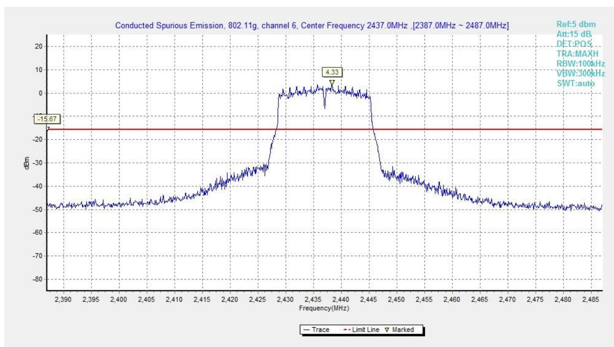
Fig.A.6.1.33 Conducted Spurious Emission (802.11g, Ch6, Center Frequency)
