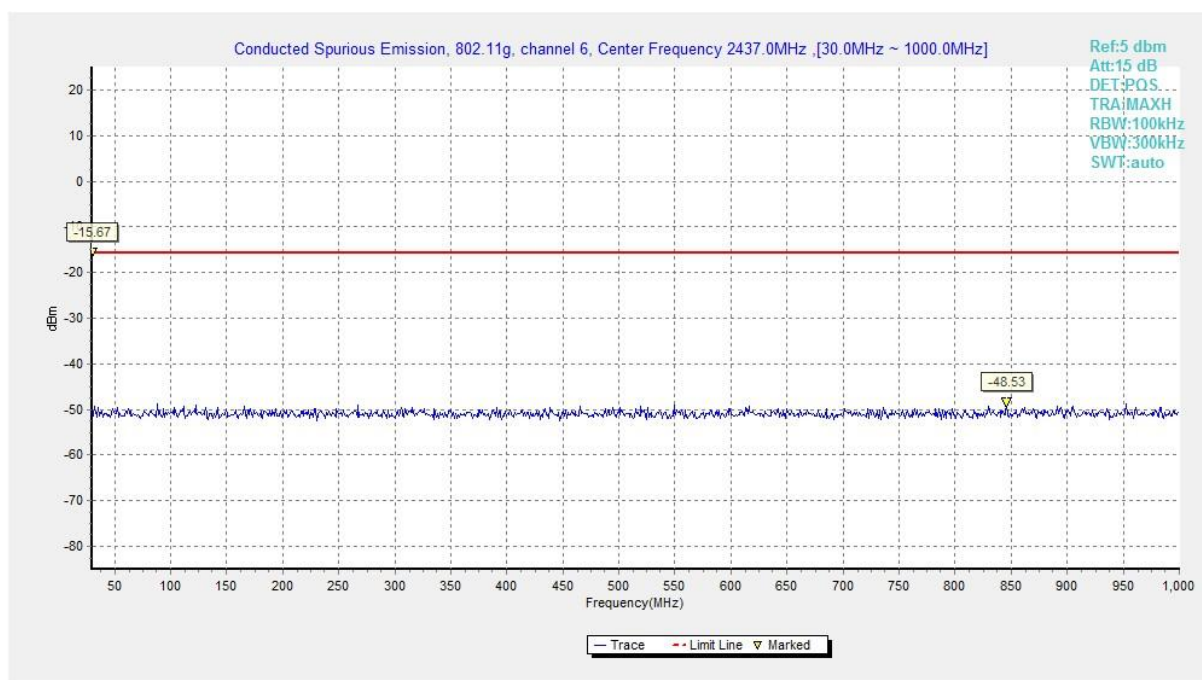
Fig.A.6.1.34 Conducted Spurious Emission (802.11g, Ch6, 30 MHz-1 GHz)
