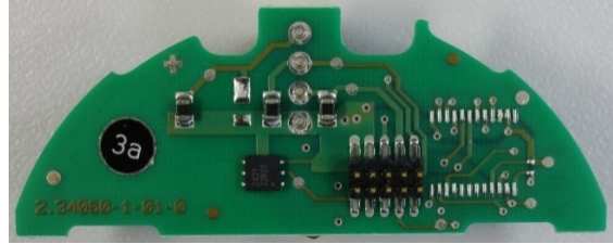
Bottom View
