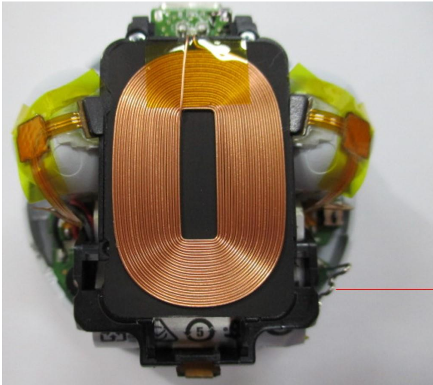
Figure E-1 Antenna Location (Rear Side View)
