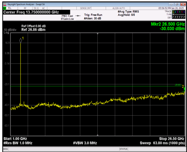
Band7-5MHz-64QAM-21100-1RB#0-Range2:1000~2 6500MHz
