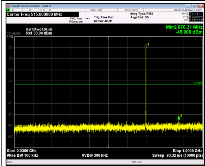
Band12-1.4MHz-64QAM-23095-1RB#0-Range1:30~1000MHz
