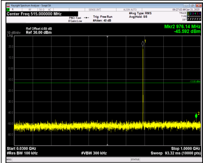
Band12-1.4MHz-64QAM-23095-1RB#0-Range1:30~1000MHz
