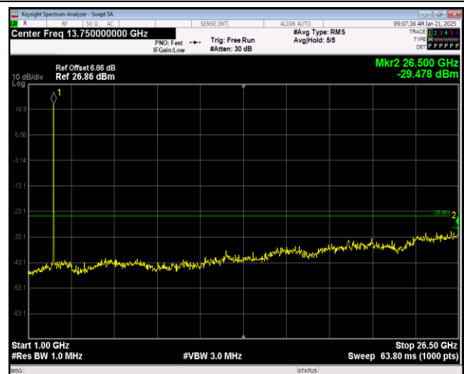
Band7-20MHz-16QAM-21100-1RB#0-Range2:1000~ 26500MHz
