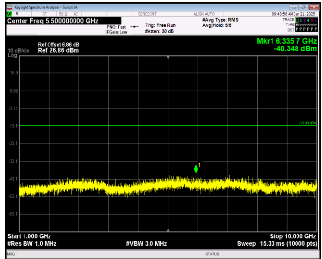
Band12-10MHz-16QAM-23130-1RB#0-Range2:1000 ~10000MHz
