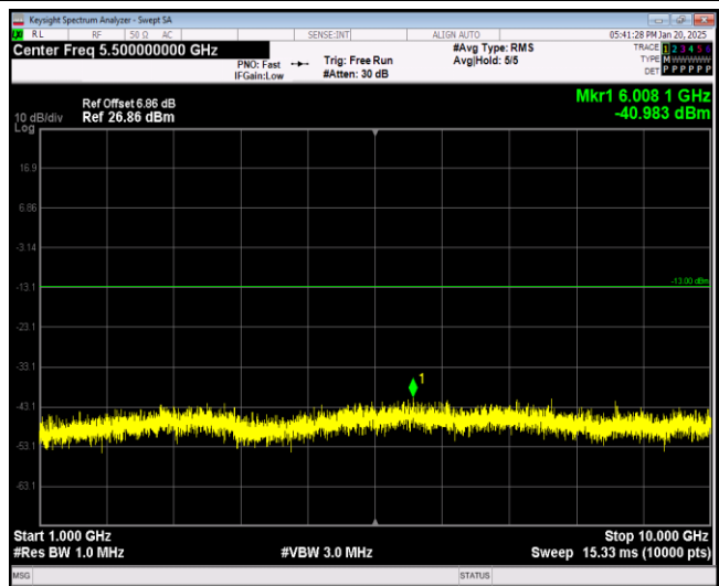
Band5-10MHz-64QAM-20525-1RB#0-Range2:1000~10000MHz
