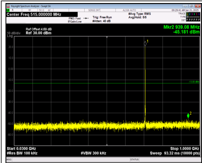
Band12-1.4MHz-64QAM-23017-1RB#0-Range1:30~1000MHz
