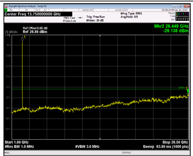
Band7-5MHz-16QAM-21425-1RB#0-Range2:1000~26500MHz
