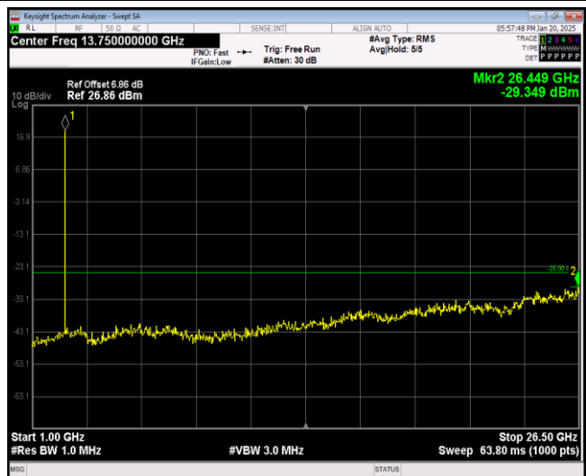
Band7-5MHz-64QAM-21425-1RB#0-Range2:1000~2 6500MHz
