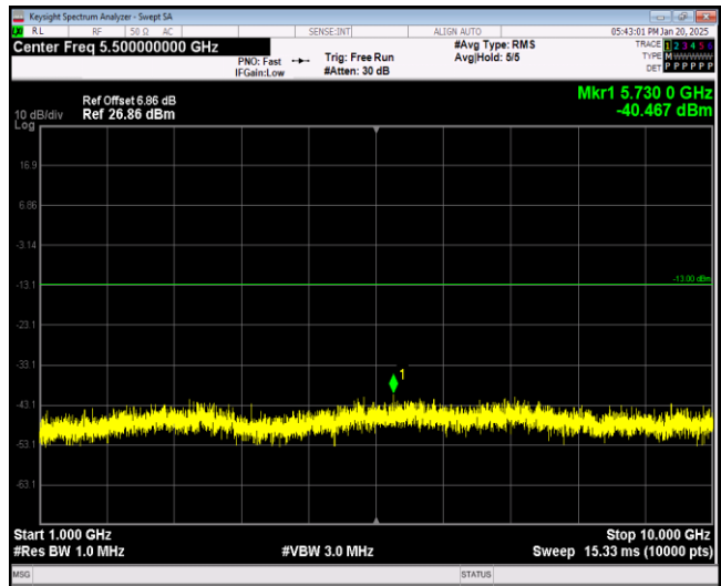
Band5-10MHz-64QAM-20450-1RB#0-Range2:1000~10000MHz
