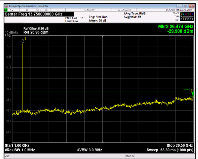
Band7-5MHz-16QAM-21425-1RB#0-Range2:1000~26500MHz
