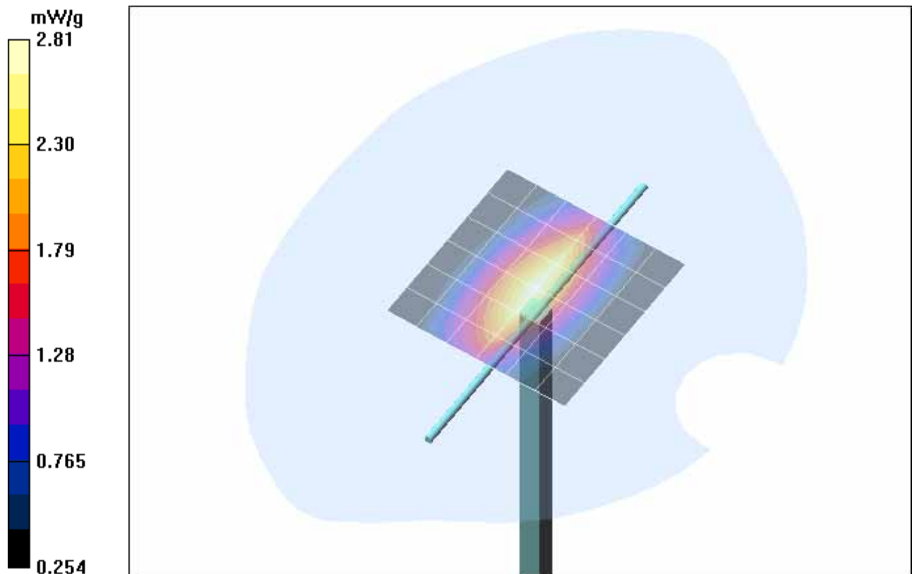
Fig. 12: Validation measurement 835MHz Body (GSM 850 and WCDMA V, January 16, 2006), coarse grid. Ambient Temperature: 21.2^\circ\text{C} , Liquid Temperature: 20.1^\circ\text{C} .
