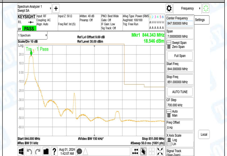
Band5_5MHz_QPSK_20625_25RB#0
