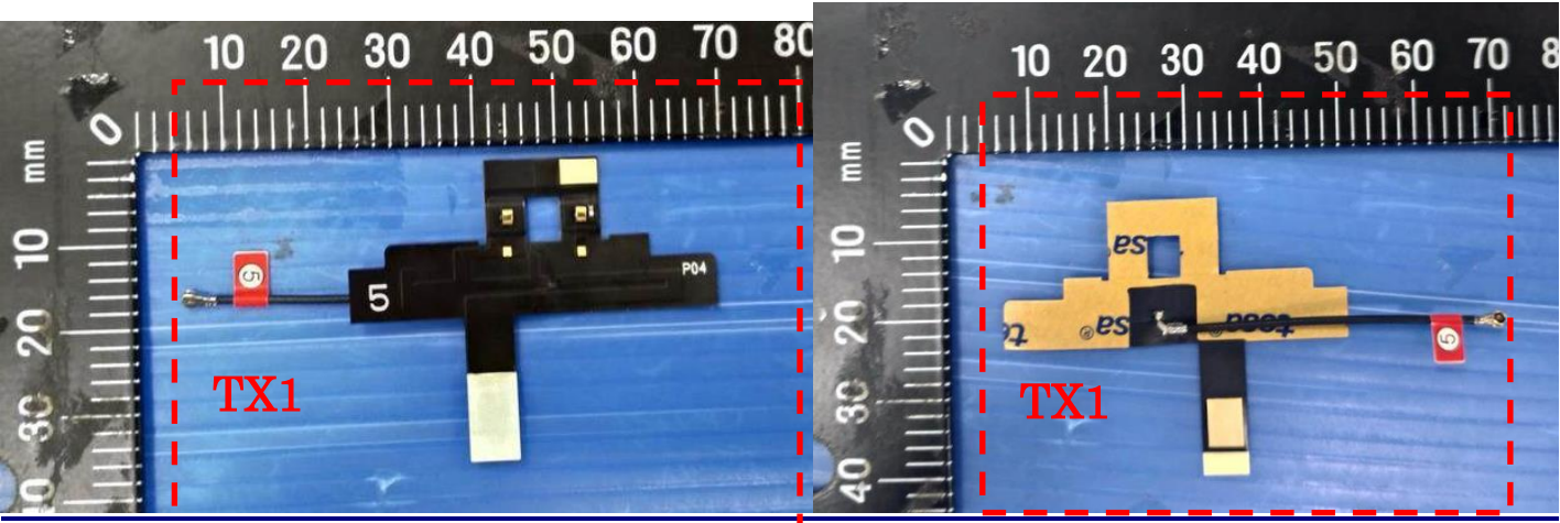
Tx1 Antenna Photo:
