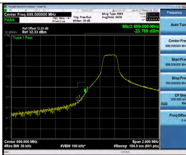
Band12-5MHz-64QAM-23035-25RB#0
