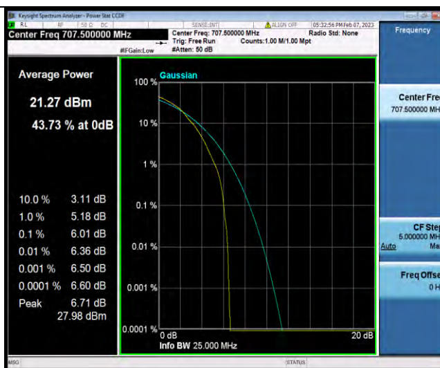
Band12-10MHz-64QAM-23095-50RB#0
