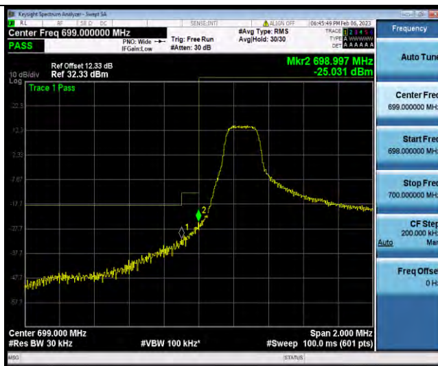
Band12-1.4MHz-64QAM-23017-6RB#0
