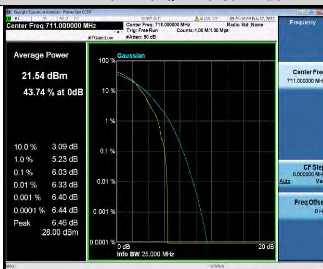
Band12-10MHz-64QAM-23130-50RB#0
