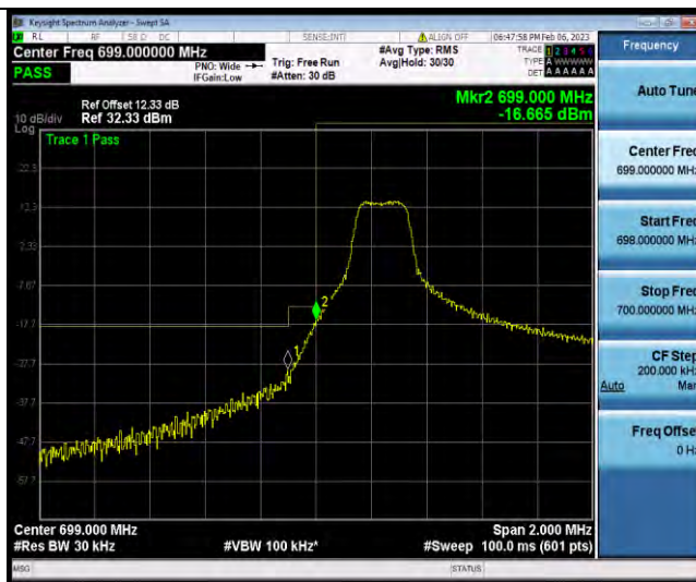
Band12-3MHz-64QAM-23025-15RB#0
