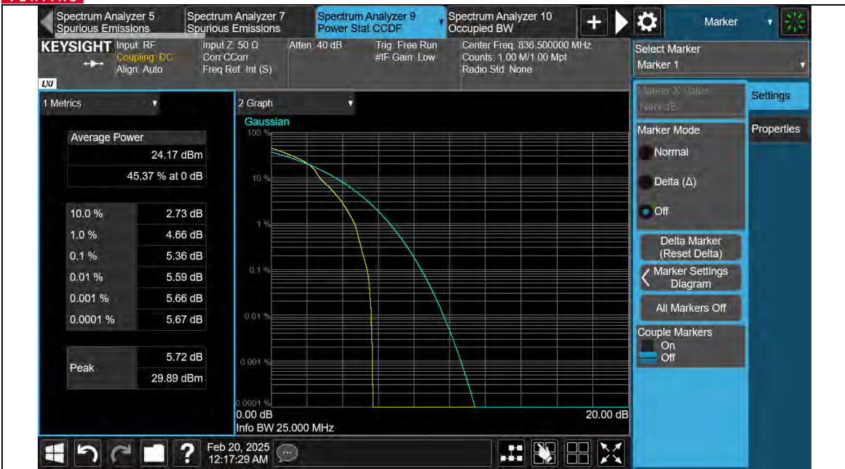
Band26-15MHz-16QAM-26915-27RB#0
