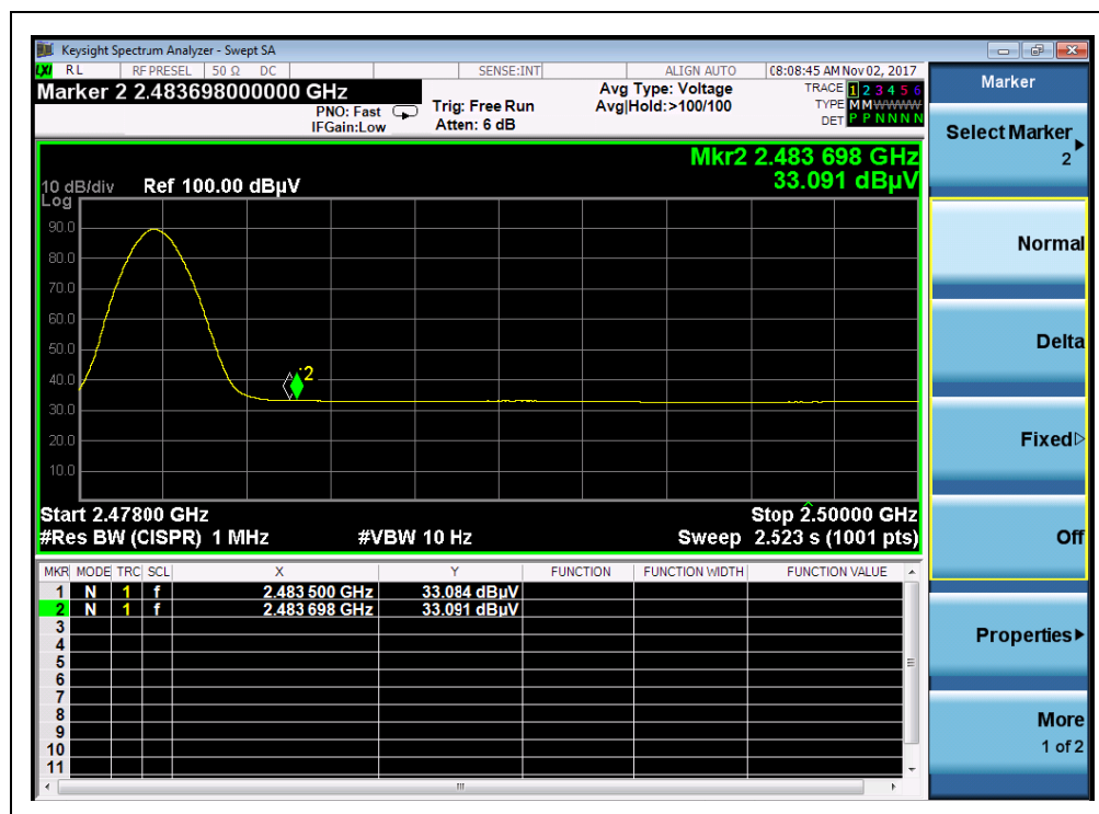
(Plot F2:Channel = 78 AVERAGE @ 8-DPSK Mode)
