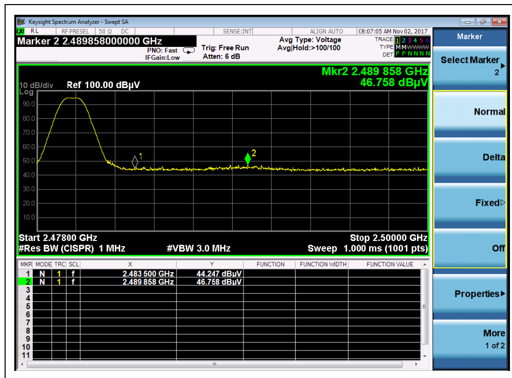
(Plot F1:Channel = 78 PEAK @ 8-DPSK Mode)
