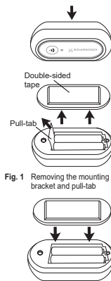
Fig. 2 Replacing the mounting bracket
