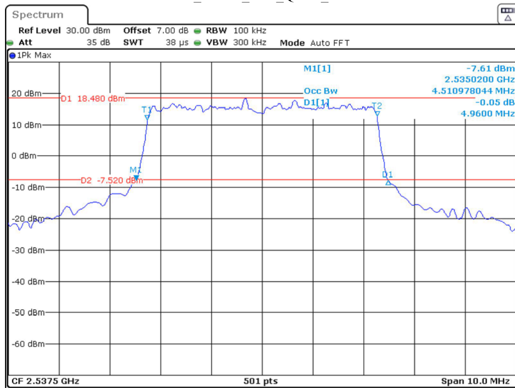
Band 41_5 MHz_Low_QPSK_RB25#0
