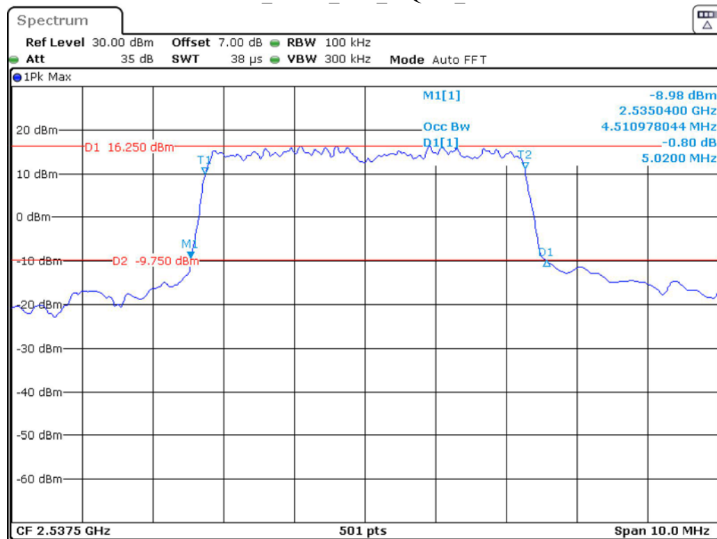
Band 41_5 MHz_Low_16QAM_RB25#0
