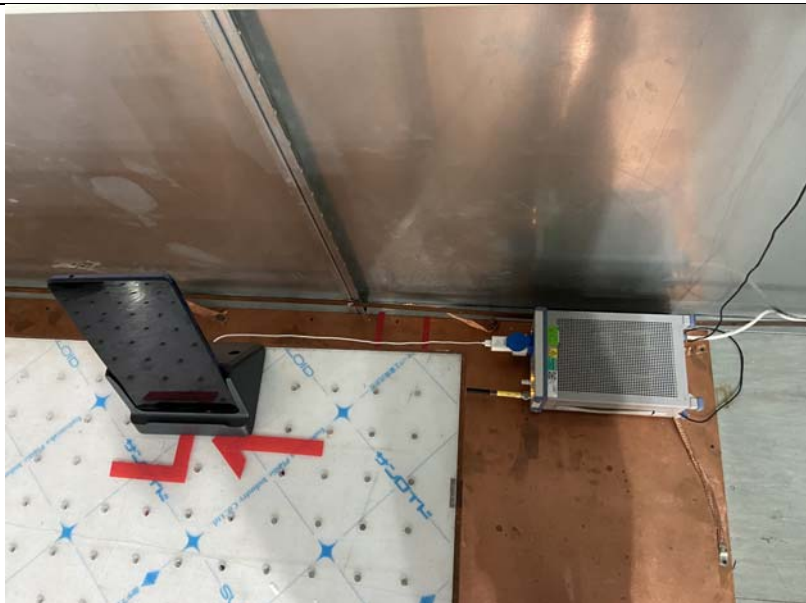
Conducted Emissions Test Setup (with charger)
