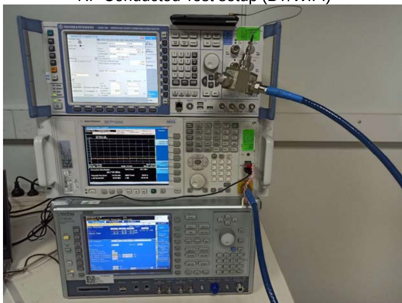
RF Conducted Test setup (WCDMA/LTE)
