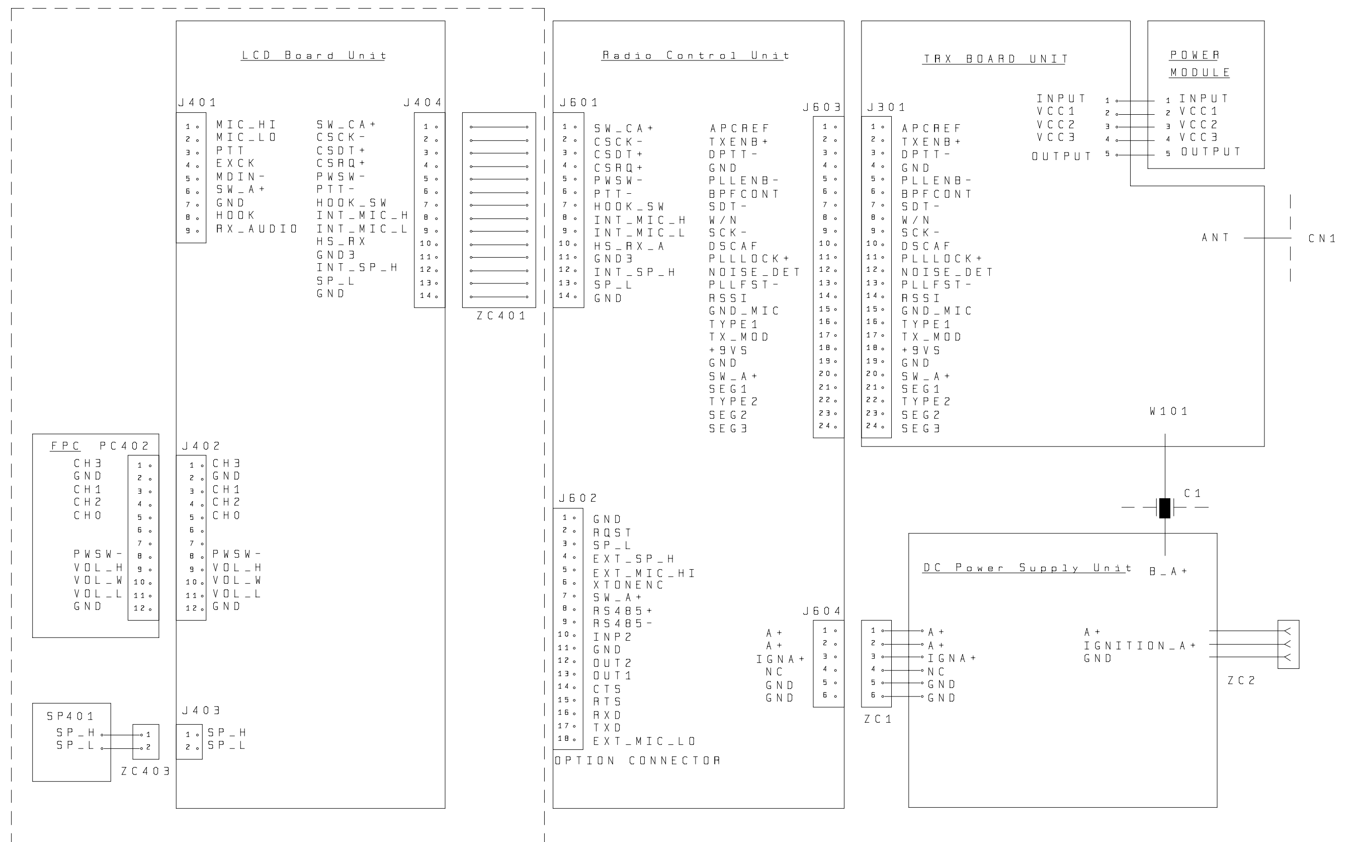
Schematic of KME800 Interconnection For FCC XD00-DTF-114S
