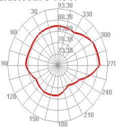
Bluetooth 0 TIS H
