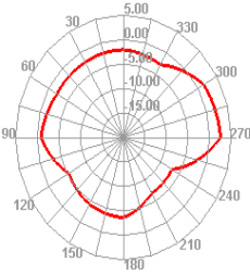
Bluetooth 39 TRP H
