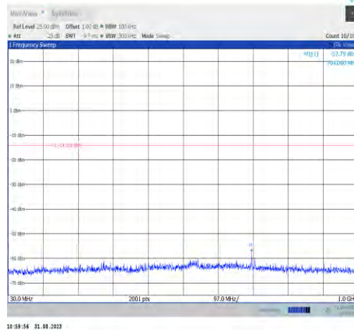
11n20MIMO-Ant9-2412-30~1000-PASS
