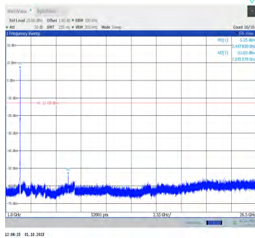
11n20MIMO-Ant7-2447-1000~26500-PASS
