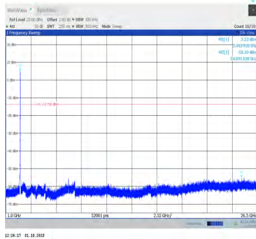
11ax20MIMO-Ant7-2447-1000~26500-PASS
