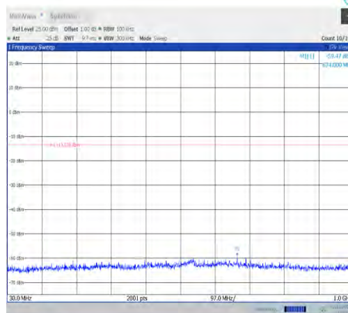
11ax20MIMO-Ant9-2422-30~1000-PASS
