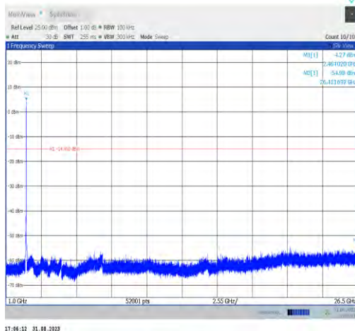
11ax20MIMO-Ant9-2462-1000~26500-PASS
