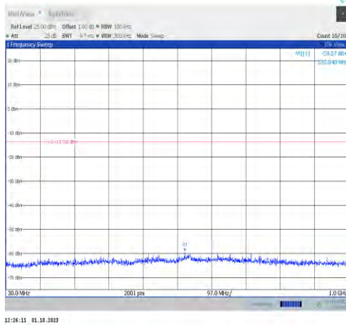
11ax20MIMO-Ant7-2447-30~1000-PASS
