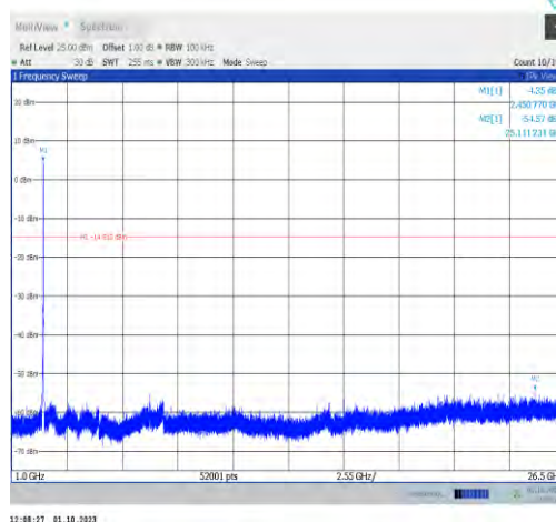
11n20MIMO-Ant7-2452-1000~26500-PASS
