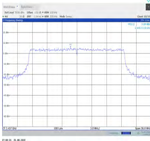
11ax20MIMO-Ant9-2437-0~Reference-PASS
