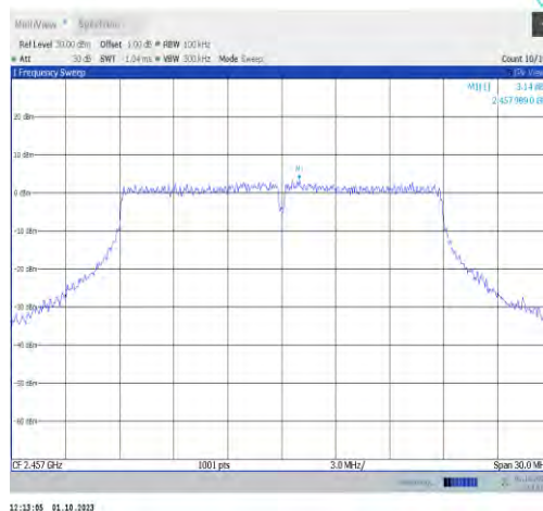
11n20MIMO-Ant7-2457-0~Reference-PASS
