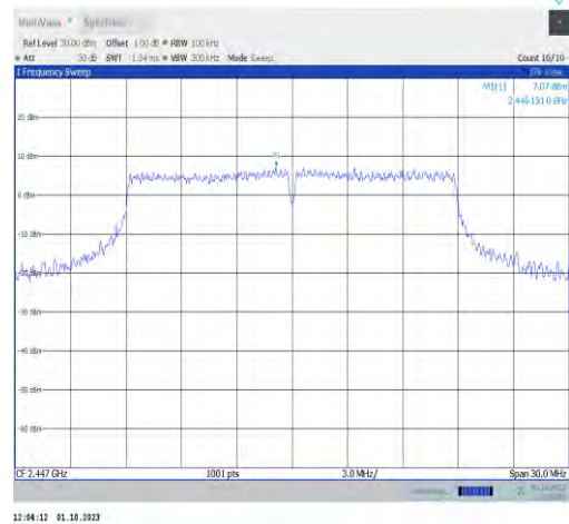
11n20MIMO-Ant7-2447-0~Reference-PASS
