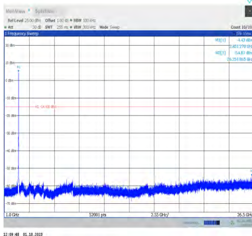
11n20MIMO-Ant9-2452-1000~26500-PASS
