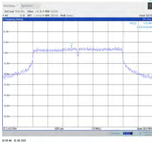
11n20MIMO-Ant9-2412-0~Reference-PASS
