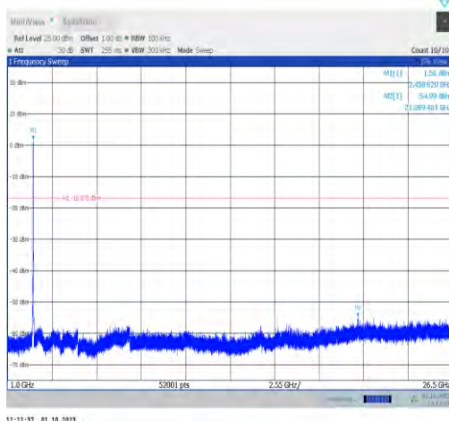
11n20MIMO-Ant9-2457-1000~26500-PASS
