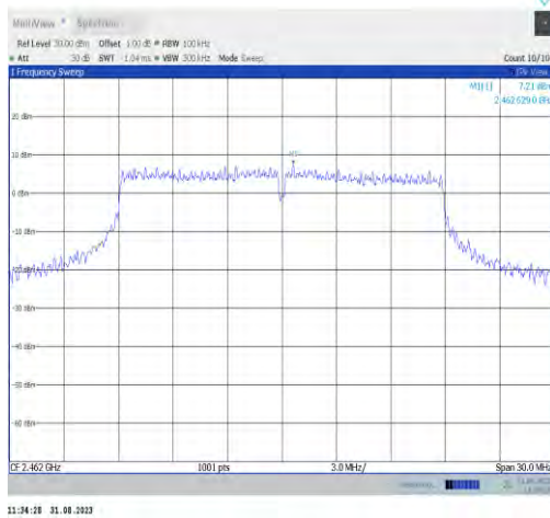
11n20MIMO-Ant9-2462-0~Reference-PASS
