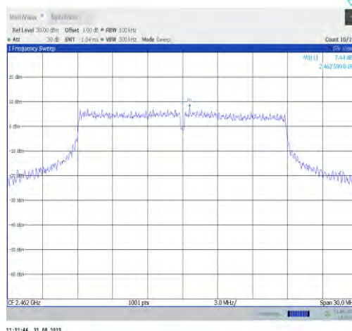
11n20MIMO-Ant7-2462-0~Reference-PASS
