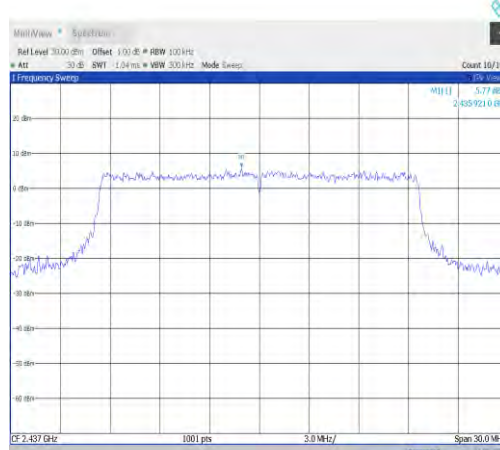
11ax20MIMO-Ant7-2437-0~Reference-PASS
