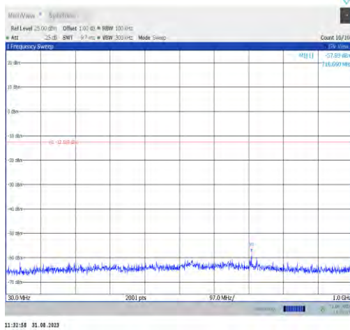
11n20MIMO-Ant7-2462-30~1000-PASS
