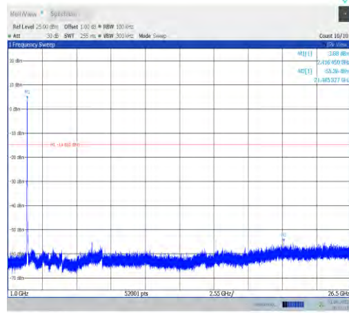
11ax20MIMO-Ant7-2412-1000~26500-PASS
