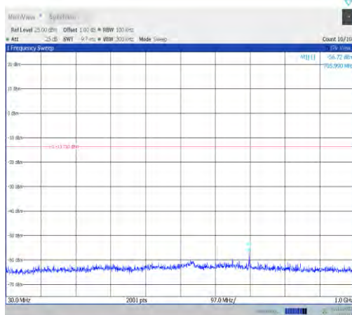
11ax20MIMO-Ant7-2422-30~1000-PASS
