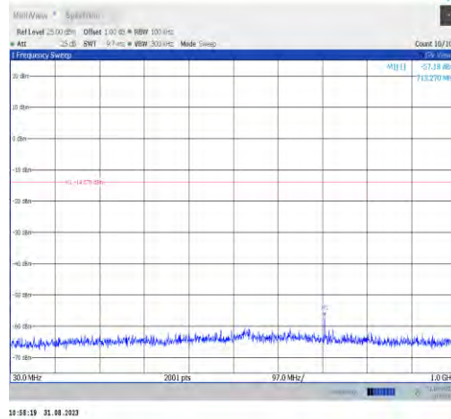
11n20MIMO-Ant7-2412-30~1000-PASS
