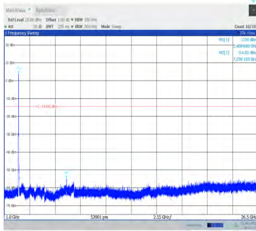
11ax20MIMO-Ant9-2412-1000~26500-PASS
