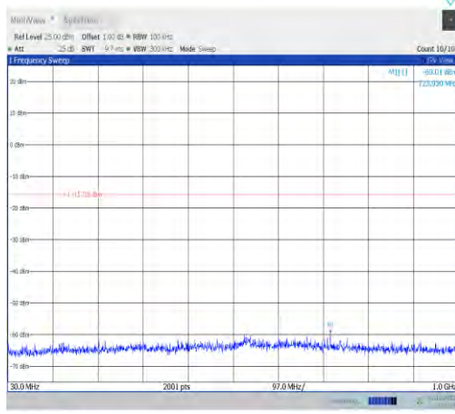
11ax20MIMO-Ant7-2457-30~1000-PASS
