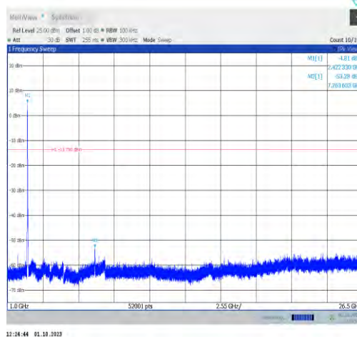
11ax20MIMO-Ant7-2422-1000~26500-PASS
