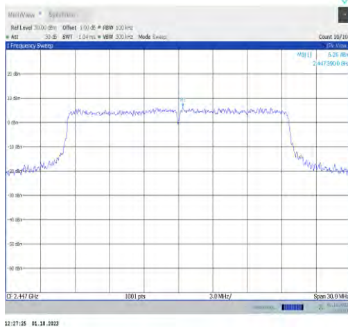
11ax20MIMO-Ant9-2447-0~Reference-PASS
