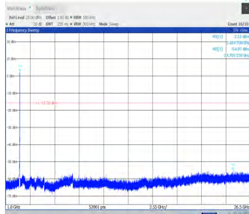
11ax20MIMO-Ant7-2452-1000~26500-PASS
