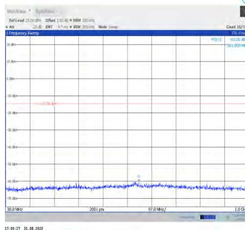
11ax20MIMO-Ant9-2437-30~1000-PASS
