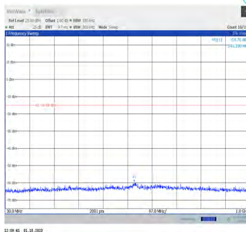
11n20MIMO-Ant9-2452-30~1000-PASS
