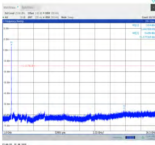
11ax20MIMO-Ant9-2437-1000~26500-PASS
