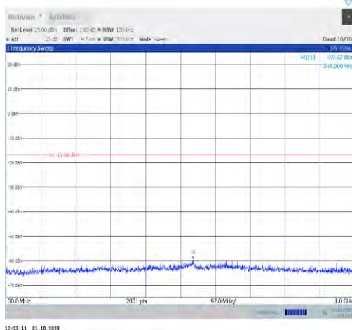
11n20MIMO-Ant7-2457-30~1000-PASS
