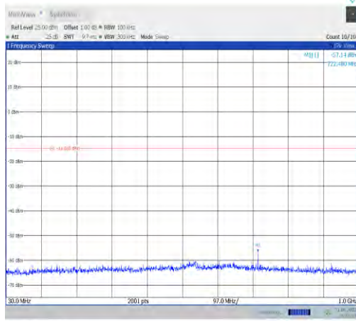
11ax20MIMO-Ant7-2412-30~1000-PASS
