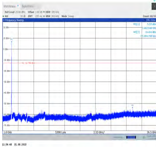
11n20MIMO-Ant9-2462-1000~26500-PASS
