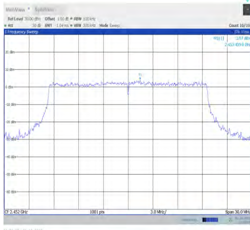
11ax20MIMO-Ant9-2452-0~Reference-PASS
