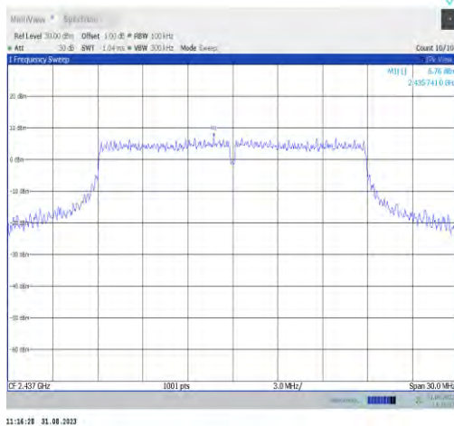
11n20MIMO-Ant9-2437-0~Reference-PASS
