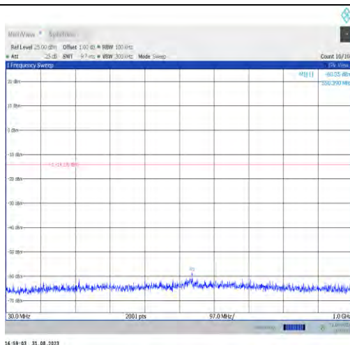
11ax20MIMO-Ant7-2437-30~1000-PASS
