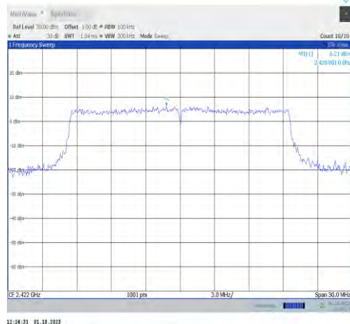
11ax20MIMO-Ant7-2422-0~Reference-PASS
