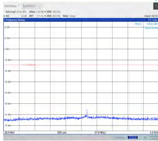
11ax20MIMO-Ant9-2412-30~1000-PASS
