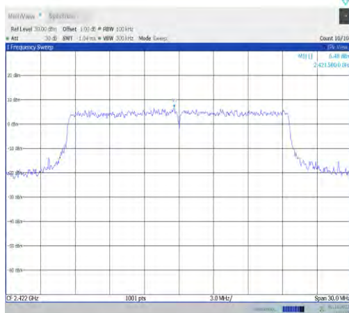
11ax20MIMO-Ant9-2422-0~Reference-PASS
