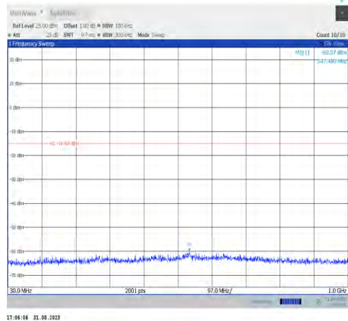
11ax20MIMO-Ant9-2462-30~1000-PASS
