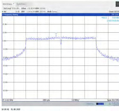
11n20MIMO-Ant7-2412-0~Reference-PASS
