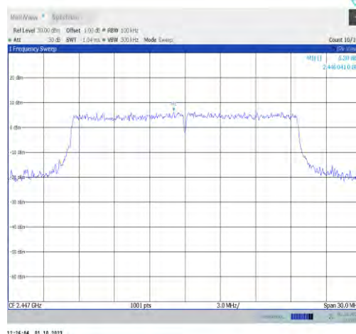
11ax20MIMO-Ant7-2447-0~Reference-PASS
