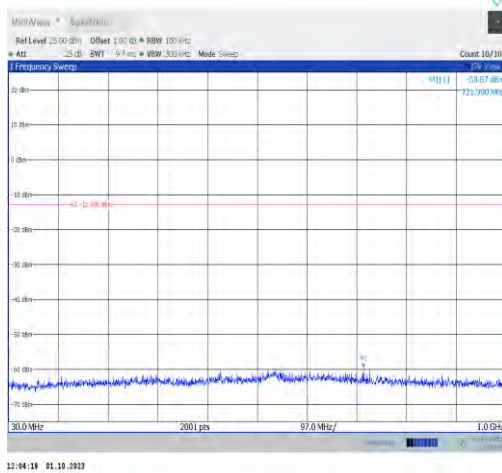
11n20MIMO-Ant7-2447-30~1000-PASS
