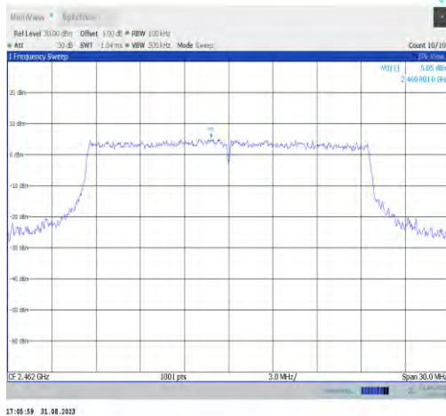
11ax20MIMO-Ant9-2462-0~Reference-PASS
