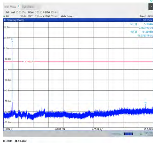
11n20MIMO-Ant7-2462-1000~26500-PASS
