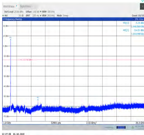
11ax20MIMO-Ant9-2447-1000~26500-PASS
