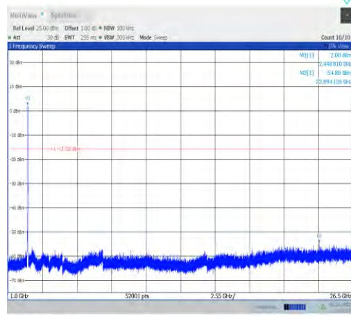
11ax20MIMO-Ant7-2457-1000~26500-PASS
