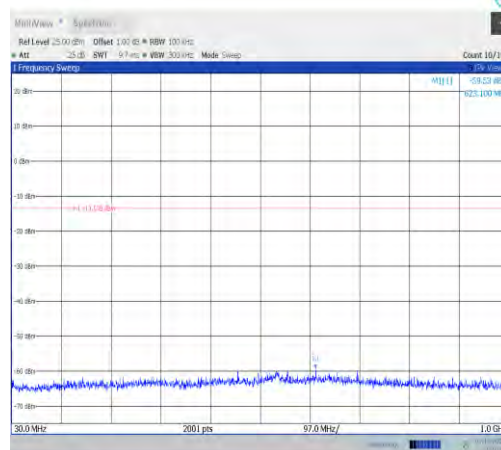
11n20MIMO-Ant9-2417-30~1000-PASS
