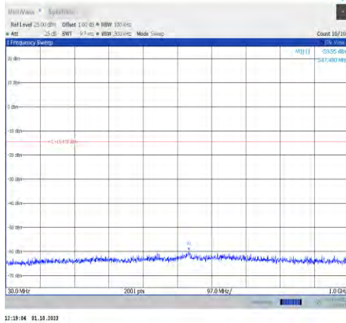
11ax20MIMO-Ant7-2417-30~1000-PASS
