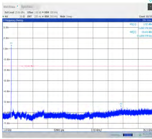
11ax20MIMO-Ant9-2457-1000~26500-PASS
