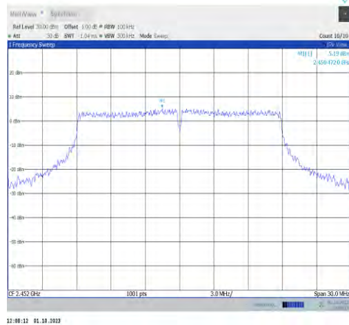
11n20MIMO-Ant7-2452-0~Reference-PASS
