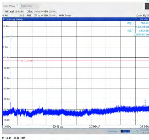
11n20MIMO-Ant9-2437-1000~26500-PASS
