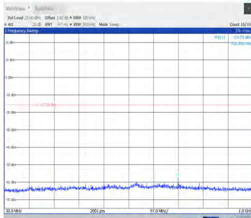
11ax20MIMO-Ant7-2452-30~1000-PASS
