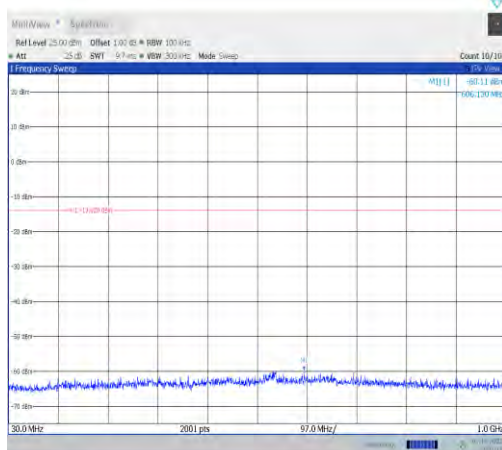
11n20MIMO-Ant7-2417-30~1000-PASS
