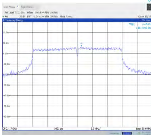
11n20MIMO-Ant9-2417-0~Reference-PASS
