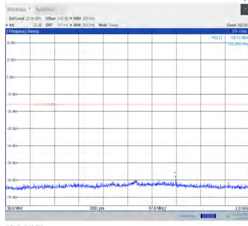
11ax20MIMO-Ant9-2452-30~1000-PASS
