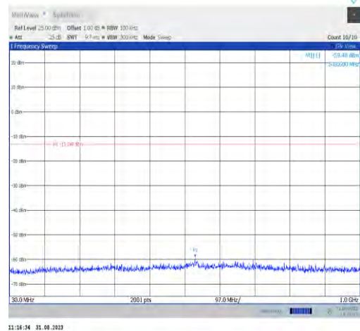
11n20MIMO-Ant9-2437-30~1000-PASS
