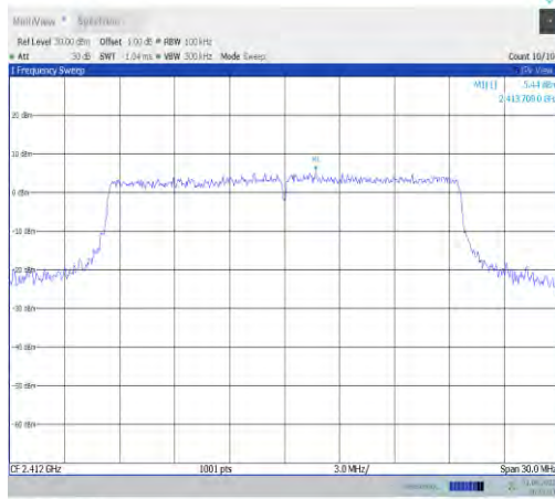
11ax20MIMO-Ant9-2412-0~Reference-PASS
