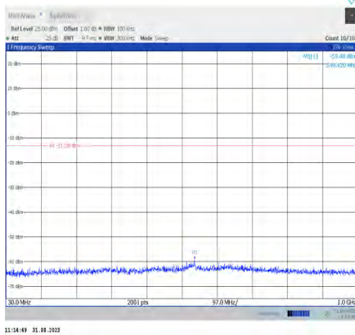
11n20MIMO-Ant7-2437-30~1000-PASS
