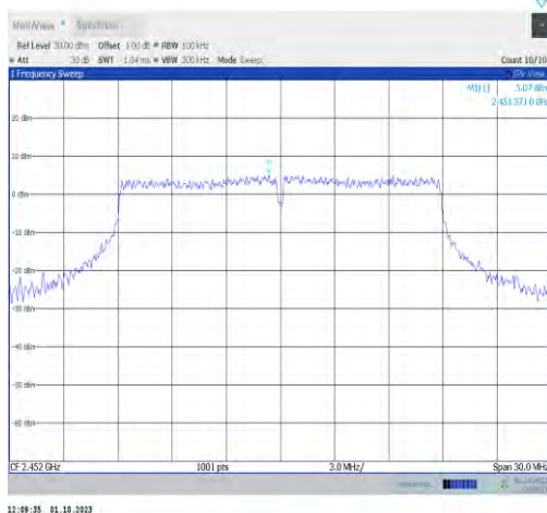
11n20MIMO-Ant9-2452-0~Reference-PASS
