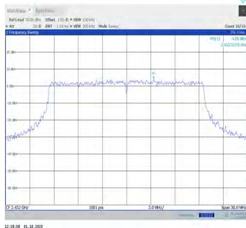
11ax20MIMO-Ant7-2452-0~Reference-PASS
