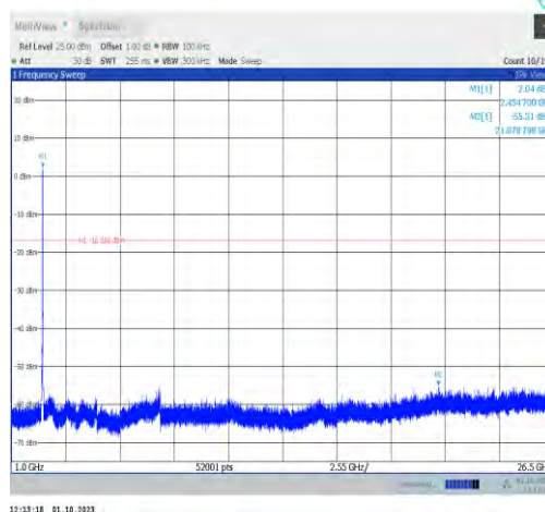
11n20MIMO-Ant7-2457-1000~26500-PASS
