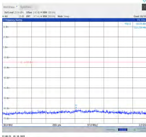
11n20MIMO-Ant7-2452-30~1000-PASS
