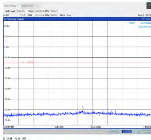
11ax20MIMO-Ant9-2417-30~1000-PASS
