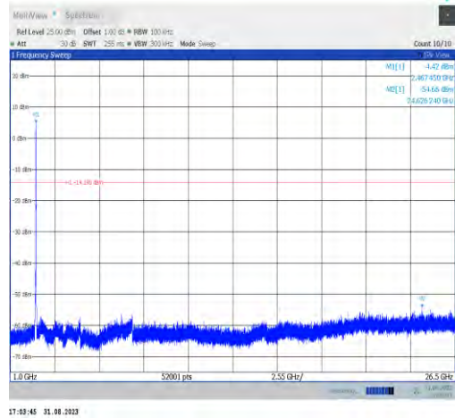
11ax20MIMO-Ant7-2462-1000~26500-PASS
