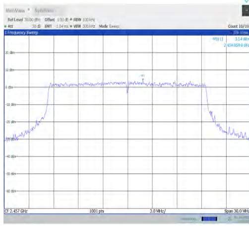
11ax20MIMO-Ant9-2457-0~Reference-PASS
