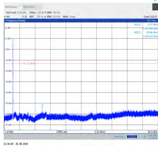
11n20MIMO-Ant7-2437-1000~26500-PASS
