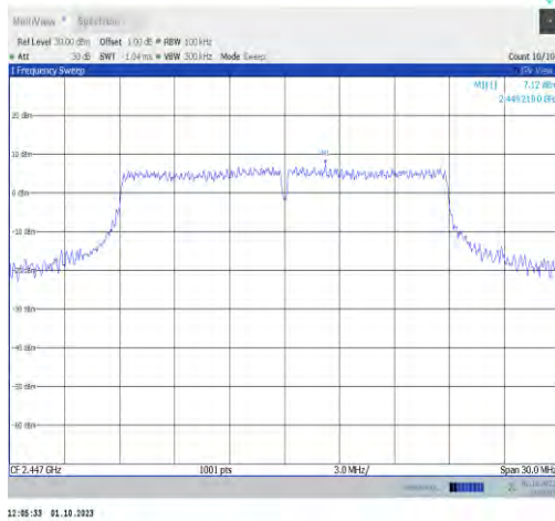
11n20MIMO-Ant9-2447-0~Reference-PASS
