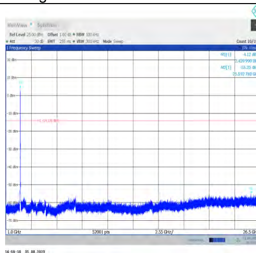
11ax20MIMO-Ant7-2437-1000~26500-PASS
