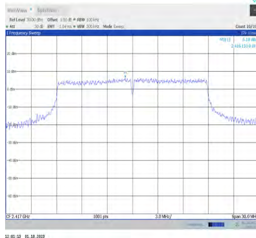
11n20MIMO-Ant7-2417-0~Reference-PASS
