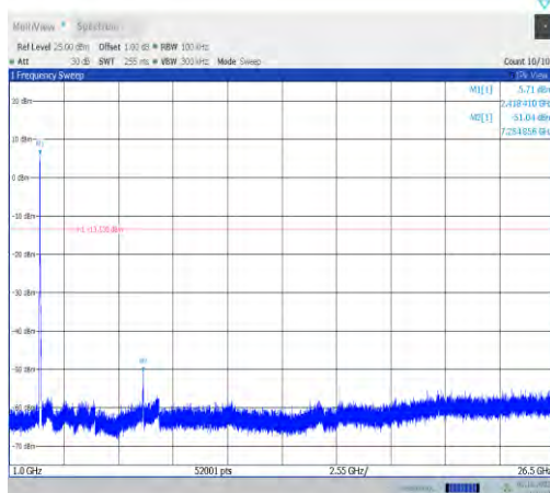
11n20MIMO-Ant9-2417-1000~26500-PASS
