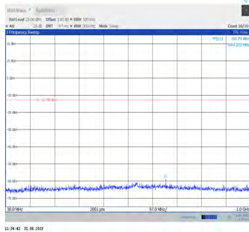
11n20MIMO-Ant9-2462-30~1000-PASS
