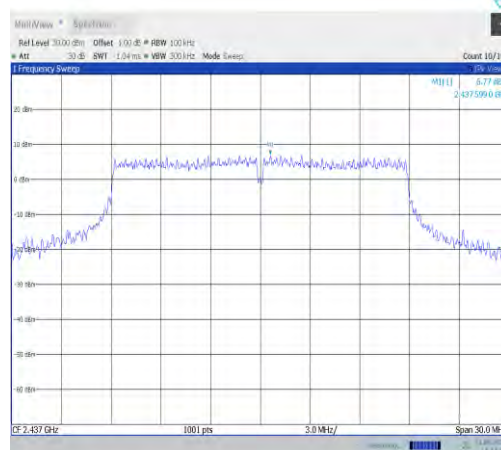
11n20MIMO-Ant7-2437-0~Reference-PASS
