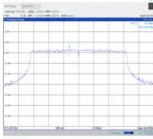
11ax20MIMO-Ant7-2457-0~Reference-PASS
