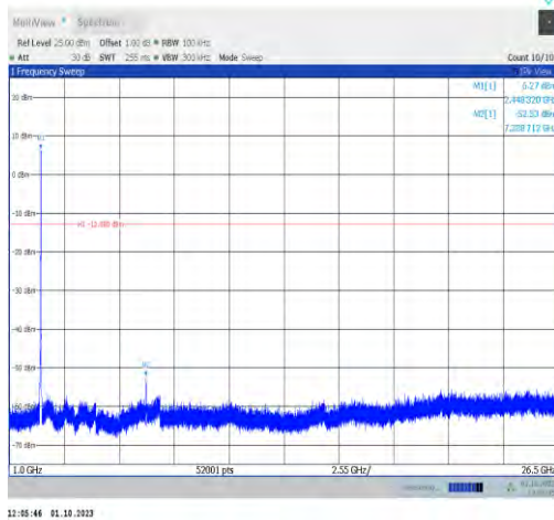
11n20MIMO-Ant9-2447-1000~26500-PASS
