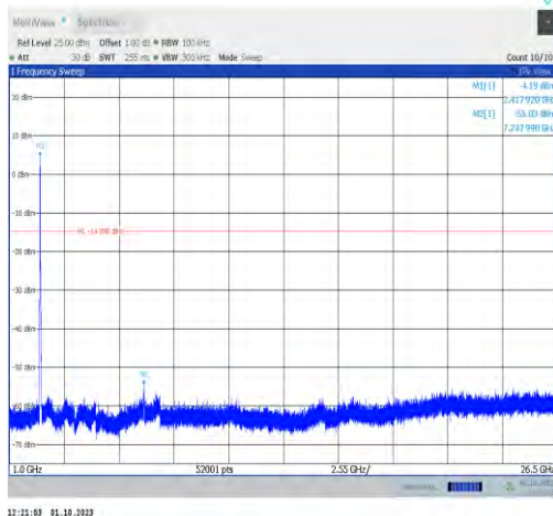
11ax20MIMO-Ant9-2417-1000~26500-PASS
