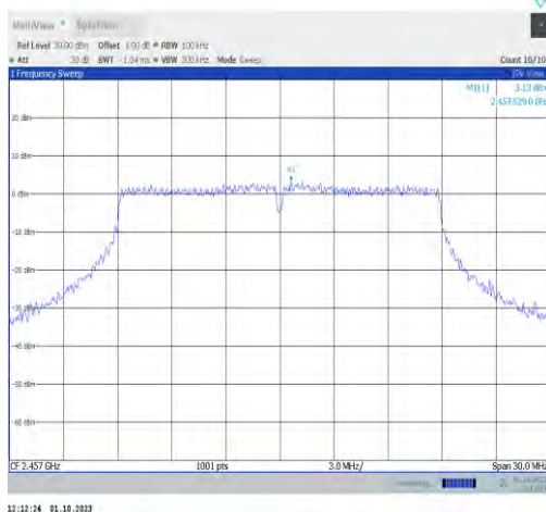
11n20MIMO-Ant9-2457-0~Reference-PASS
