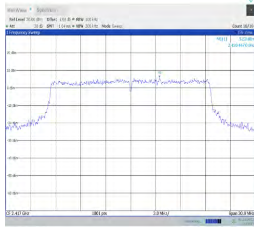
11ax20MIMO-Ant7-2417-0~Reference-PASS
