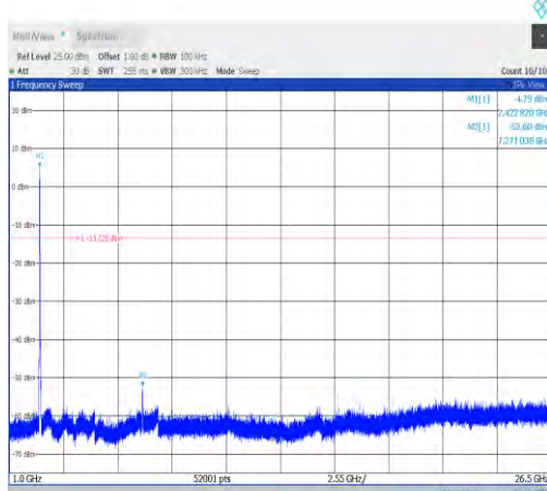
11ax20MIMO-Ant9-2422-1000~26500-PASS
