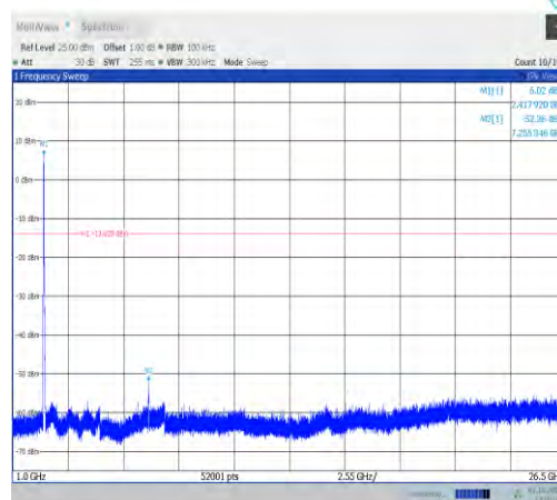
11n20MIMO-Ant7-2417-1000~26500-PASS
