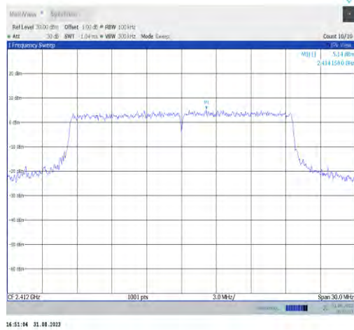
11ax20MIMO-Ant7-2412-0~Reference-PASS
