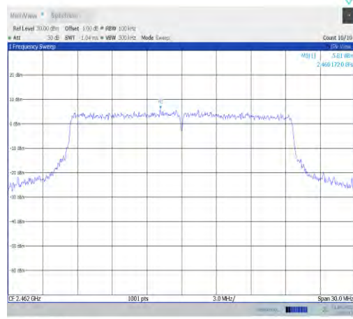
11ax20MIMO-Ant7-2462-0~Reference-PASS
