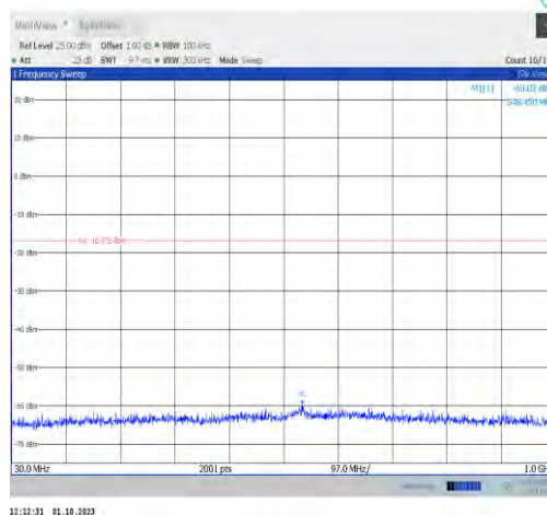
11n20MIMO-Ant9-2457-30~1000-PASS
