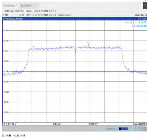
11ax20MIMO-Ant9-2417-0~Reference-PASS
