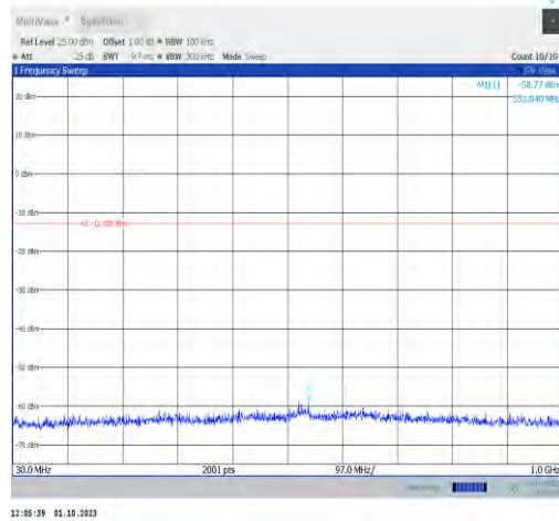
11n20MIMO-Ant9-2447-30~1000-PASS
