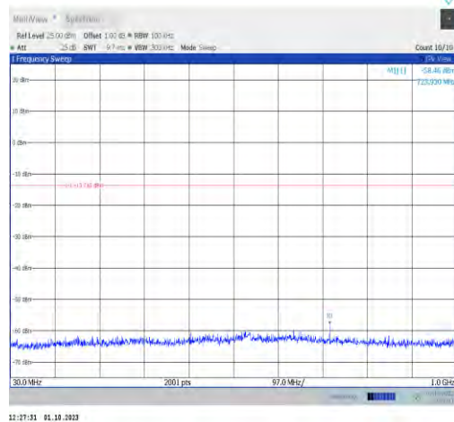
11ax20MIMO-Ant9-2447-30~1000-PASS
