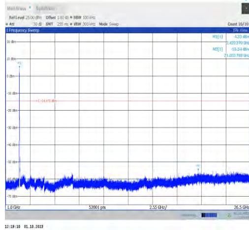
11ax20MIMO-Ant7-2417-1000~26500-PASS
