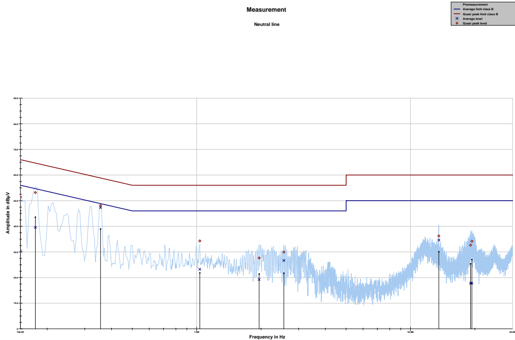
Plot 6: M30: 150 kHz to 30 MHz, neutral line
