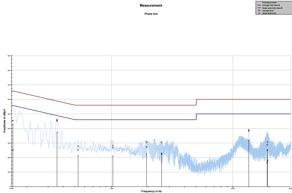
Plot 5: M30: 150 kHz to 30 MHz, phase line
