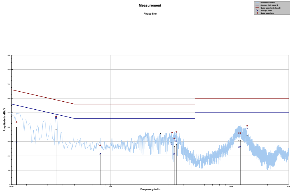
Plot 3: M18: 150 kHz to 30 MHz, phase line
