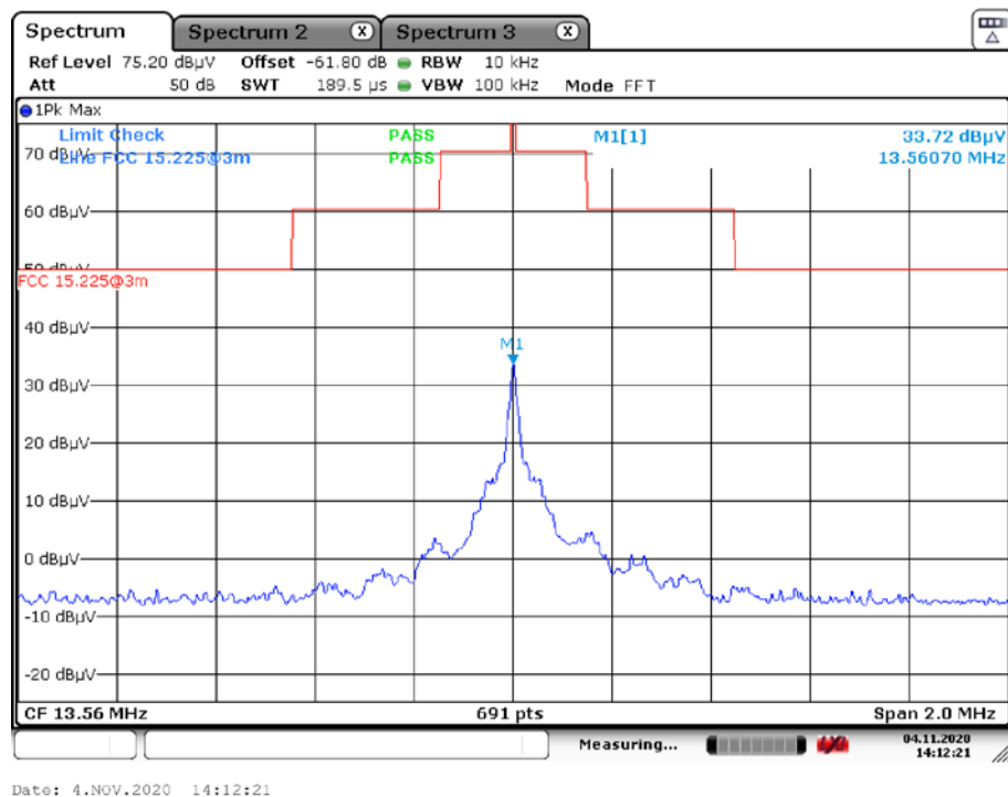
Plot 8: M30: Spectrum mask (the limits are recalculated according to the ANSI C63.10-2013 sub clause 6.4)
