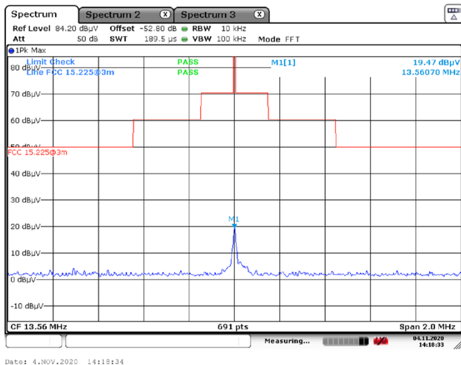
Plot 2: M12: Spectrum mask (the limits are recalculated according to the ANSI C63.10-2013 sub clause 6.4)
