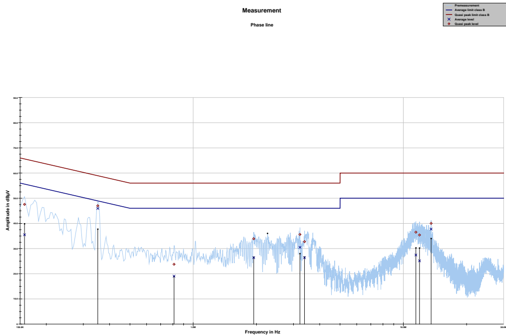
Plot 1: M12: 150 kHz to 30 MHz, phase line
