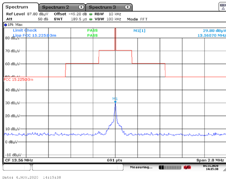
Plot 5: M18: Spectrum mask (the limits are recalculated according to the ANSI C63.10-2013 sub clause 6.4)
