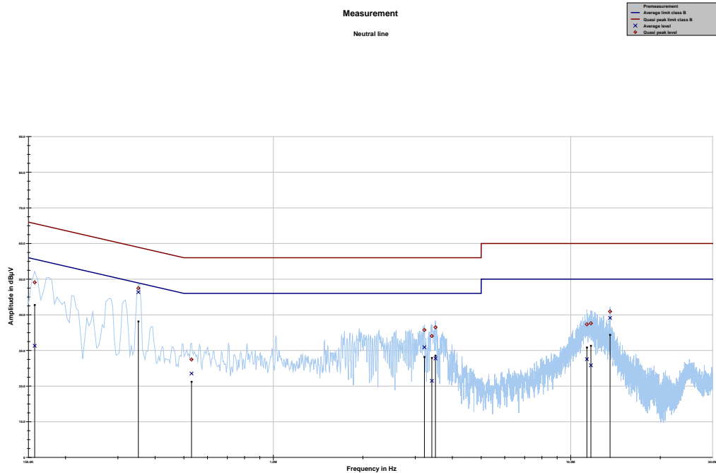
Plot 4: M18: 150 kHz to 30 MHz, neutral line
