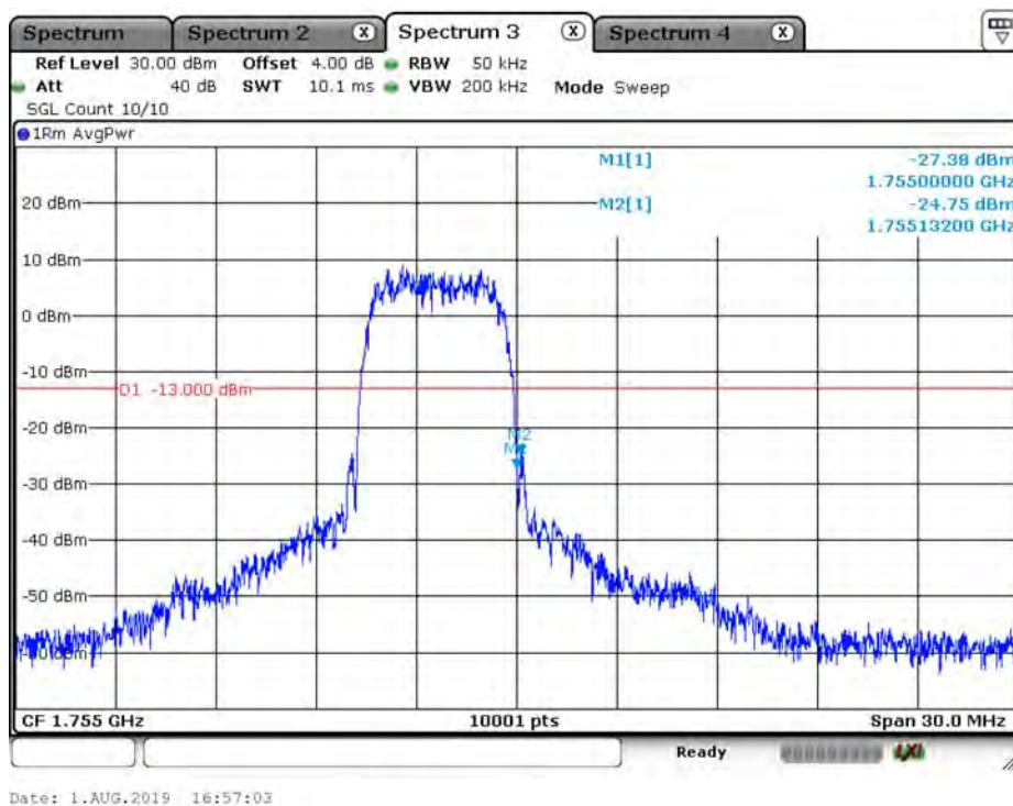
WCDMA_Band4_RMC_1752.6
