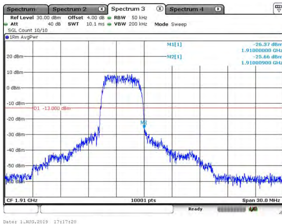
WCDMA_Band2_RMC_1907.6
