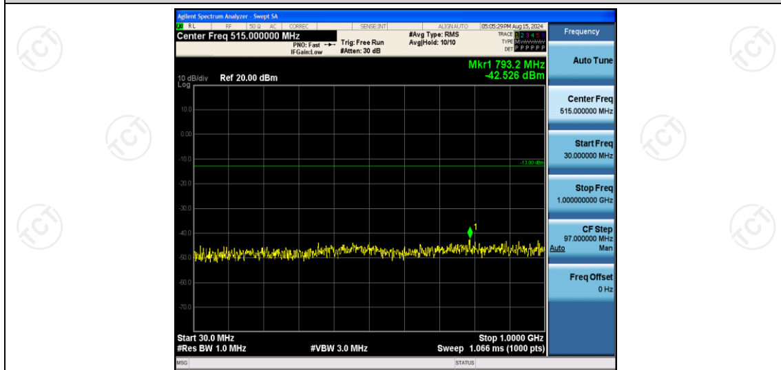
Band66-1.4MHz-QPSK-132322-1RB#0-Range1:30~1000MHz
