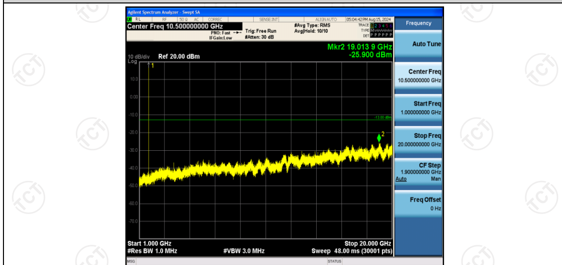
Band66-1.4MHz-QPSK-131979-1RB#0-Range2:1000~20000MHz
