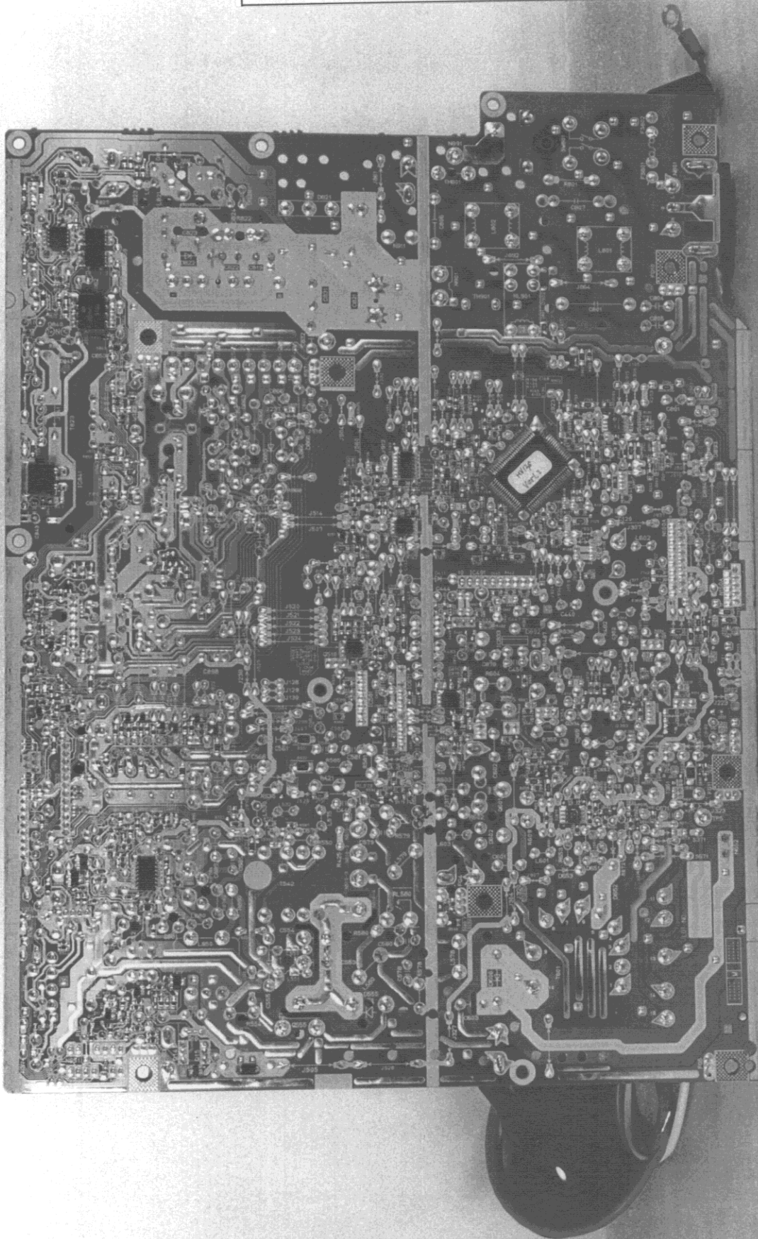
Photo 8. Main and Power Supply PWB (Solder side) of VCDTS21492-4*
