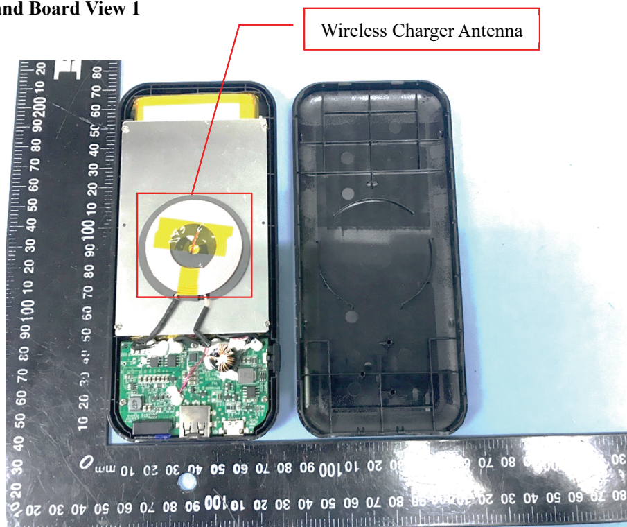
EUT Housing and Board View 1
