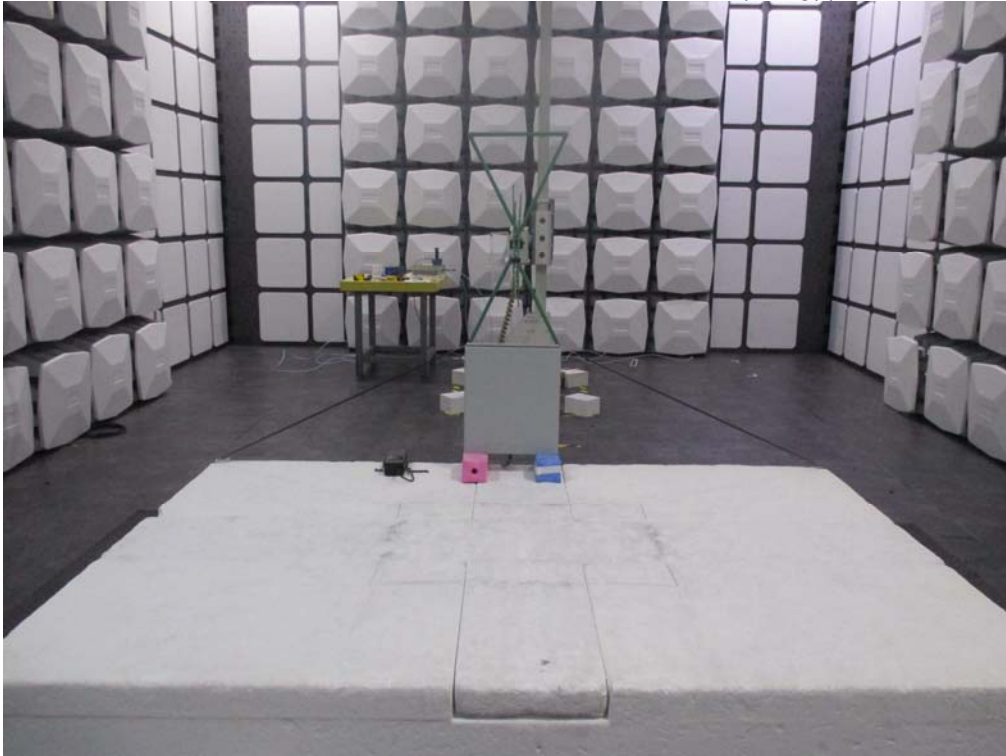
Description: Back View of Radiated Emission Test Setup (Bilog)(ADP-65JH HB)
