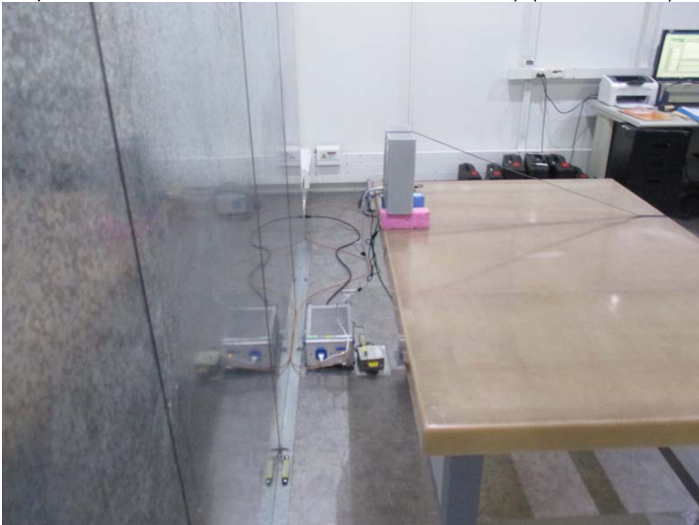
Description: Back View of Conducted Emission Test Setup (ADP-65JH HB)
