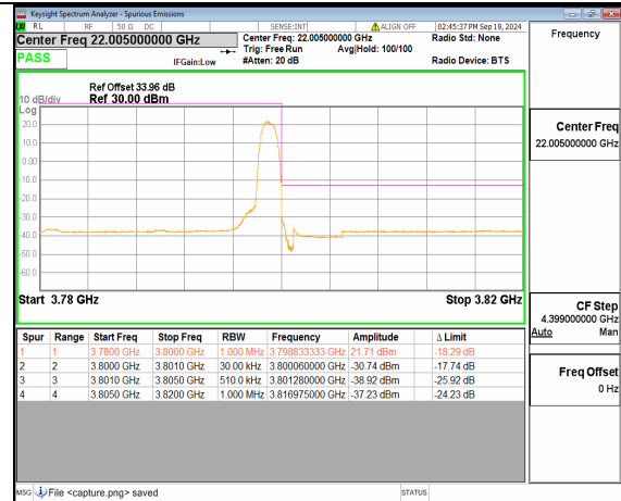
n78(3700-3800MHz) 20M DFT-s-OFDM BPSK Edge_1RB_Right High
