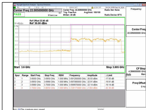
n78(3700-3800MHz) 100M DFT-s-OFDM BPSK Outer_Full Low
