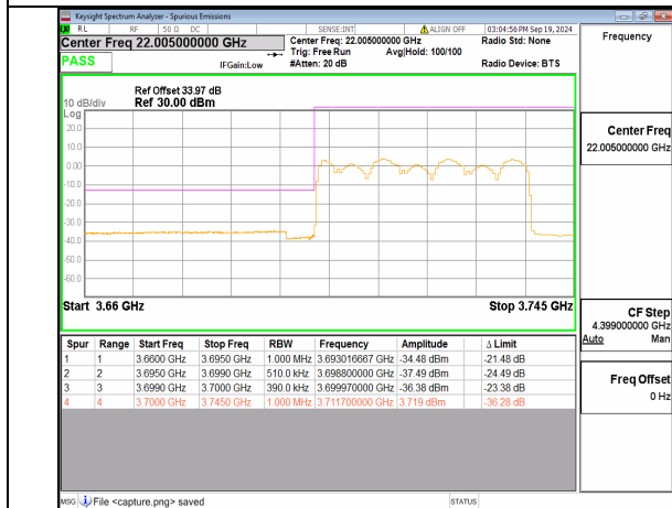
n78(3700-3800MHz) 40M DFT-s-OFDM QPSK Outer_Full Low
