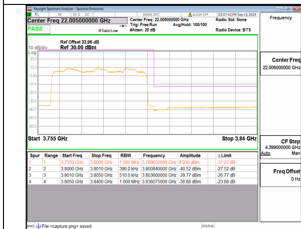
n78(3700-3800MHz) 40M DFT-s-OFDM BPSK Outer_Full High
