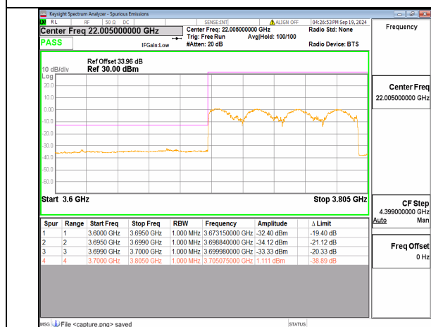
n78(3700-3800MHz) 100M DFT-s-OFDM QPSK Outer_Full Low
