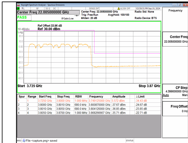
n78(3700-3800MHz) 70M DFT-s-OFDM QPSK Outer_Full High
