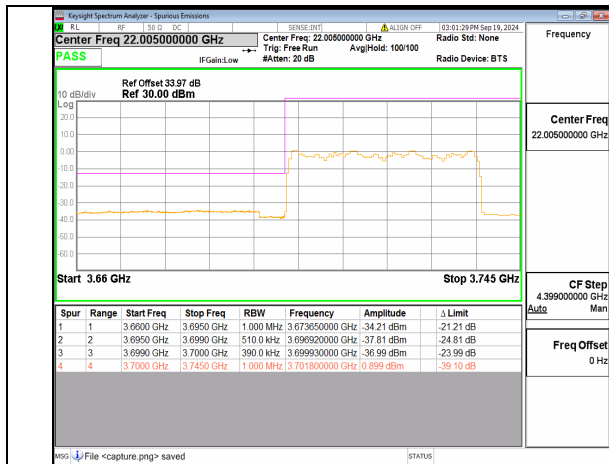
n78(3700-3800MHz) 40M DFT-s-OFDM BPSK Outer_Full Low
