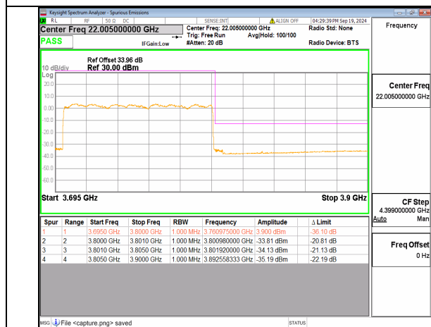
n78(3700-3800MHz) 100M DFT-s-OFDM BPSK Outer_Full High
