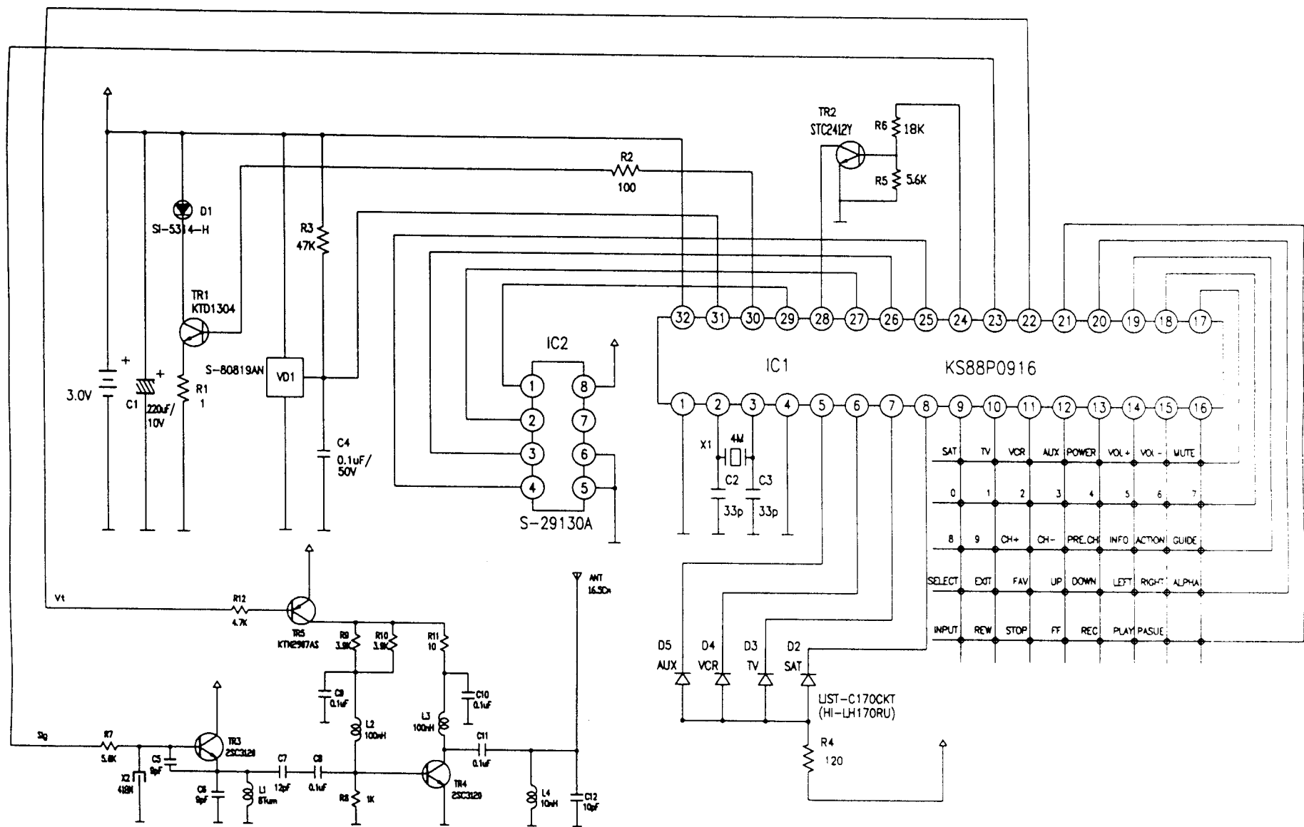
CIRCUIT DIAGRAM
