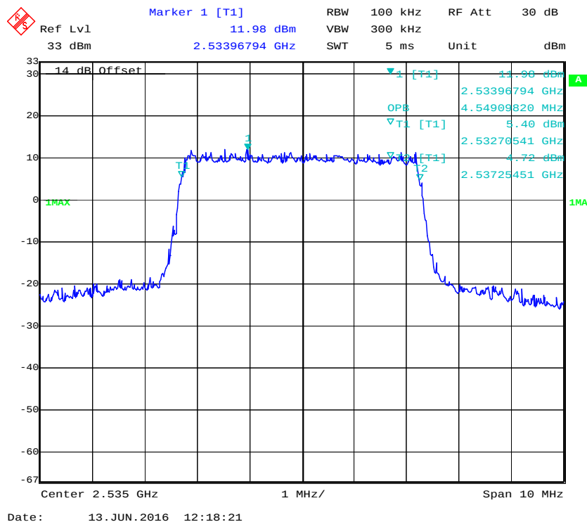
QPSK (5.0 MHz) Occupied Bandwidth, Middle channel
