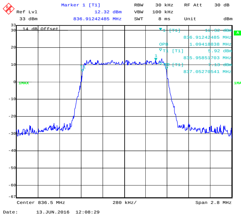
QPSK (1.4 MHz) Occupied Bandwidth Middle channel
