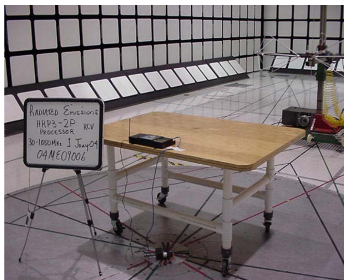
Rear – 30-1000MHz - Transmitter
