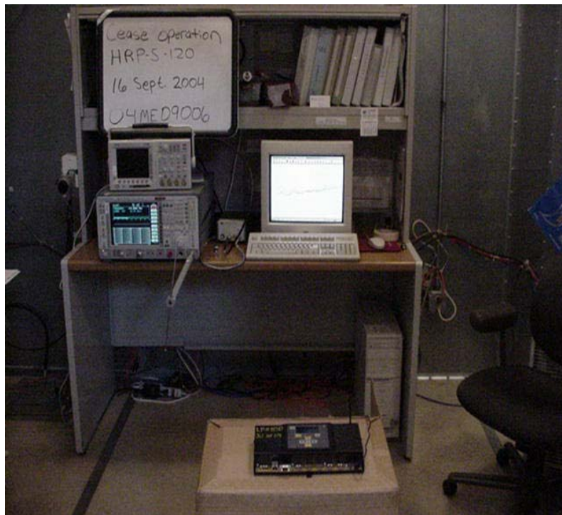
Cease Operation Test Set-Up
