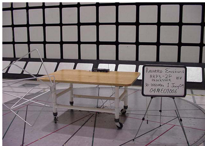
Front – 30-1000MHz - Transmitter
