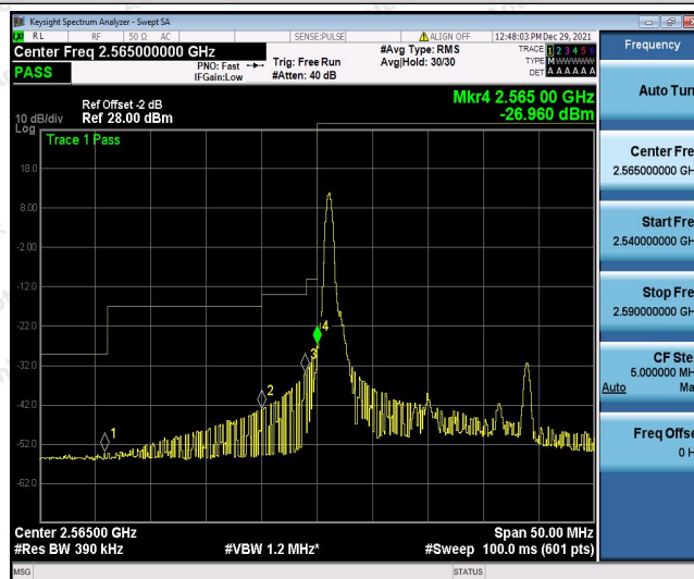
Band41-20MHz-16QAM-40440-1RB#99
