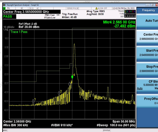
Band41-15MHz-QPSK-40415-1RB#74
