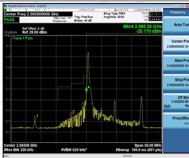
Band41-10MHz-16QAM-40390-1RB#49
