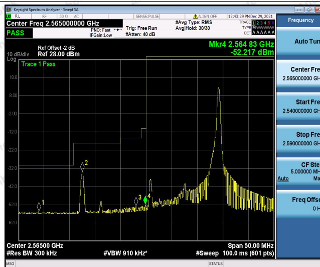
Band41-15MHz-QPSK-40415-75RB#0
