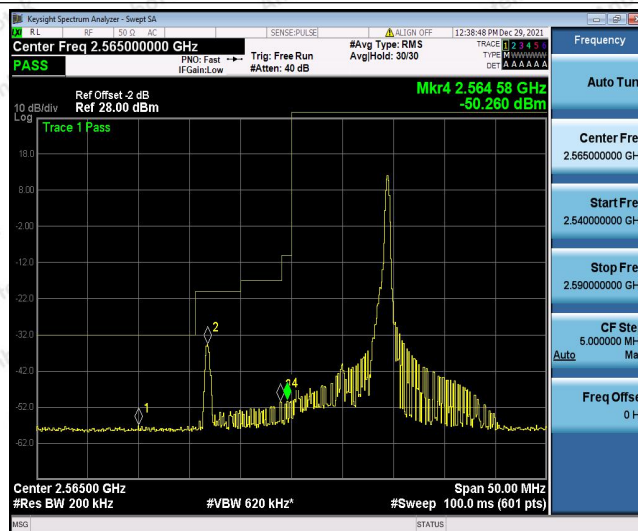
Band41-10MHz-QPSK-40390-50RB#0
