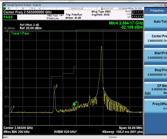
Band41-10MHz-16QAM-40390-50RB#0
