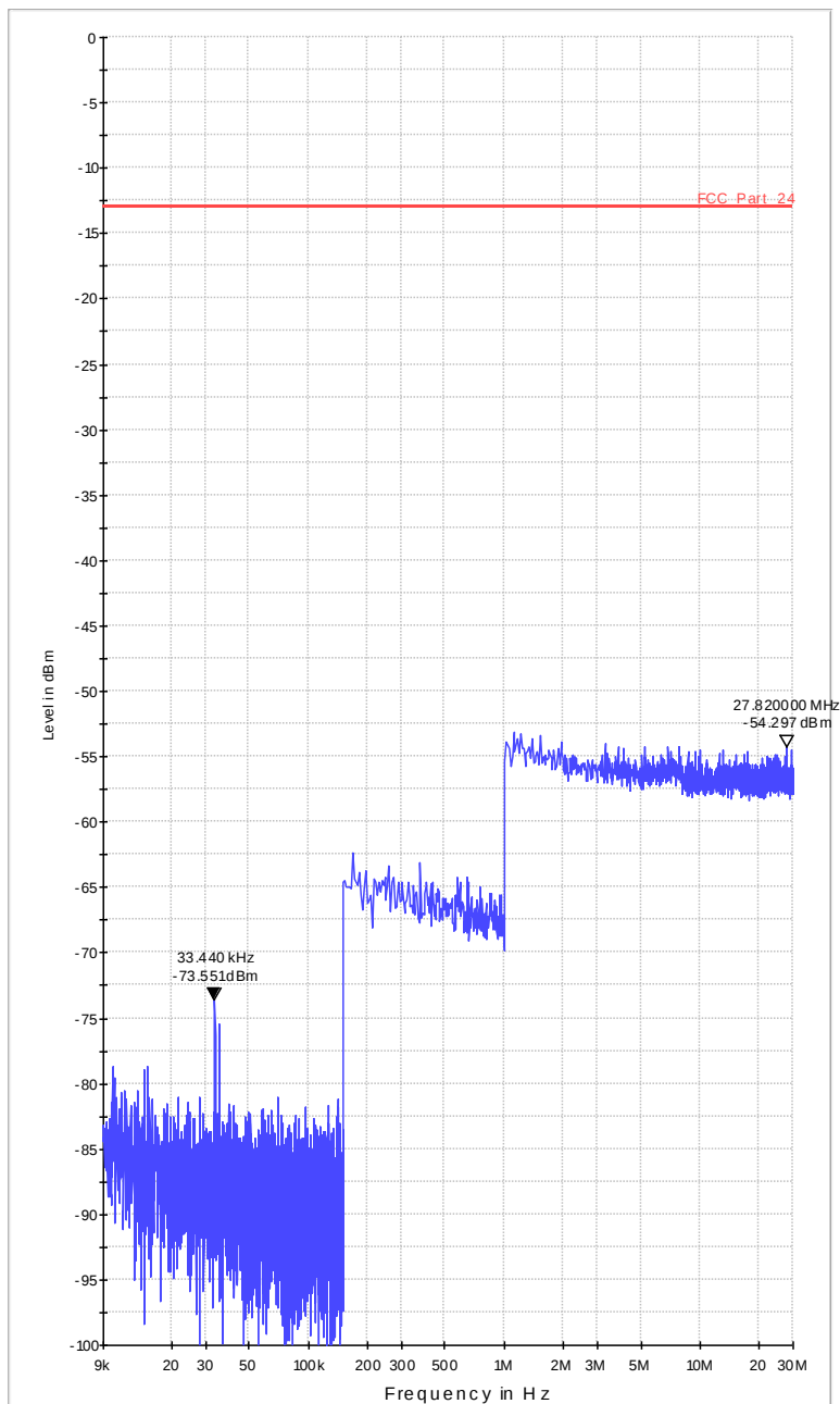
Diagram 36.05_TX_Ch9538_Sweep1
