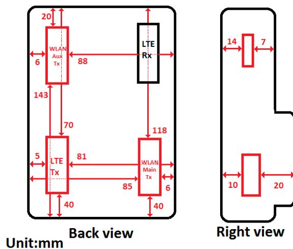
Fig.13 Antenna position of EUT (Back view &amp; Right view )
