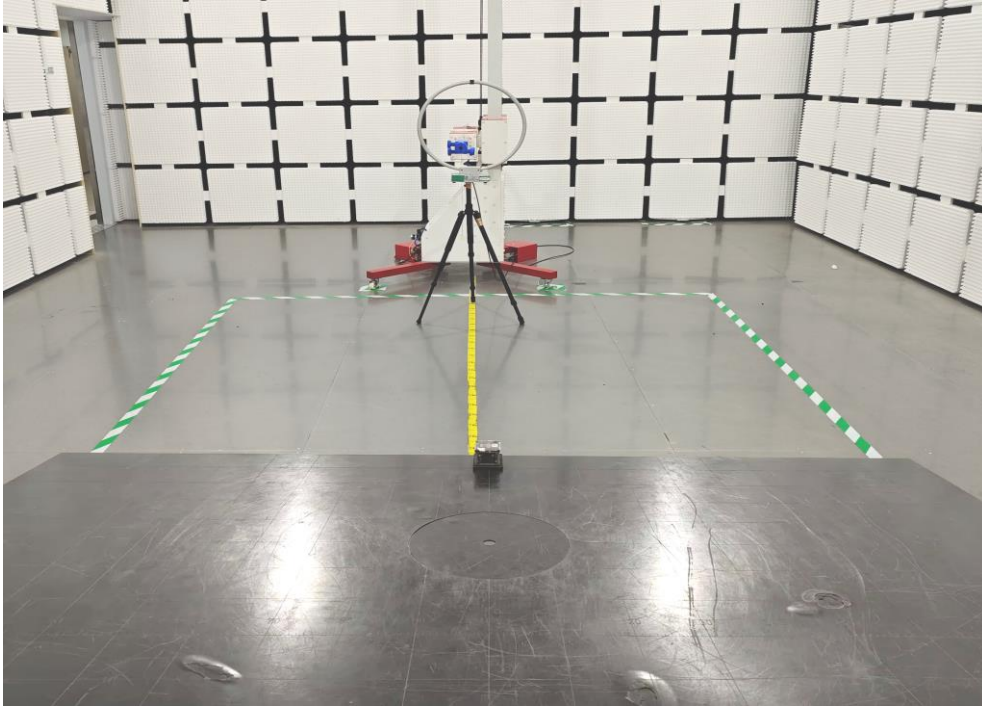
Spurious Radiation Emissions Test (<30M)
