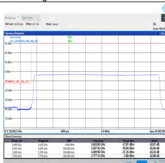
1-N77-3700-3980-30-50-L-3-DFT-PI2BPSK-Outer _Full-128@0-Ant1-1--PASS-see graph
