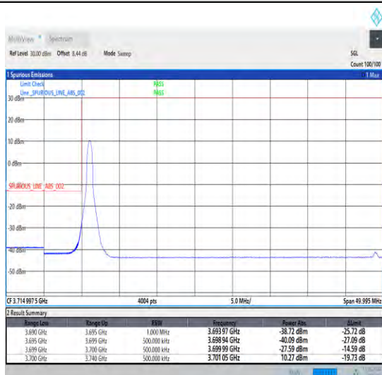
1-N77-3700-3980-30-40-L-4-CP-QPSK-Edge_1RB_Lef t-1@0-Ant1-1--PASS-see graph
