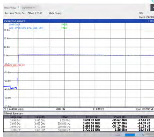
1-N77-3700-3980-30-100-L-6-CP-QPSK-Outer_Full-273@0-Ant1-1--PASS-see graph
