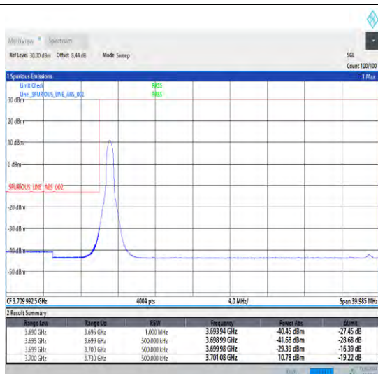
1-N77-3700-3980-30-30-L-1-DFT-PI2BPSK-Edge_1RB _Left-1@0-Ant1-1--PASS-see graph
