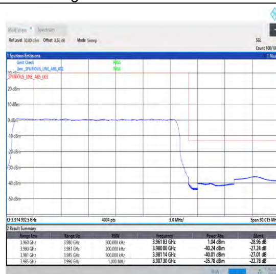
1-N77-3700-3980-30-20-H-3-DFT-PI2BPSK-Outer_Full-50@0-Ant1-1--PASS-see graph
