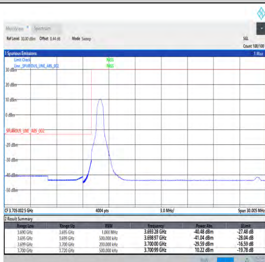
1-N77-3700-3980-30-20-L-4-CP-QPSK-Edge_1RB_Lef t-1@0-Ant1-1--PASS-see graph
