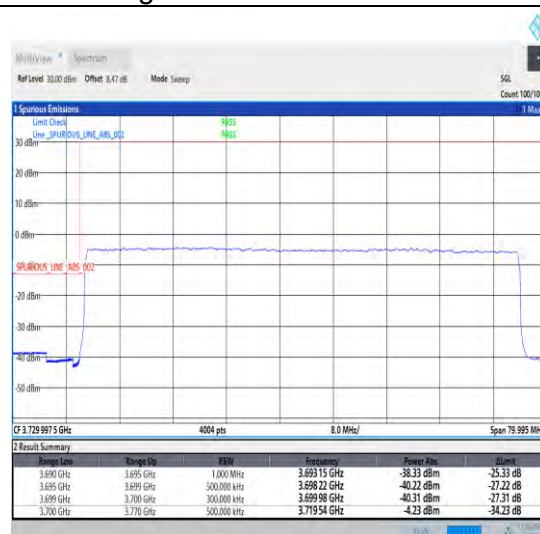
1-N77-3700-3980-30-70-L-3-DFT-PI2BPSK-Outer _Full-180@0-Ant1-1--PASS-see graph
