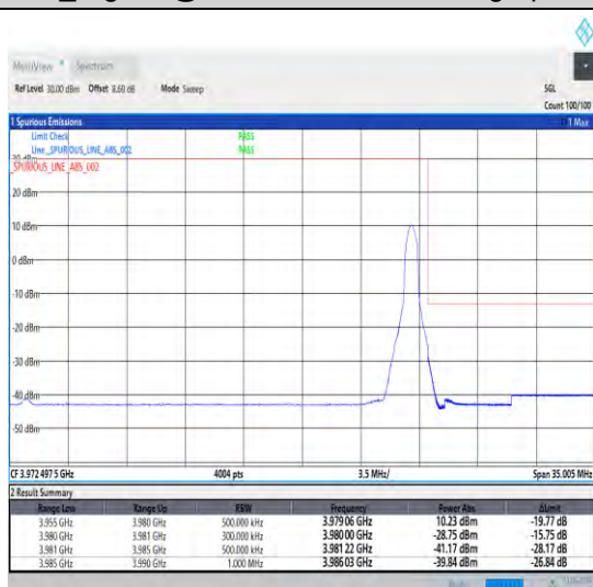
1-N77-3700-3980-30-25-H-5-CP-QPSK-Edge_1RB_Right-1@64-Ant1-1--PASS-see graph
