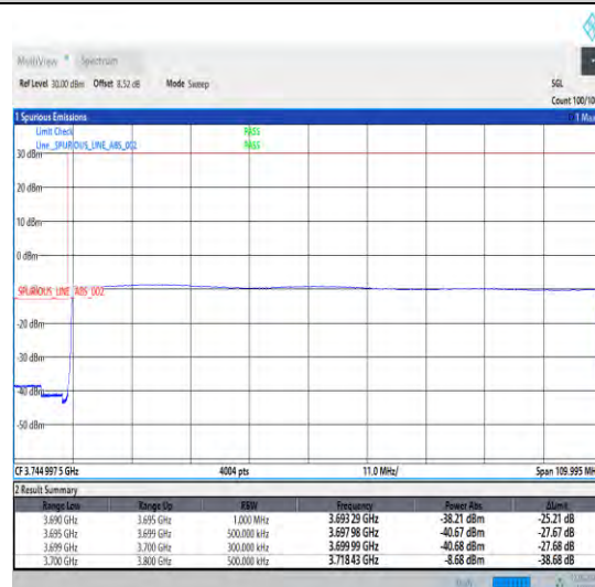
1-N77-3700-3980-30-100-L-6-CP-QPSK-Outer_Full-273@0-Ant1-1--PASS-see graph
