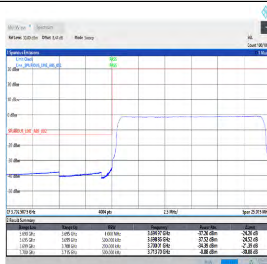
1-N77-3700-3980-30-15-L-6-CP-QPSK-Outer_Full -38@0-Ant1-1--PASS-see graph
