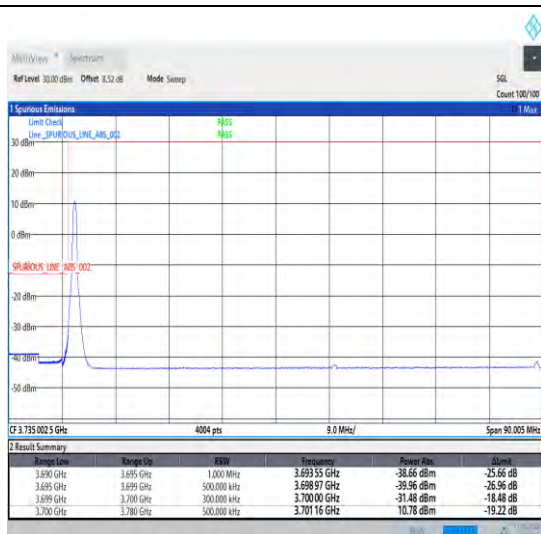
1-N77-3700-3980-30-80-L-1-DFT-PI2BPSK-Edge_1RB _Left-1@0-Ant1-1--PASS-see graph
