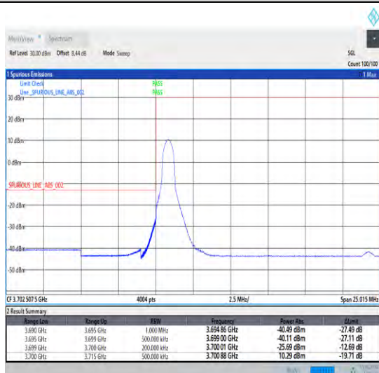
1-N77-3700-3980-30-15-L-4-CP-QPSK-Edge_1RB_Lef t-1@0-Ant1-1--PASS-see graph
