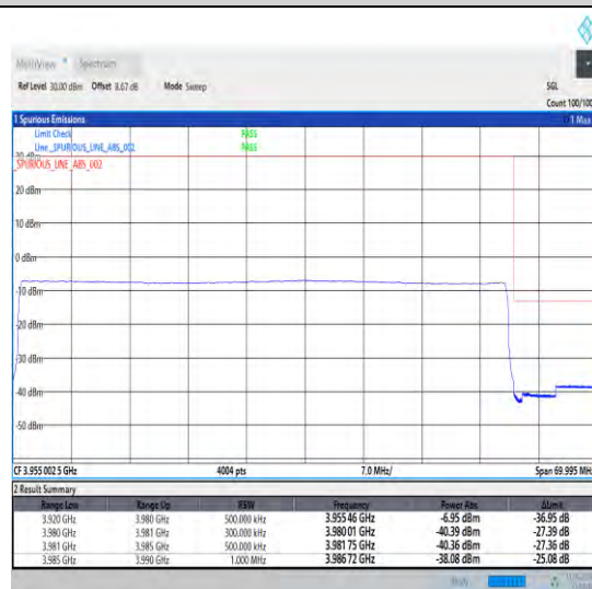
1-N77-3700-3980-30-60-H-6-CP-QPSK-Outer_Full -162@0-Ant1-1--PASS-see graph
