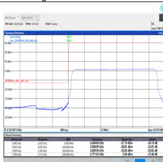
1-N77-3700-3980-30-15-L-3-DFT-PI2BPSK-Outer _Full-36@0-Ant1-1--PASS-see graph
