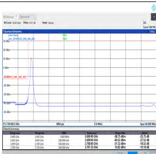
1-N77-3700-3980-30-50-L-1-DFT-PI2BPSK-Edge_1RB _Left-1@0-Ant1-1--PASS-see graph
