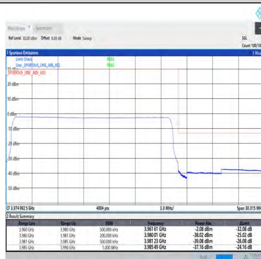
1-N77-3700-3980-30-20-H-6-CP-QPSK-Outer_Full-51@0-Ant1-1--PASS-see graph
