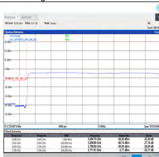
1-N77-3700-3980-30-60-L-3-DFT-PI2BPSK-Outer _Full-162@0-Ant1-1--PASS-see graph
