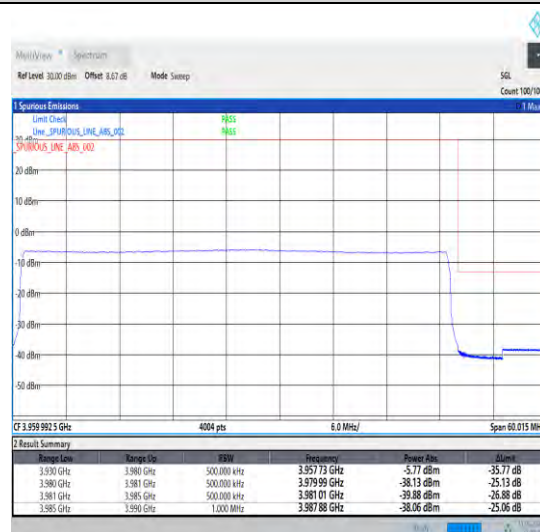
1-N77-3700-3980-30-50-H-6-CP-QPSK-Outer_Full -133@0-Ant1-1--PASS-see graph
