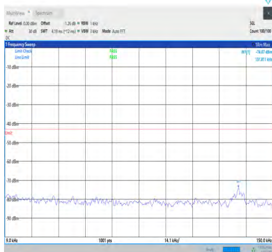
1-N77-3700-3980-30-100-H-1-DFT-QPSK-Edge_1R B_Left-1@0-0.009-0.15-Ant1-0.13--74.07--43-PASS
