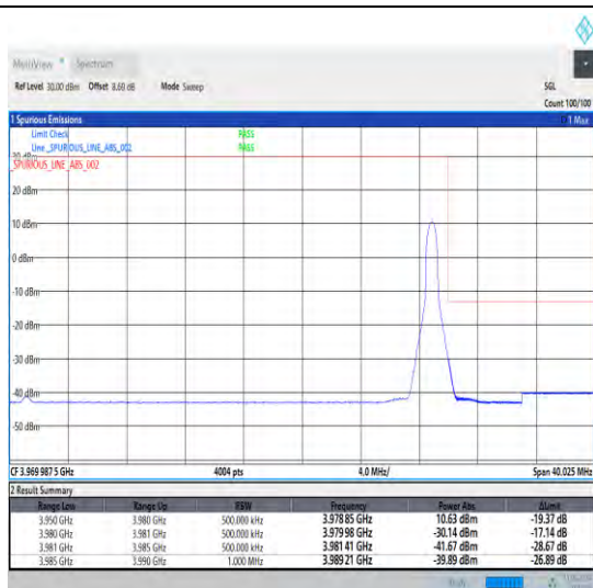
1-N77-3700-3980-30-30-H-2-DFT-PI2BPSK-Edge_1R_B_Right-1@77-Ant1-1--PASS-see graph
