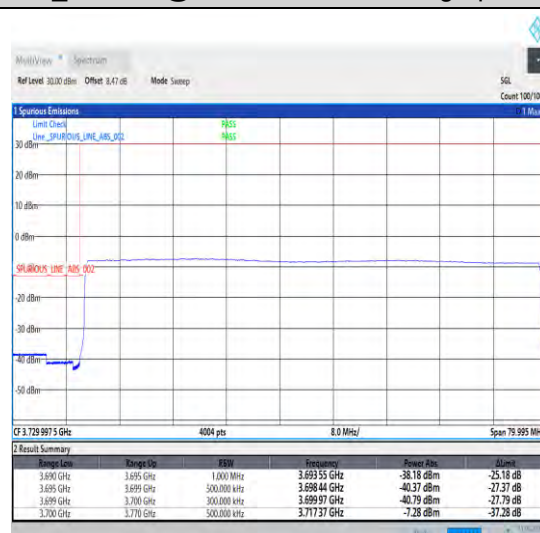
1-N77-3700-3980-30-70-L-6-CP-QPSK-Outer_Full -189@0-Ant1-1--PASS-see graph
