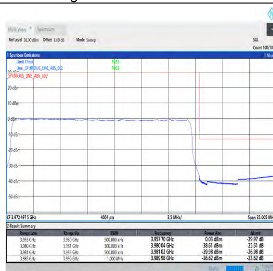
1-N77-3700-3980-30-25-H-3-DFT-PI2BPSK-Outer_Full-64@0-Ant1-1--PASS-see graph
