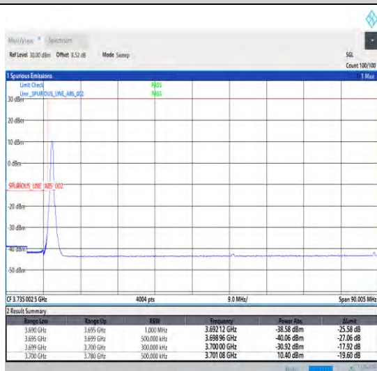
1-N77-3700-3980-30-80-L-4-CP-QPSK-Edge_1RB_Lef t-1@0-Ant1-1--PASS-see graph
