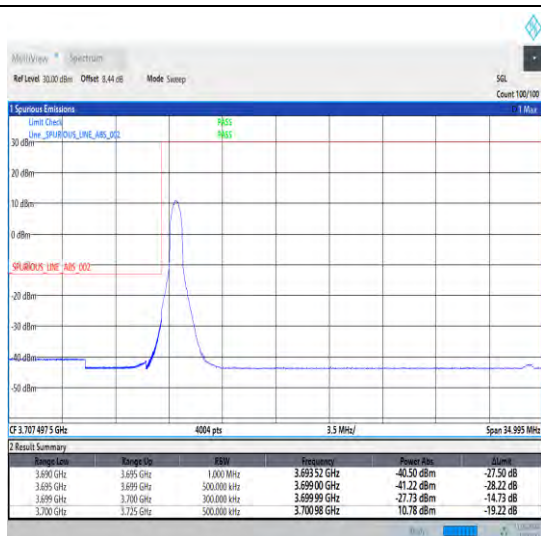
1-N77-3700-3980-30-25-L-1-DFT-PI2BPSK-Edge_1RB_Left-1@0-Ant1-1--PASS-see graph
