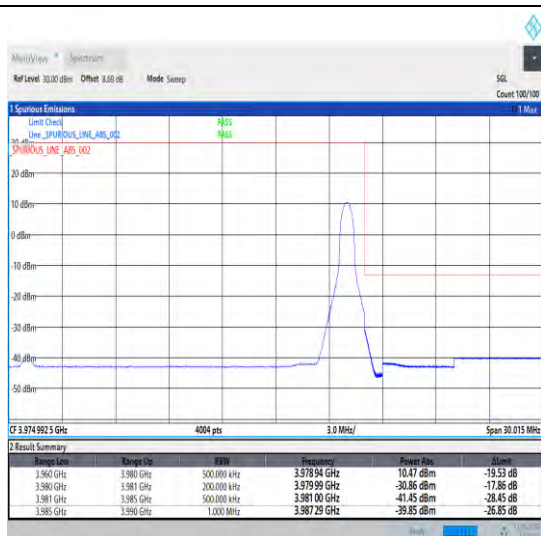
1-N77-3700-3980-30-20-H-2-DFT-PI2BPSK-Edge_1R_B_Right-1@50-Ant1-1--PASS-see graph
