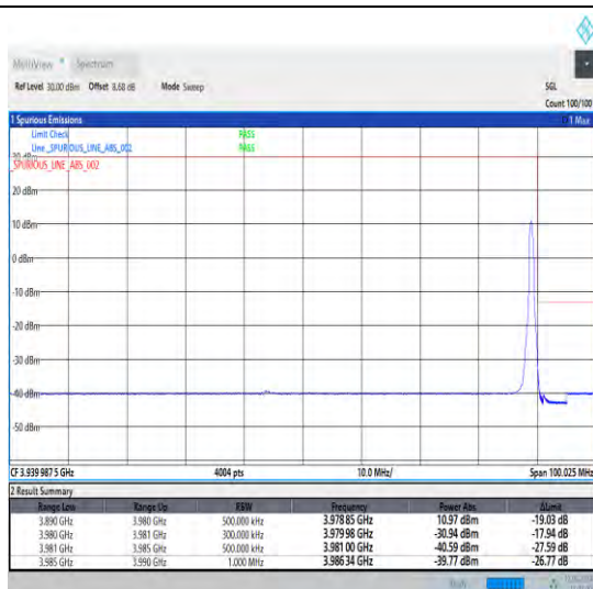
1-N77-3700-3980-30-90-H-2-DFT-PI2BPSK-Edge_1R B_Right-1@244-Ant1-1--PASS-see graph
