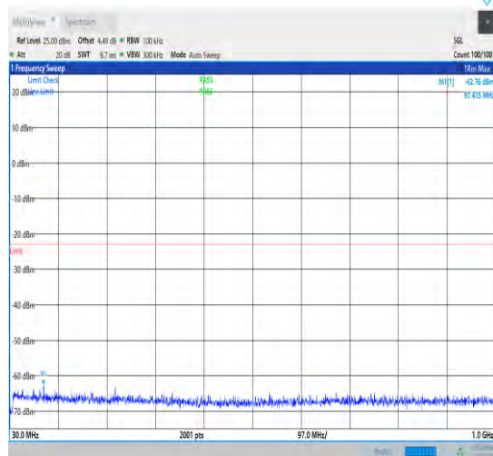
1-N77-3700-3980-30-100-M-1-DFT-QPSK-Edge_1R B_Left-1@0-30-1000-Ant1-97.42--62.76--23-PASS
