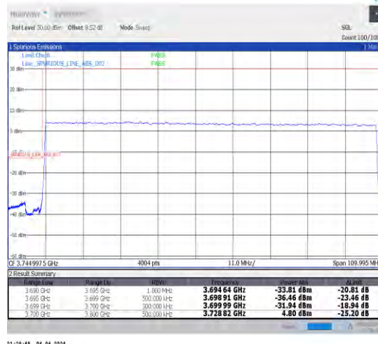
1-N77-3700-3980-30-100-L-3-DFT-PI2BPSK-Outer_Full-270@0-Ant1-1--PASS-see graph
