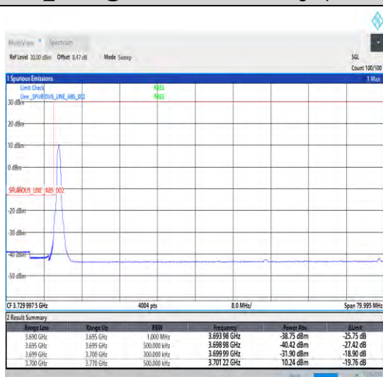
1-N77-3700-3980-30-70-L-4-CP-QPSK-Edge_1RB_Lef t-1@0-Ant1-1--PASS-see graph
