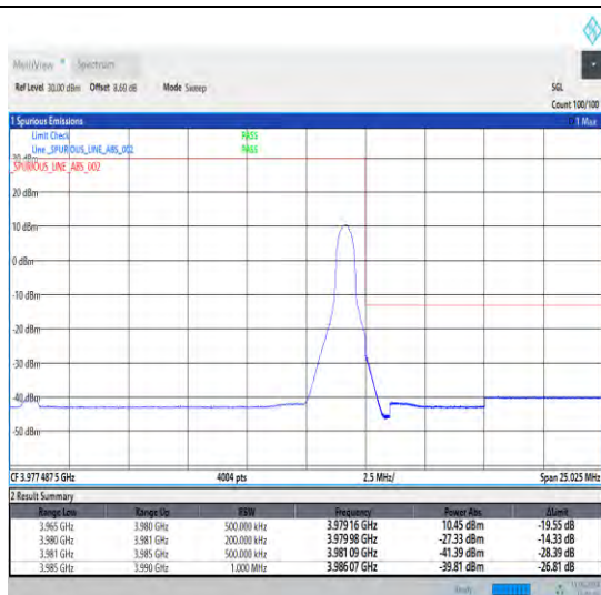
1-N77-3700-3980-30-15-H-2-DFT-PI2BPSK-Edge_1R_B_Right-1@37-Ant1-1--PASS-see graph
