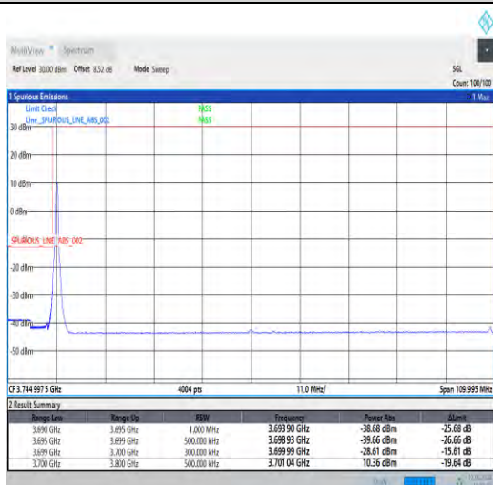
1-N77-3700-3980-30-100-L-4-CP-QPSK-Edge_1RB_Left-1@0-Ant1-1--PASS-see graph
