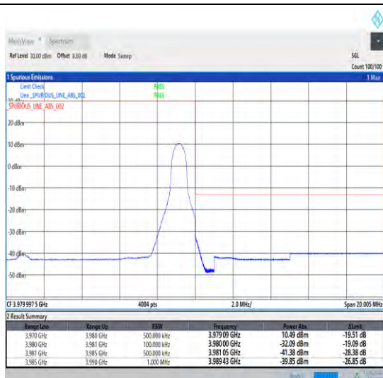
1-N77-3700-3980-30-10-H-2-DFT-PI2BPSK-Edge_1R_B_Right-1@23-Ant1-1--PASS-see graph
