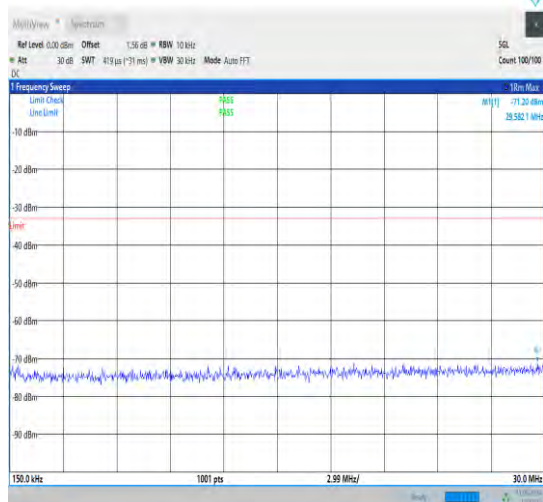
1-N77-3700-3980-30-100-M-1-DFT-QPSK-Edge_1R B_Left-1@0-0.15-30-Ant1-29.58--71.20--33-PASS
