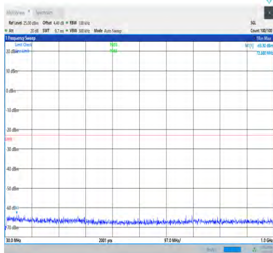
1-N77-3700-3980-30-100-L-1-DFT-QPSK-Edge_1R B_Left-1@0-30-1000-Ant1-72.68--63.30--23-PASS
