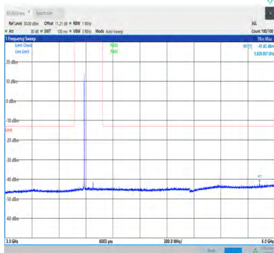
1-N77-3700-3980-30-100-H-1-DFT-QPSK-Edge_1R B_Left-1@0-3000-6000-Ant1-5829.06--41.92--13-PA SS
