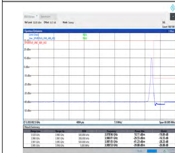
1-N77-3700-3980-30-60-H-5-CP-QPSK-Edge_1RB_Ri ght-1@161-Ant1-1--PASS-see graph
