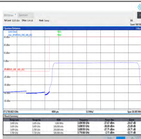
1-N77-3700-3980-30-20-L-6-CP-QPSK-Outer_Full -51@0-Ant1-1--PASS-see graph
