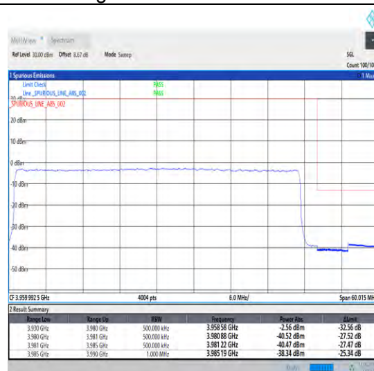
1-N77-3700-3980-30-50-H-3-DFT-PI2BPSK-Outer _Full-128@0-Ant1-1--PASS-see graph
