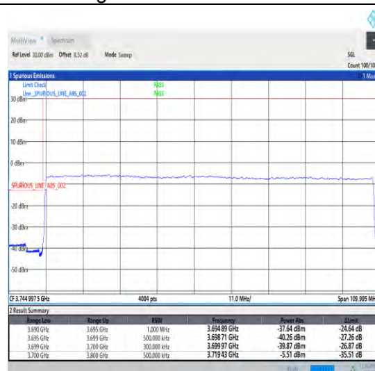
1-N77-3700-3980-30-100-L-3-DFT-PI2BPSK-Outer_Full-270@0-Ant1-1--PASS-see graph
