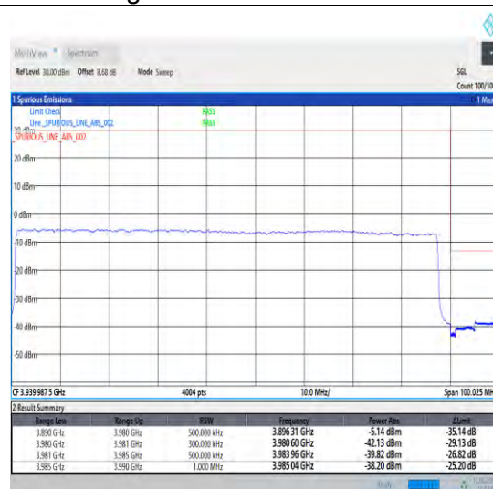
1-N77-3700-3980-30-90-H-3-DFT-PI2BPSK-Outer _Full-240@0-Ant1-1--PASS-see graph
