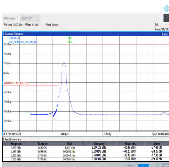
1-N77-3700-3980-30-20-L-1-DFT-PI2BPSK-Edge_1RB _Left-1@0-Ant1-1--PASS-see graph
