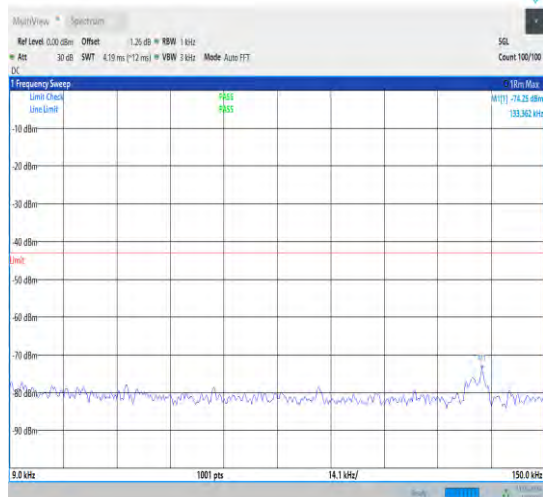
1-N77-3700-3980-30-100-L-1-DFT-QPSK-Edge_1R B_Left-1@0-0.009-0.15-Ant1-0.13--74.25--43-PASS
