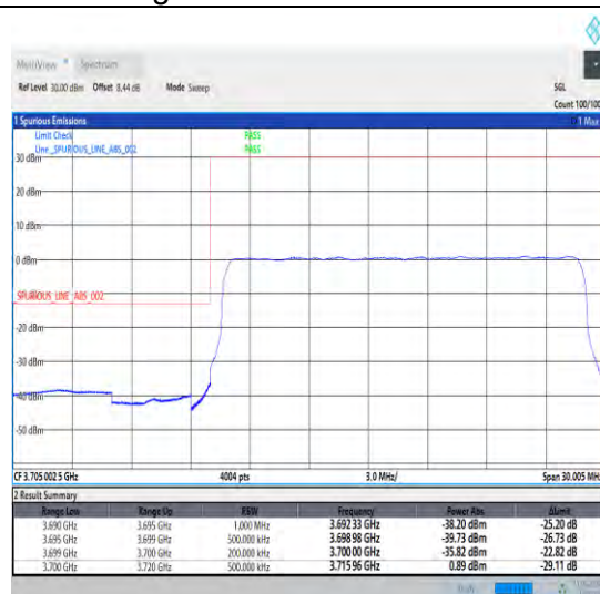
1-N77-3700-3980-30-20-L-3-DFT-PI2BPSK-Outer _Full-50@0-Ant1-1--PASS-see graph
