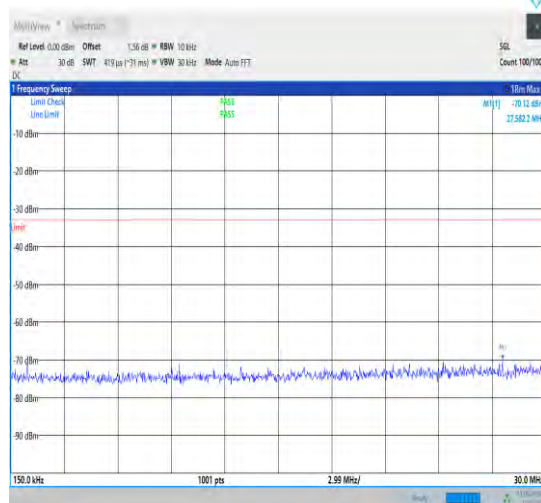
1-N77-3700-3980-30-100-H-1-DFT-QPSK-Edge_1R B_Left-1@0-0.15-30-Ant1-27.58--70.12--33-PASS
