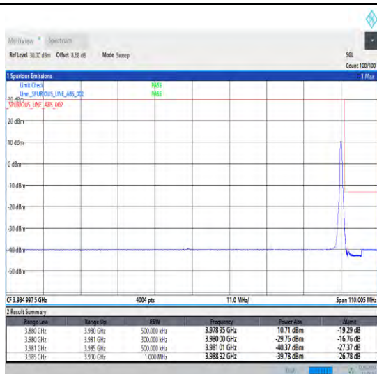
1-N77-3700-3980-30-100-H-2-DFT-PI2BPSK-Edge_1R_B_Right-1@272-Ant1-1--PASS-see graph
