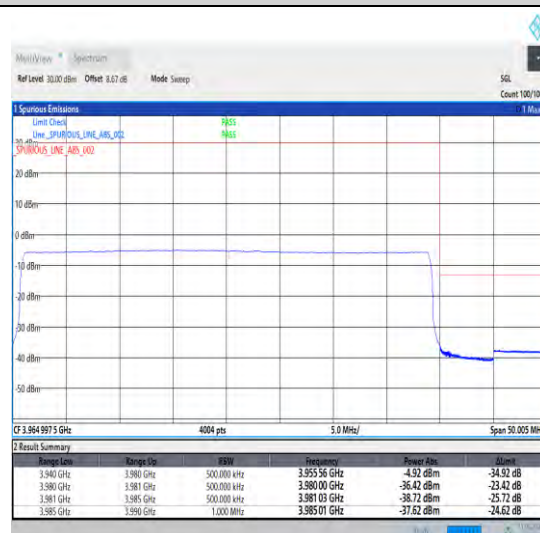
1-N77-3700-3980-30-40-H-6-CP-QPSK-Outer_Full -106@0-Ant1-1--PASS-see graph
