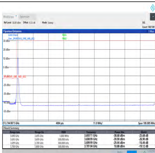
1-N77-3700-3980-30-100-L-1-DFT-PI2BPSK-Edge_1R_B_Left-1@0-Ant1-1--PASS-see graph
