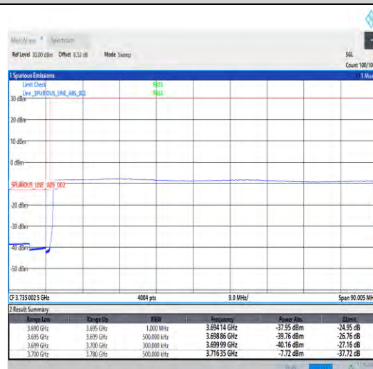
1-N77-3700-3980-30-80-L-6-CP-QPSK-Outer_Full -217@0-Ant1-1--PASS-see graph
