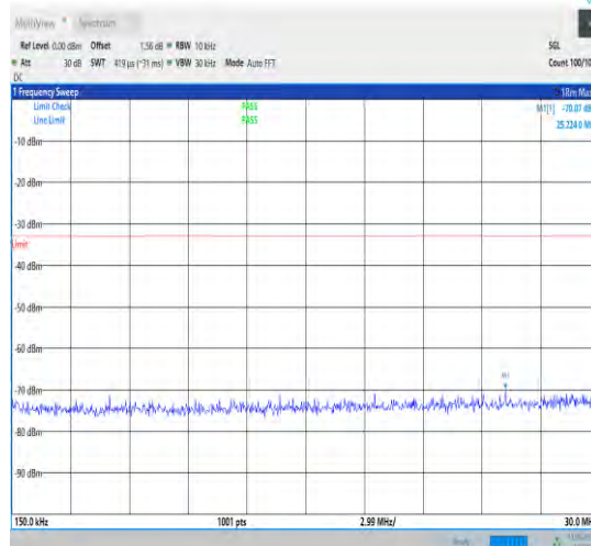
1-N77-3700-3980-30-100-L-1-DFT-QPSK-Edge_1RB _Left-1@0-0.15-30-Ant1-25.22--70.07--33-PASS
