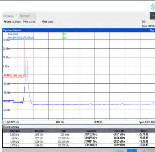
1-N77-3700-3980-30-60-L-4-CP-QPSK-Edge_1RB_Lef t-1@0-Ant1-1--PASS-see graph
