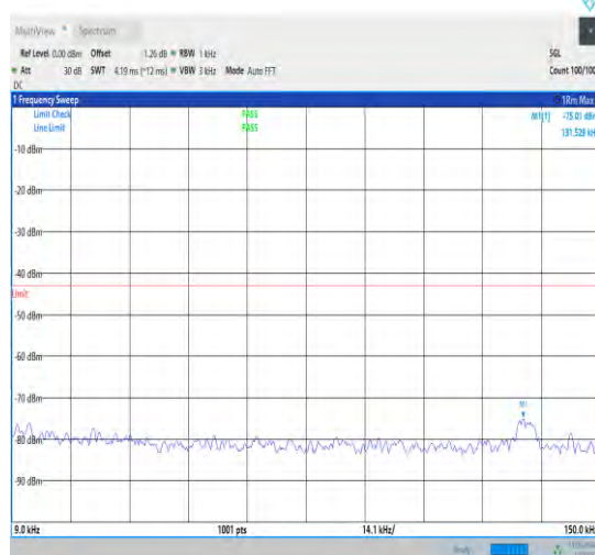
1-N77-3700-3980-30-100-M-1-DFT-QPSK-Edge_1R B_Left-1@0-0.009-0.15-Ant1-0.13--75.01--43-PASS
