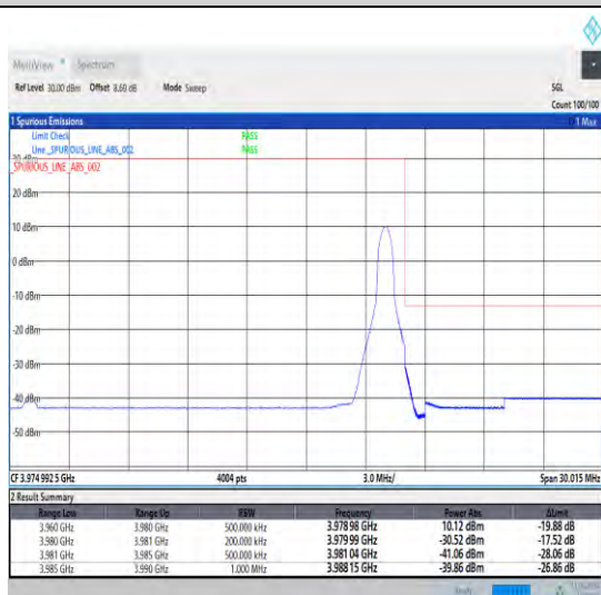
1-N77-3700-3980-30-20-H-5-CP-QPSK-Edge_1RB_Right-1@50-Ant1-1--PASS-see graph
