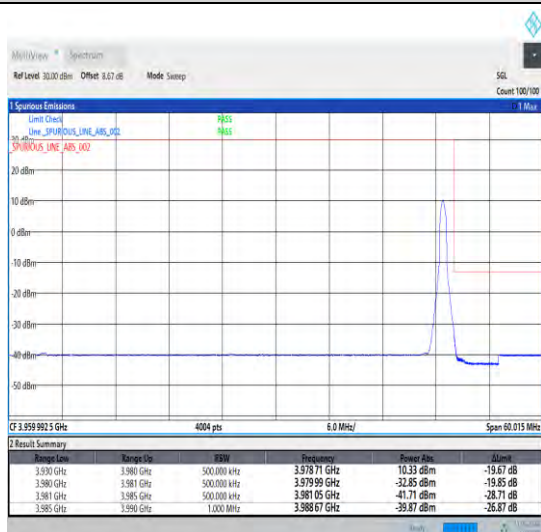
1-N77-3700-3980-30-50-H-5-CP-QPSK-Edge_1RB_Ri ght-1@132-Ant1-1--PASS-see graph
