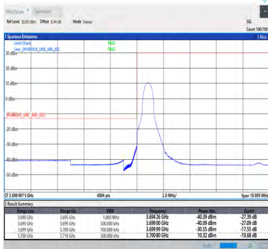
1-N77-3700-3980-30-10-L-4-CP-QPSK-Edge_1RB_Lef t-1@0-Ant1-1--PASS-see graph
