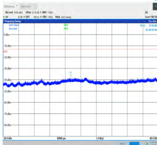
1-N77-3700-3980-30-100-M-1-DFT-QPSK-Edge_1R B_Left-1@0-26000-40000-Ant1-32105.14--37.03--13- -PASS
