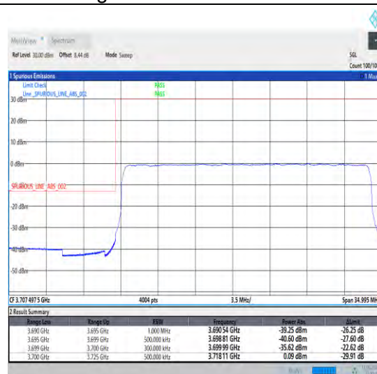
1-N77-3700-3980-30-25-L-3-DFT-PI2BPSK-Outer_Full-64@0-Ant1-1--PASS-see graph
