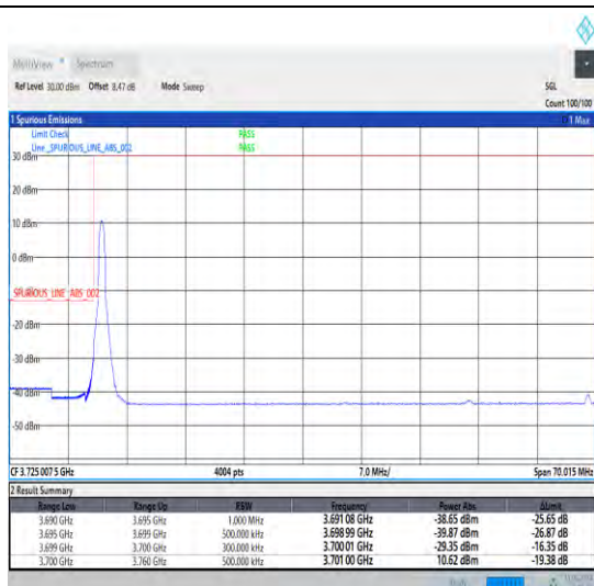
1-N77-3700-3980-30-60-L-1-DFT-PI2BPSK-Edge_1RB _Left-1@0-Ant1-1--PASS-see graph
