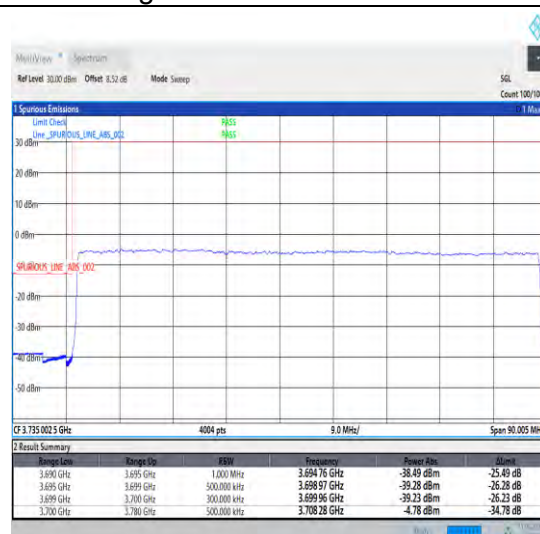
1-N77-3700-3980-30-80-L-3-DFT-PI2BPSK-Outer _Full-216@0-Ant1-1--PASS-see graph
