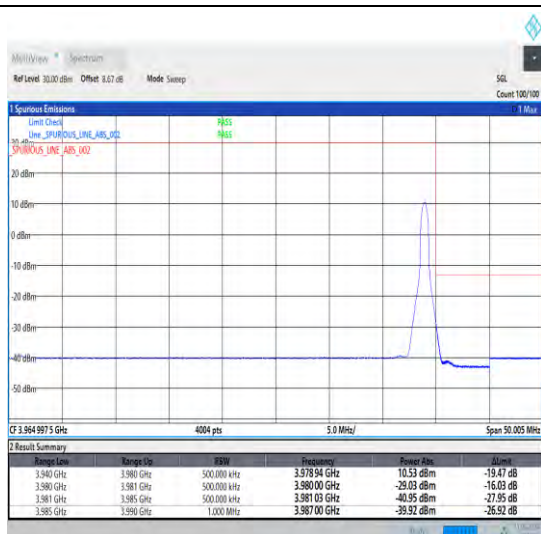
1-N77-3700-3980-30-40-H-2-DFT-PI2BPSK-Edge_1R B_Right-1@105-Ant1-1--PASS-see graph
