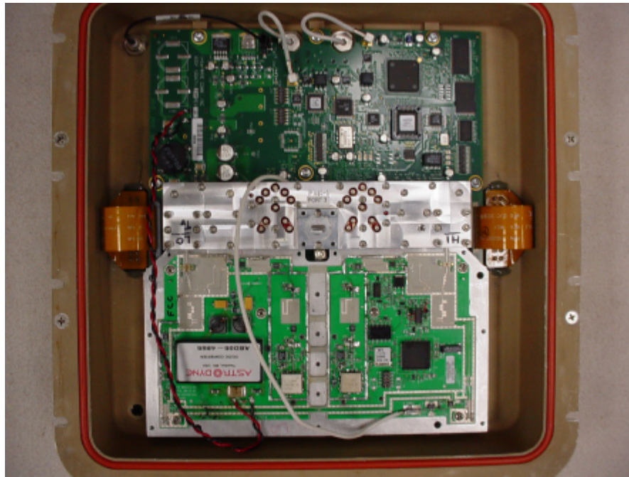
View of 24GHz RF module attached to main PCB in enclosure with shield removed
