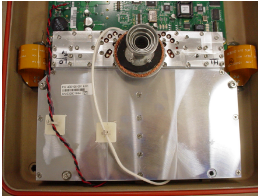
View of 24GHz RF module attached to main PCB with antenna feed and shield in place
